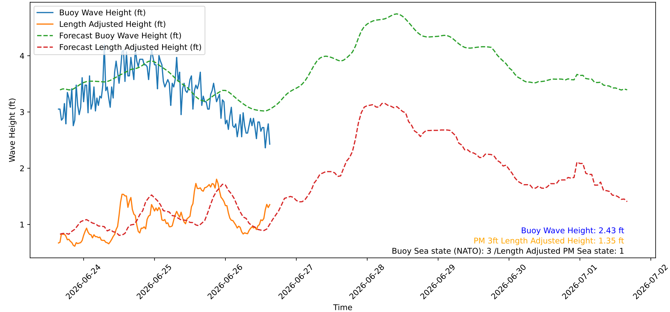
Wave Heights over Time for Green Beach at 2026-06-26 15:41:08
