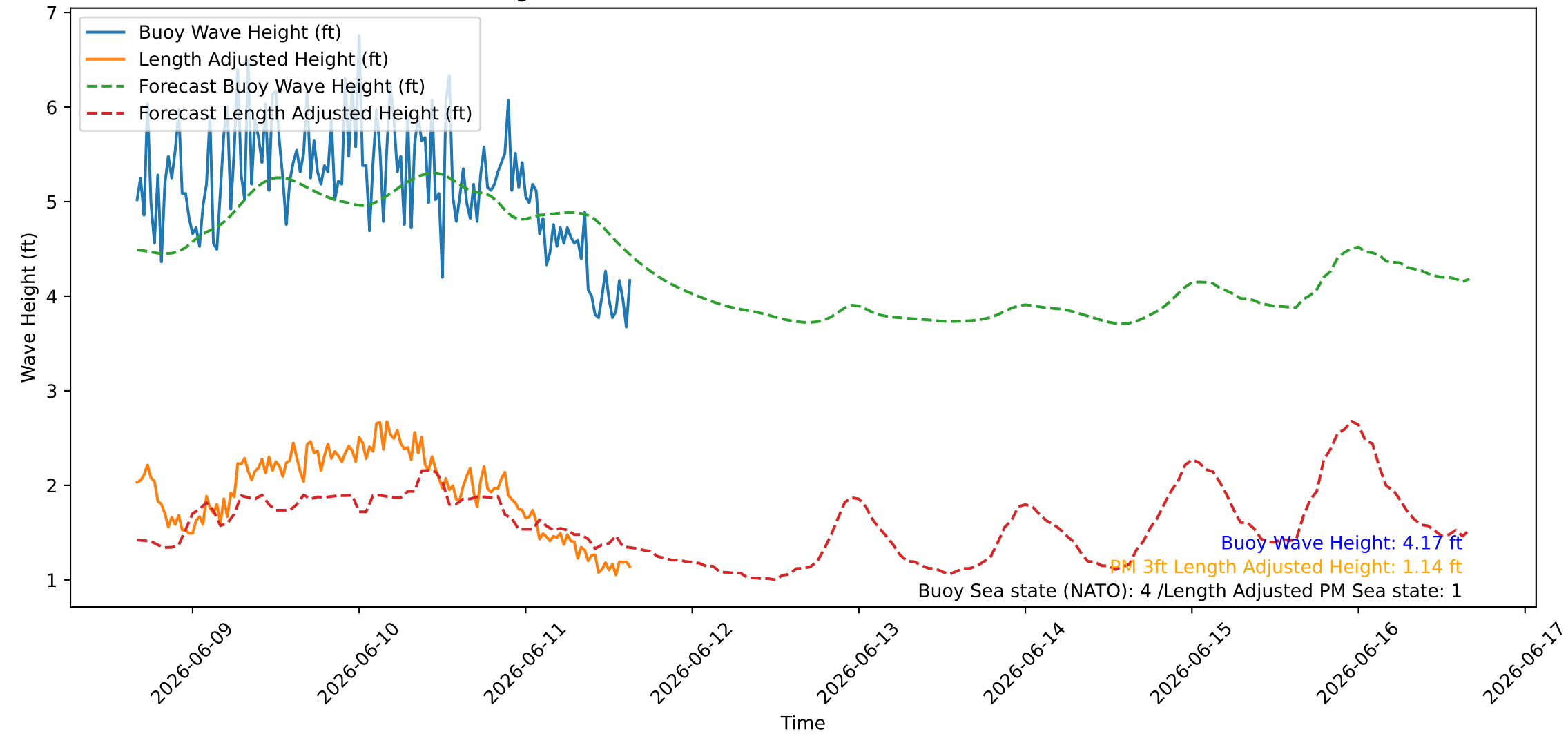
Wave Heights over Time for Oceanside Harbor at 2026-06-11 15:50:26
