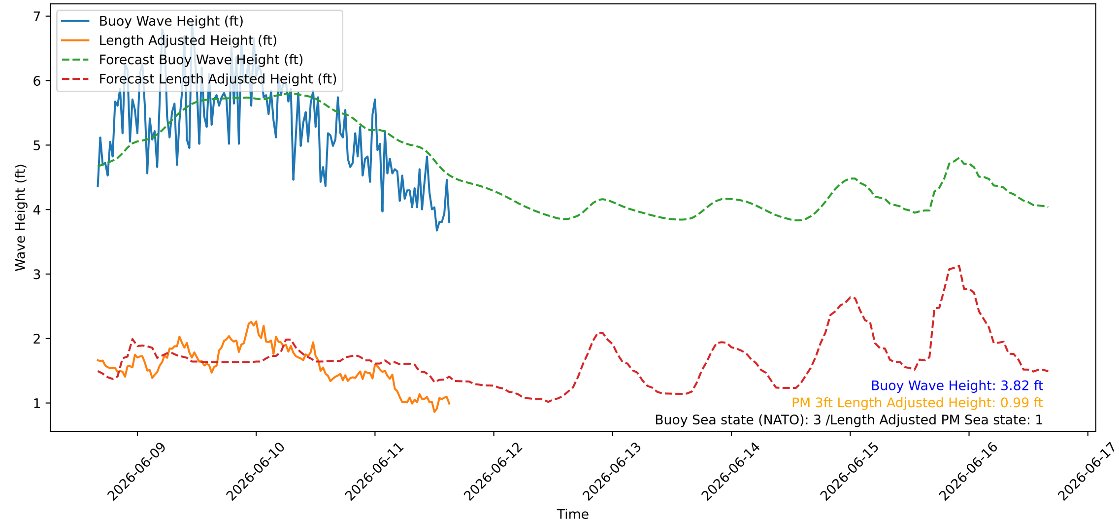
Wave Heights over Time for Green Beach at 2026-06-11 15:51:09
