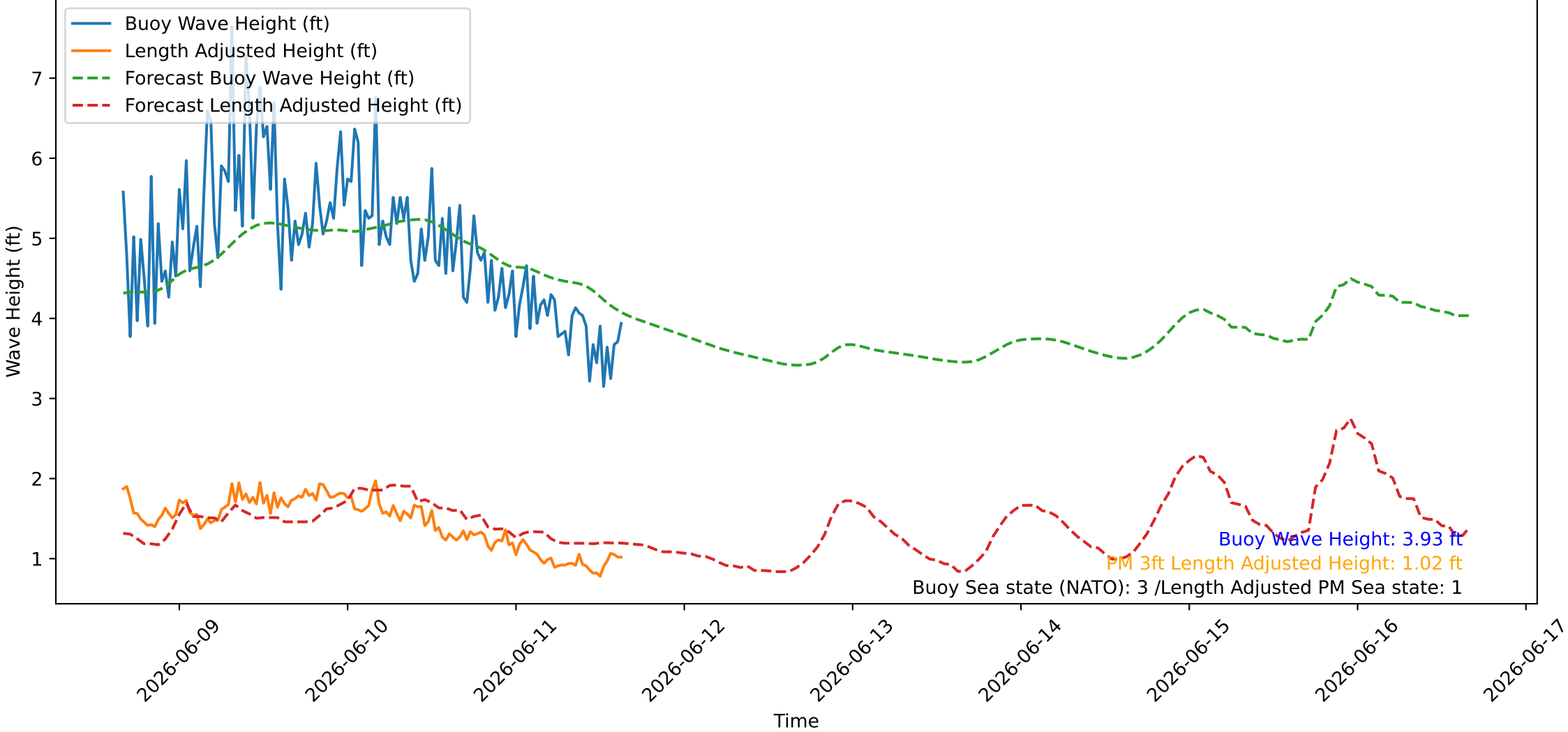
Wave Heights over Time for Red Beach at 2026-06-11 15:50:46
