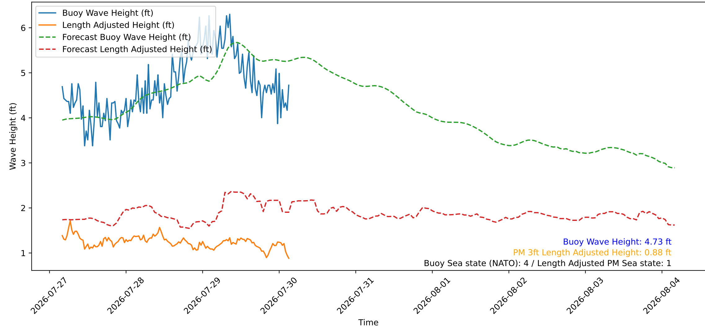
Wave Heights over Time for Green Beach at 2026-07-30 04:01:09
