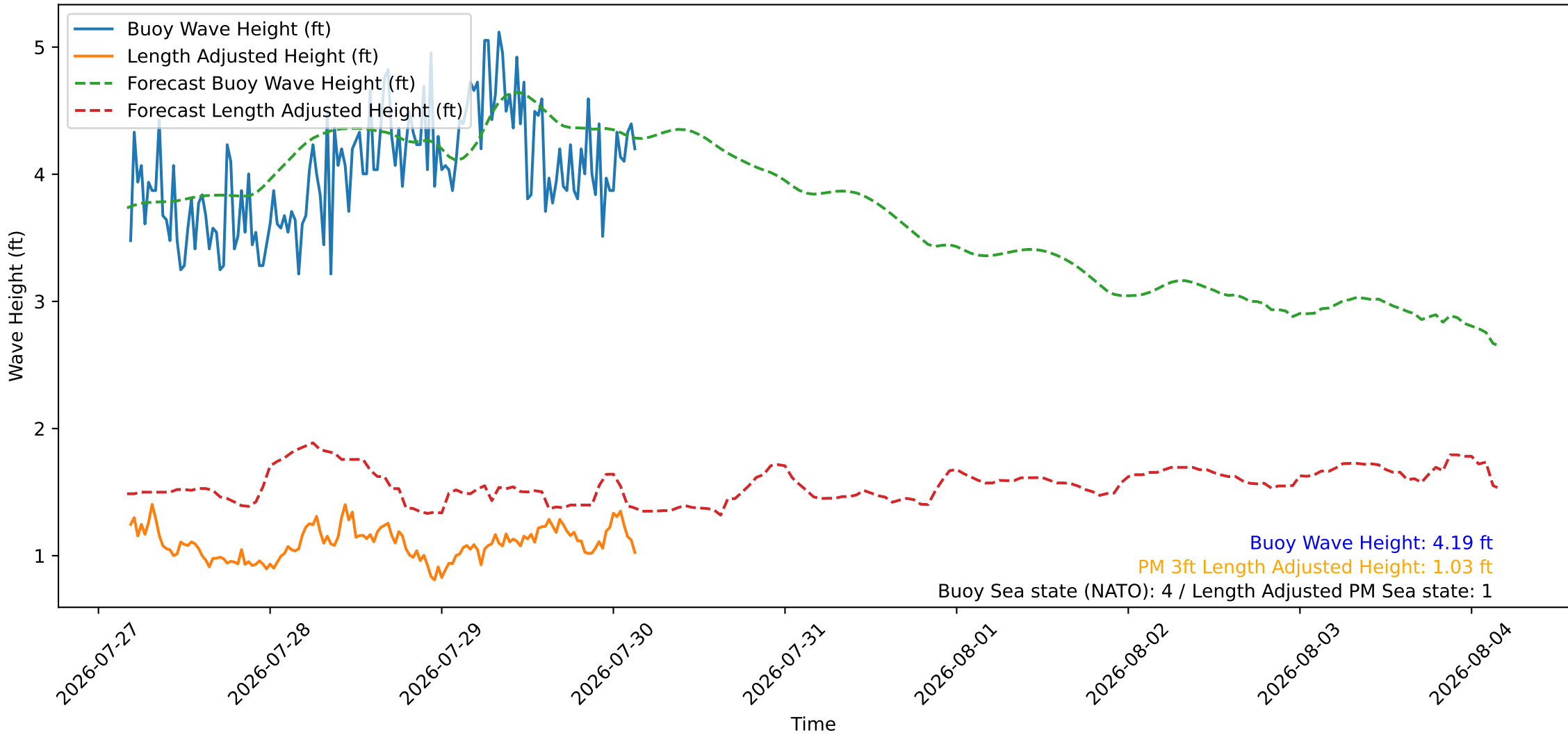
Wave Heights over Time for Red Beach at 2026-07-30 04:00:46
