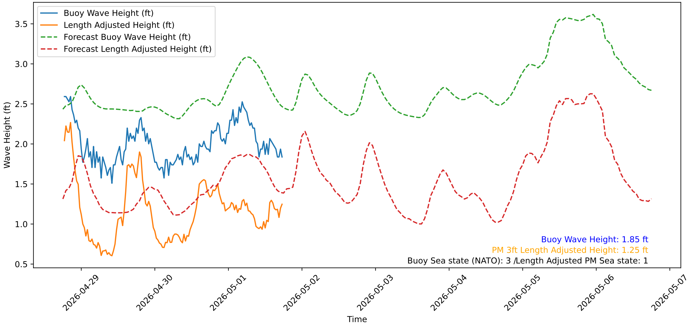
Wave Heights over Time for Red Beach at 2026-05-01 18:10:50
