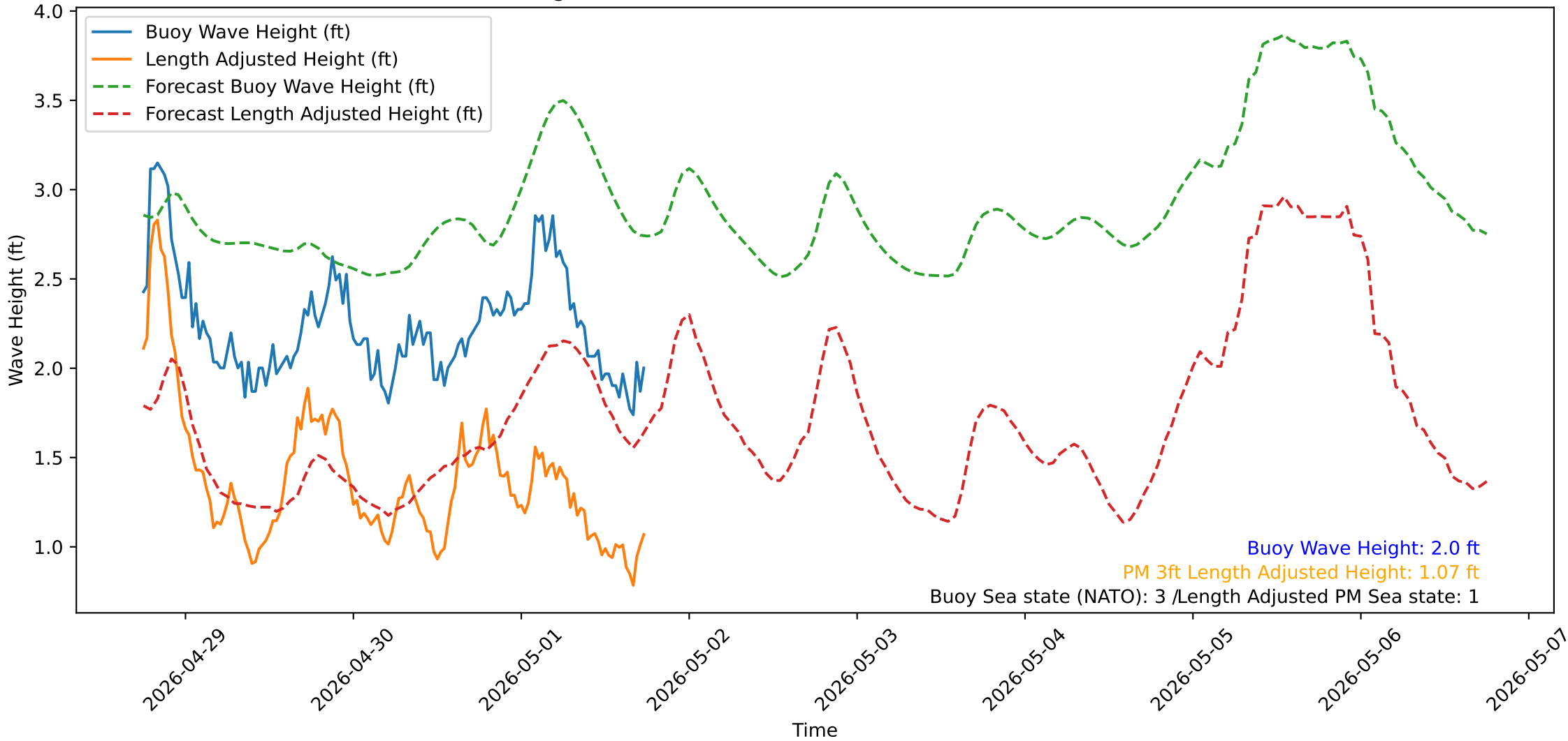
Wave Heights over Time for Green Beach at 2026-05-01 18:11:13
