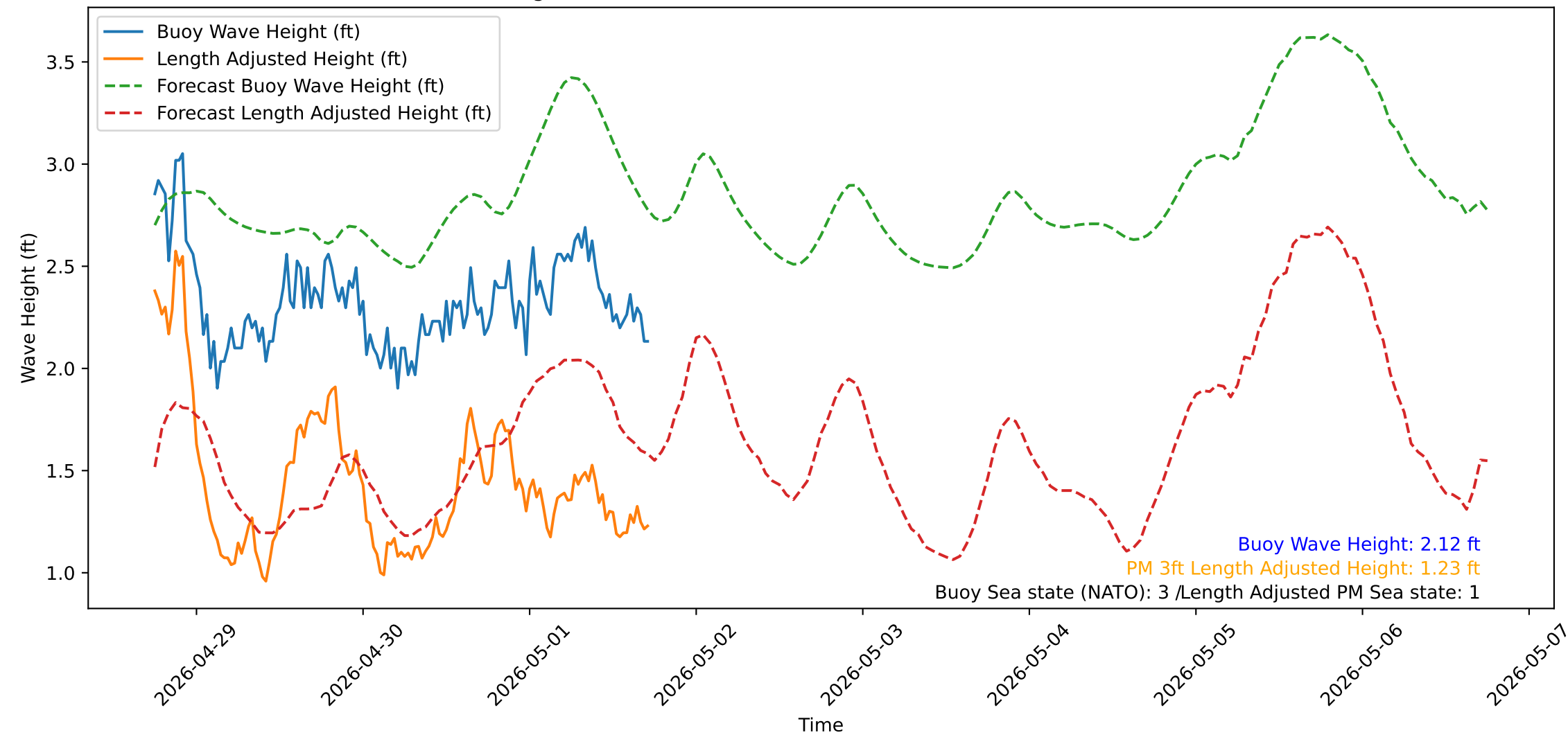
Wave Heights over Time for Oceanside Harbor at 2026-05-01 18:10:31
