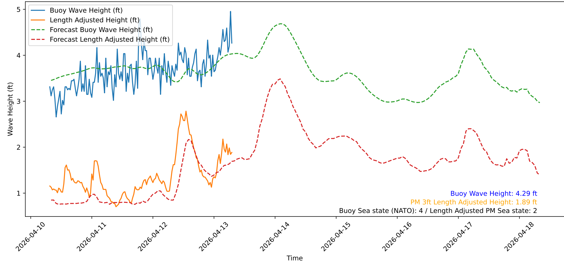
Wave Heights over Time for Oceanside Harbor at 2026-04-13 07:30:31
