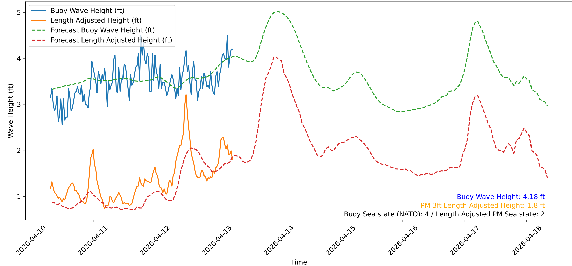
Wave Heights over Time for Green Beach at 2026-04-13 07:31:12
