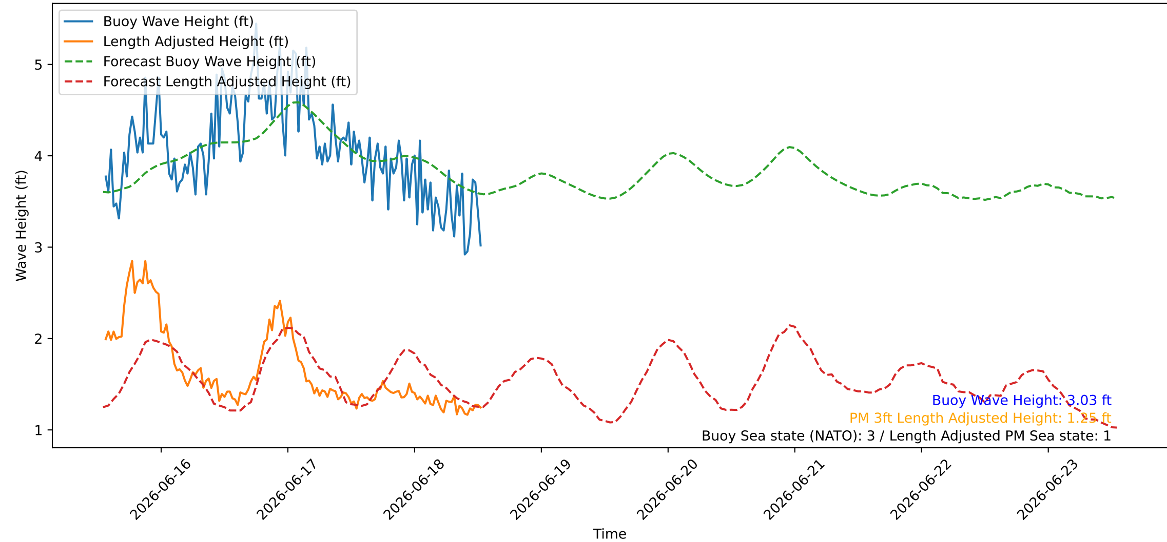
Wave Heights over Time for Oceanside Harbor at 2026-06-18 13:20:26
