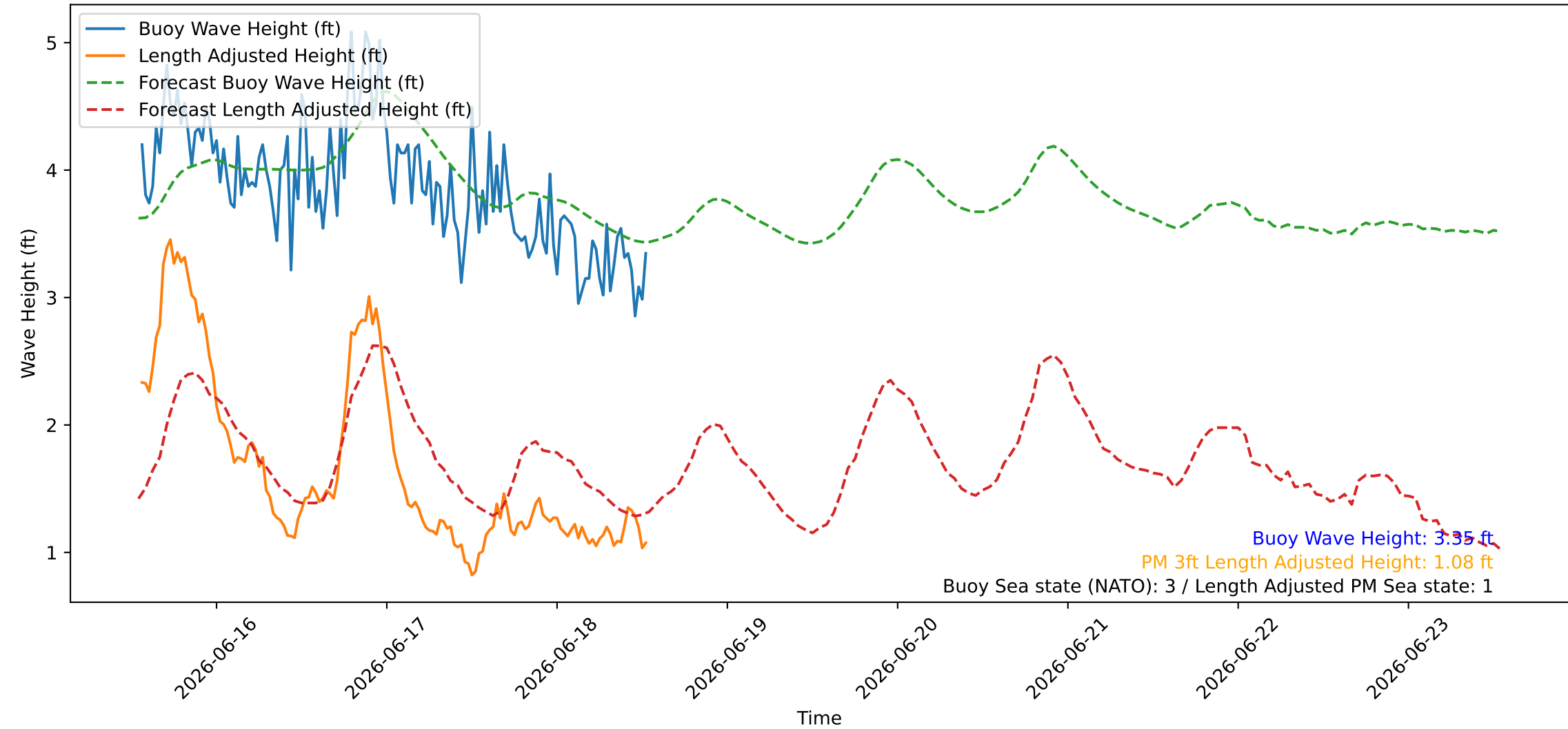
Wave Heights over Time for Green Beach at 2026-06-18 13:21:09
