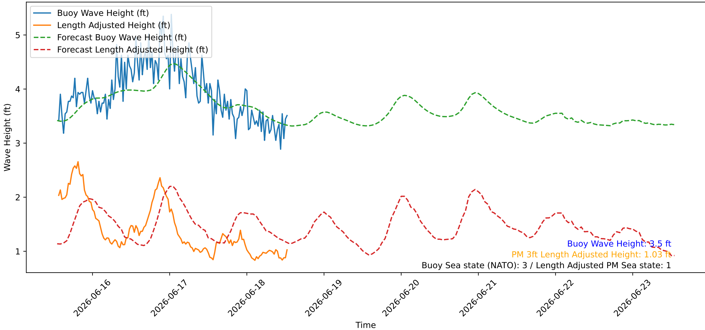
Wave Heights over Time for Red Beach at 2026-06-18 13:20:47
