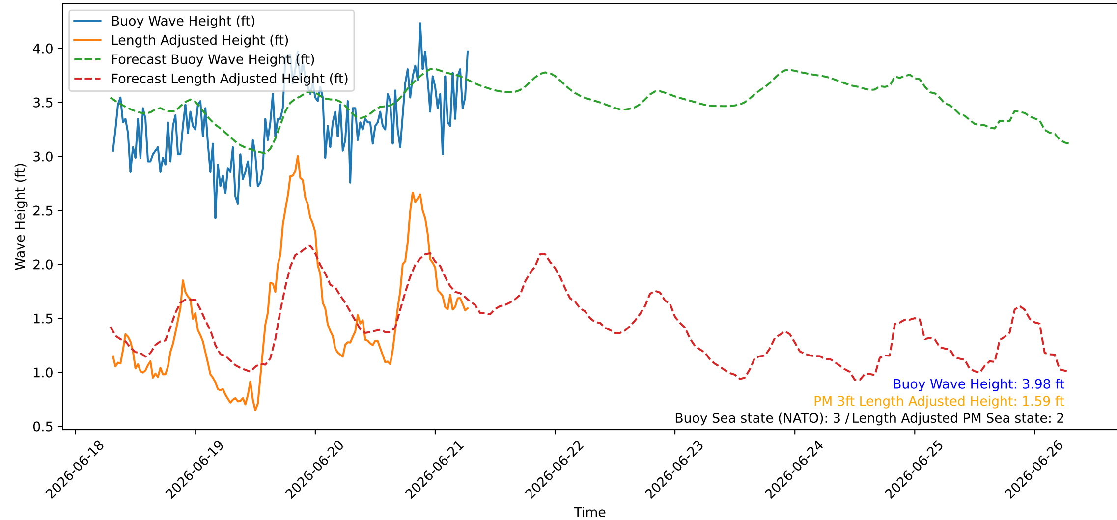
Wave Heights over Time for Green Beach at 2026-06-21 07:21:08
