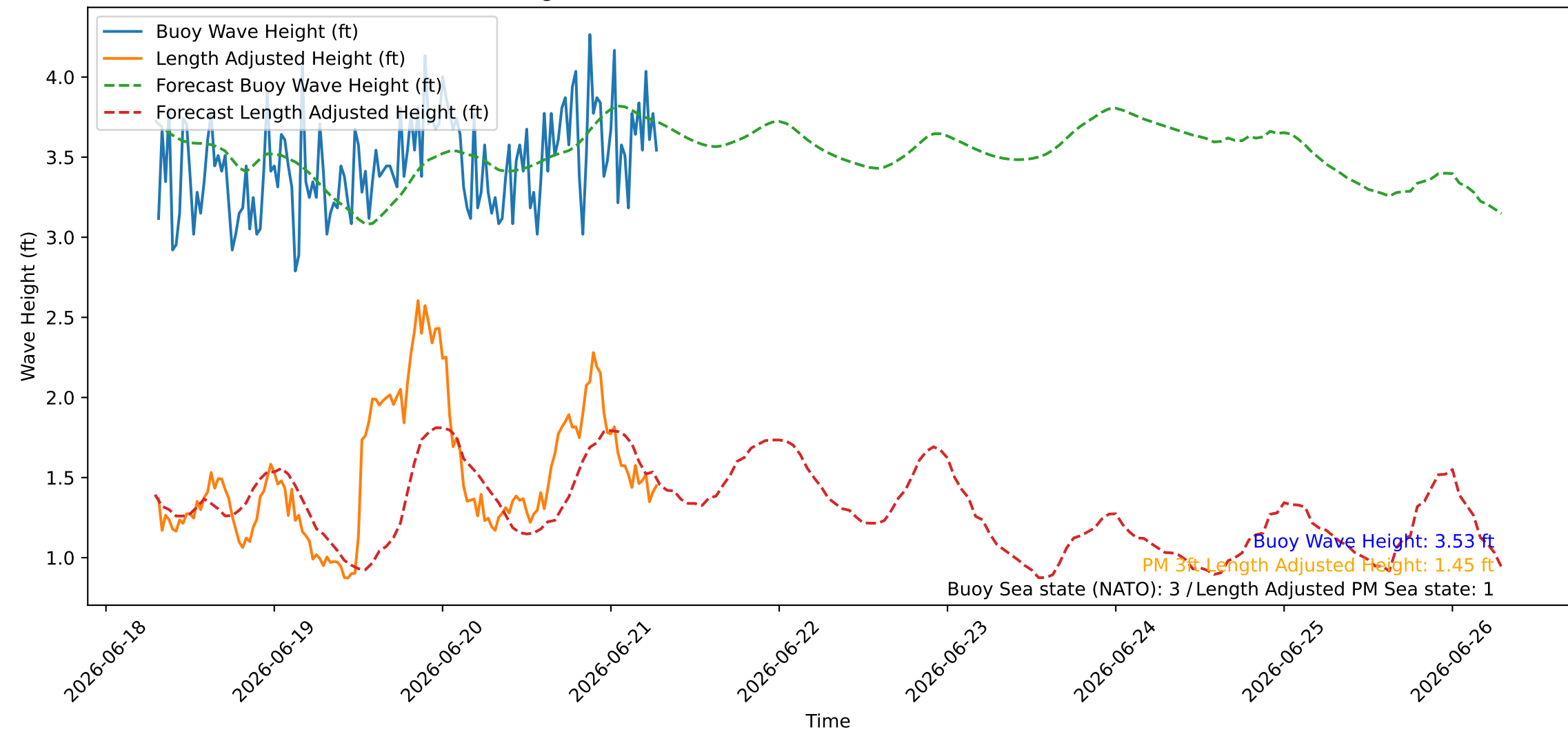
Wave Heights over Time for Oceanside Harbor at 2026-06-21 07:20:26
