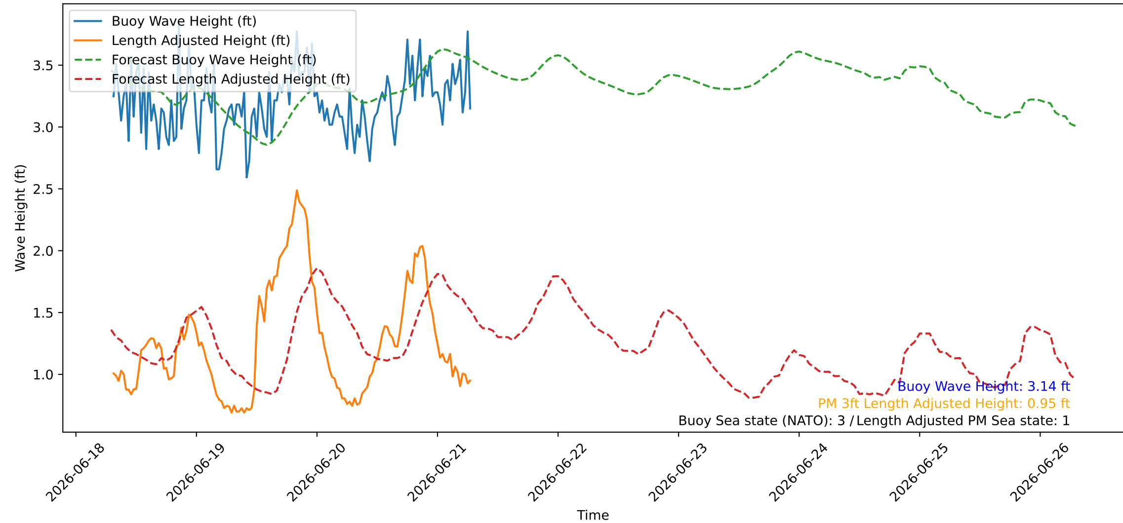
Wave Heights over Time for Red Beach at 2026-06-21 07:20:46
