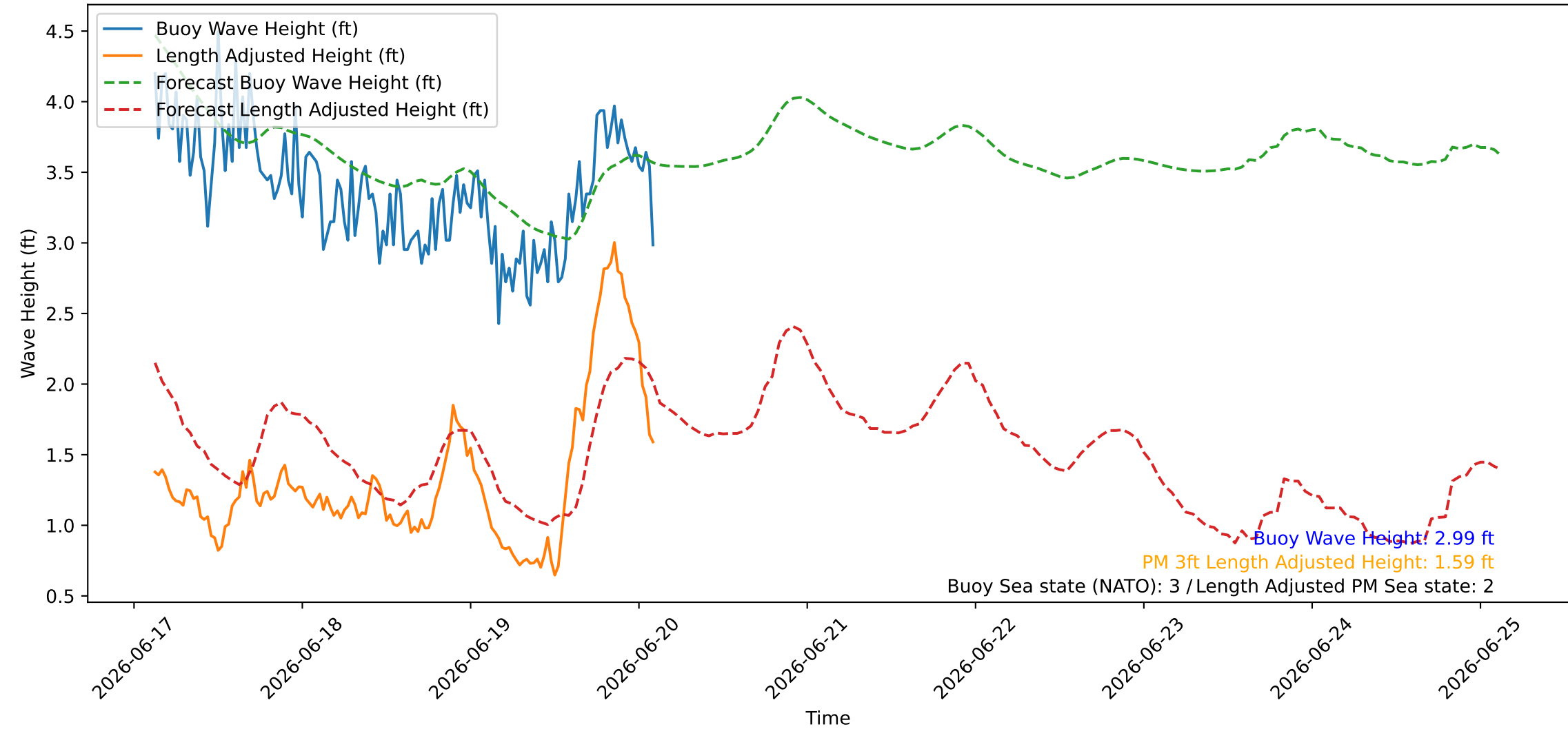
Wave Heights over Time for Green Beach at 2026-06-20 03:01:07
