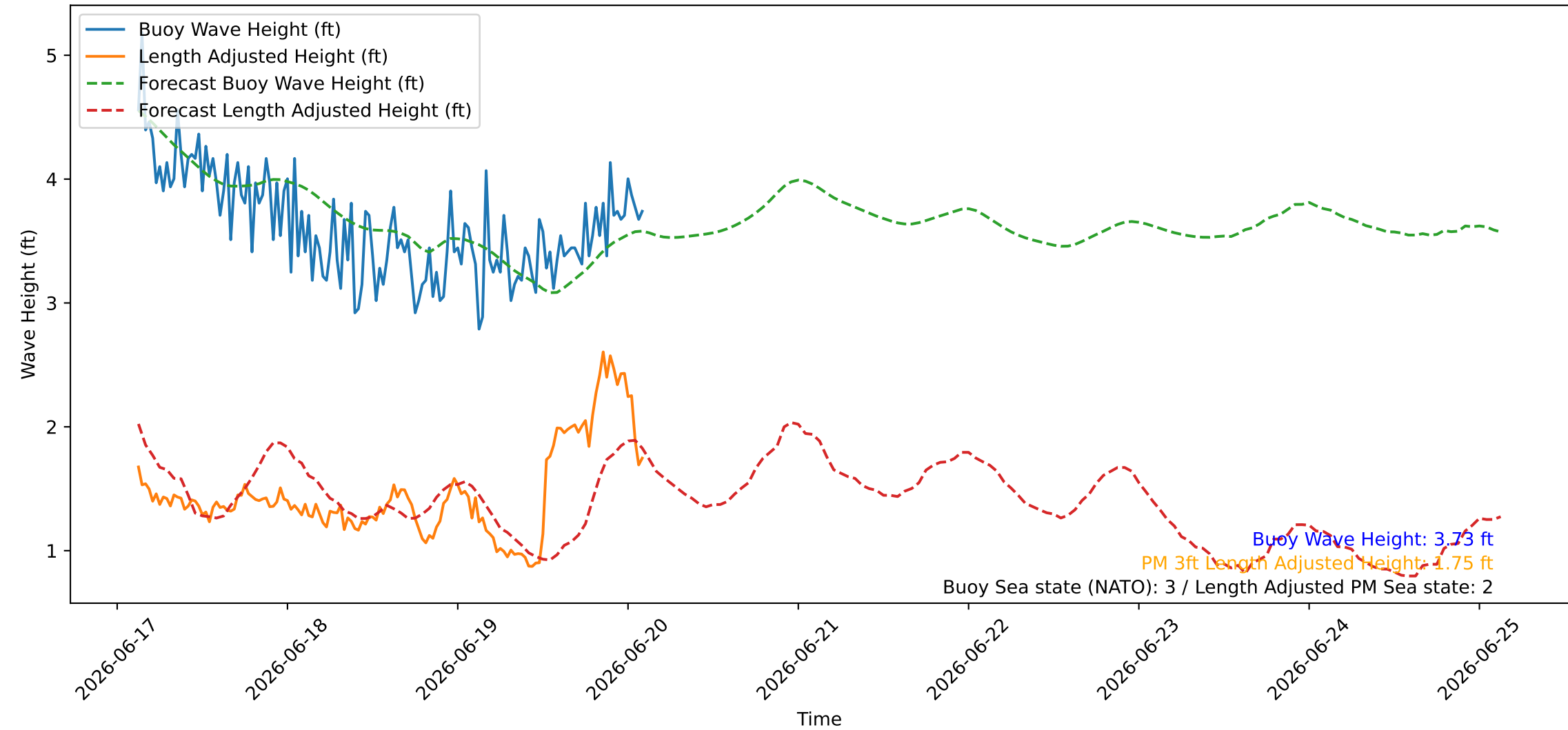
Wave Heights over Time for Oceanside Harbor at 2026-06-20 03:00:26
