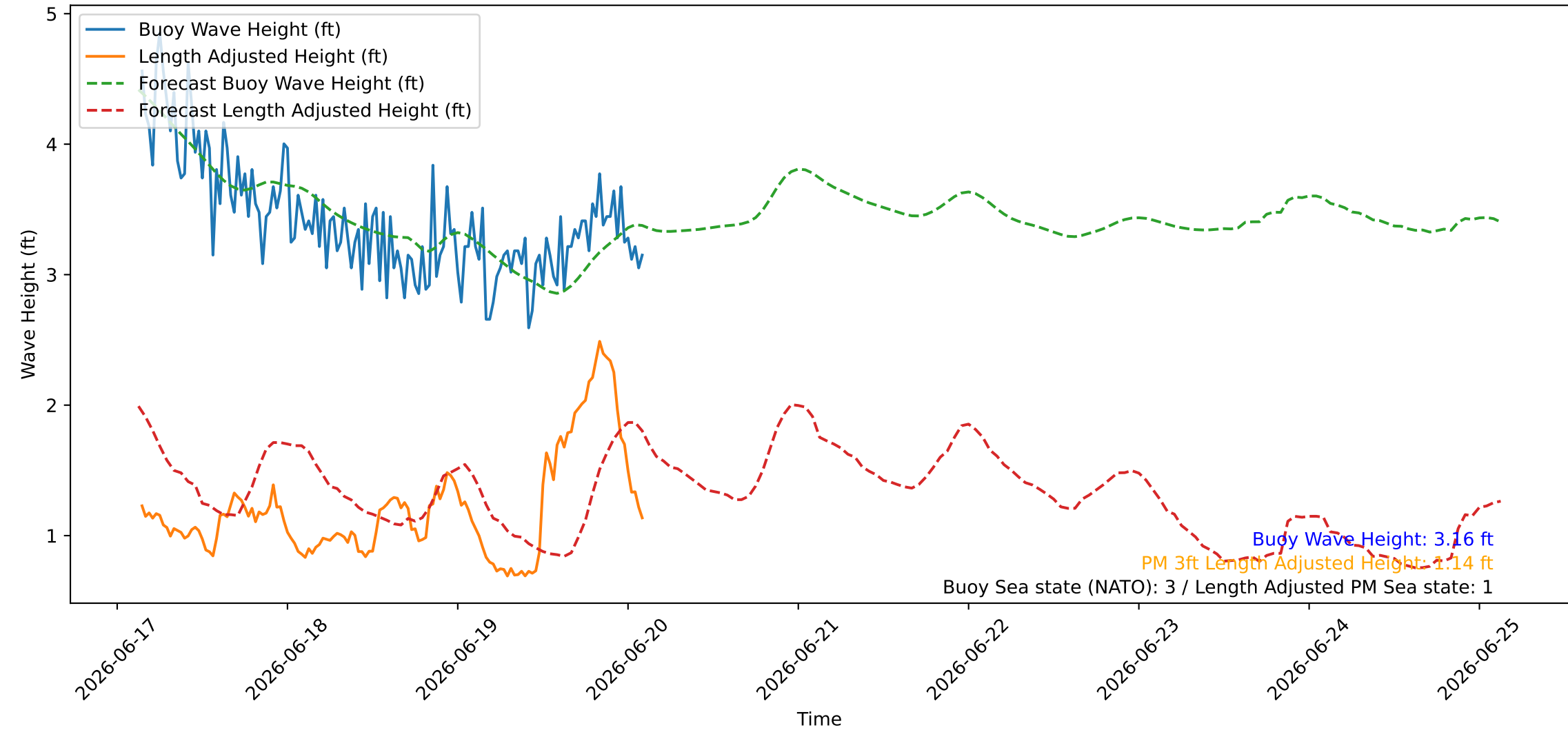
Wave Heights over Time for Red Beach at 2026-06-20 03:00:45
