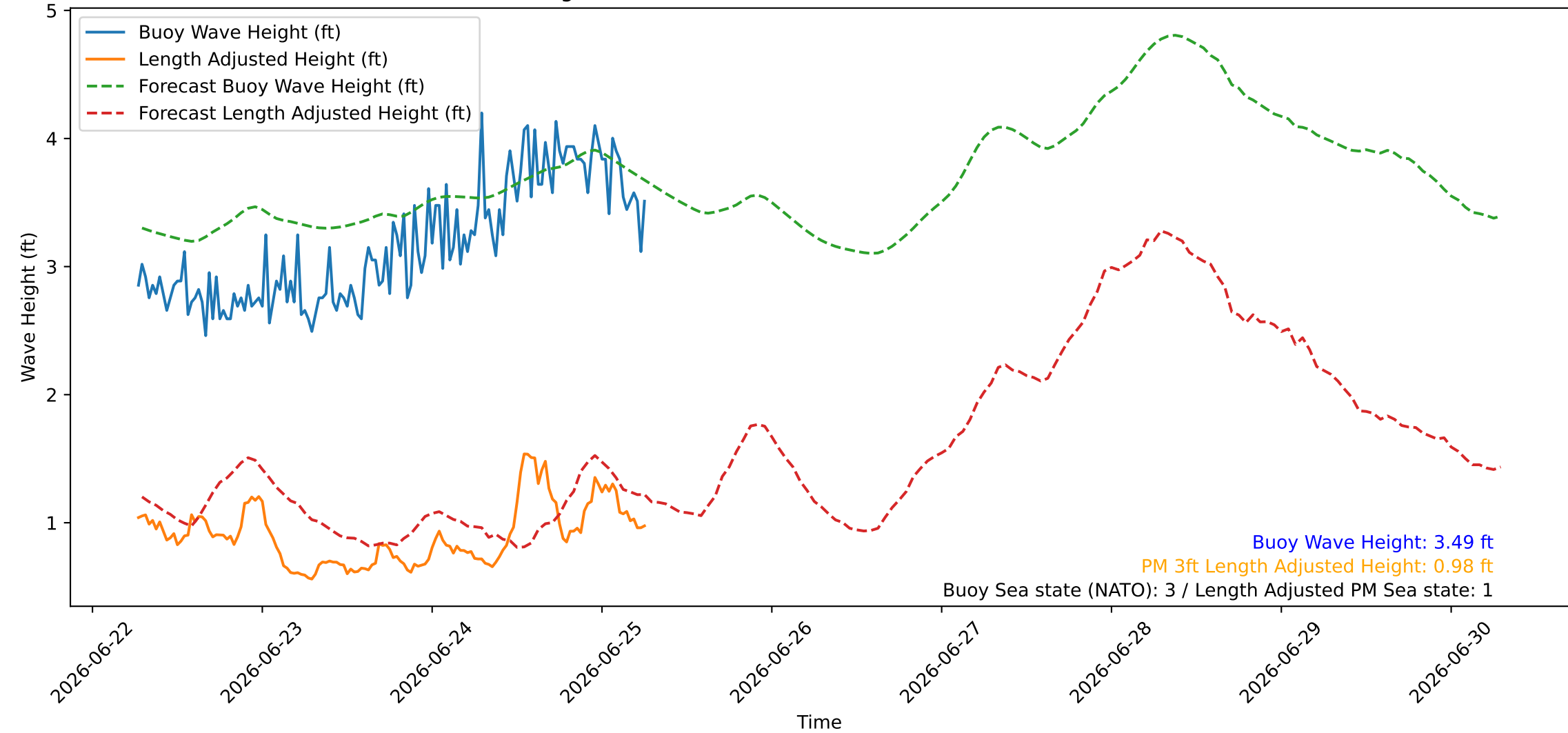
Wave Heights over Time for Green Beach at 2026-06-25 06:41:09
