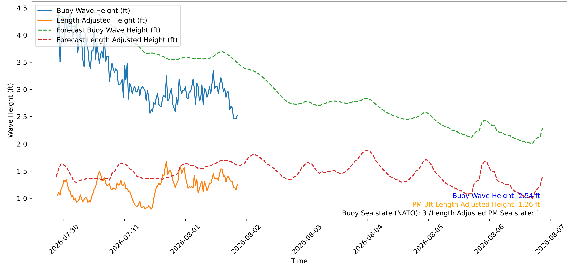
Wave Heights over Time for Red Beach at 2026-08-01 21:10:45
