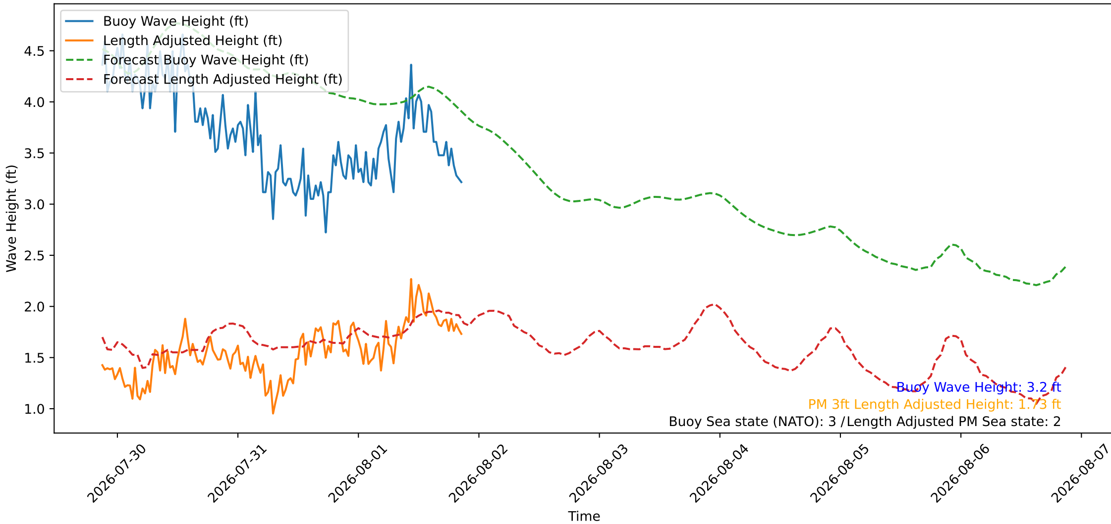
Wave Heights over Time for Oceanside Harbor at 2026-08-01 21:10:26
