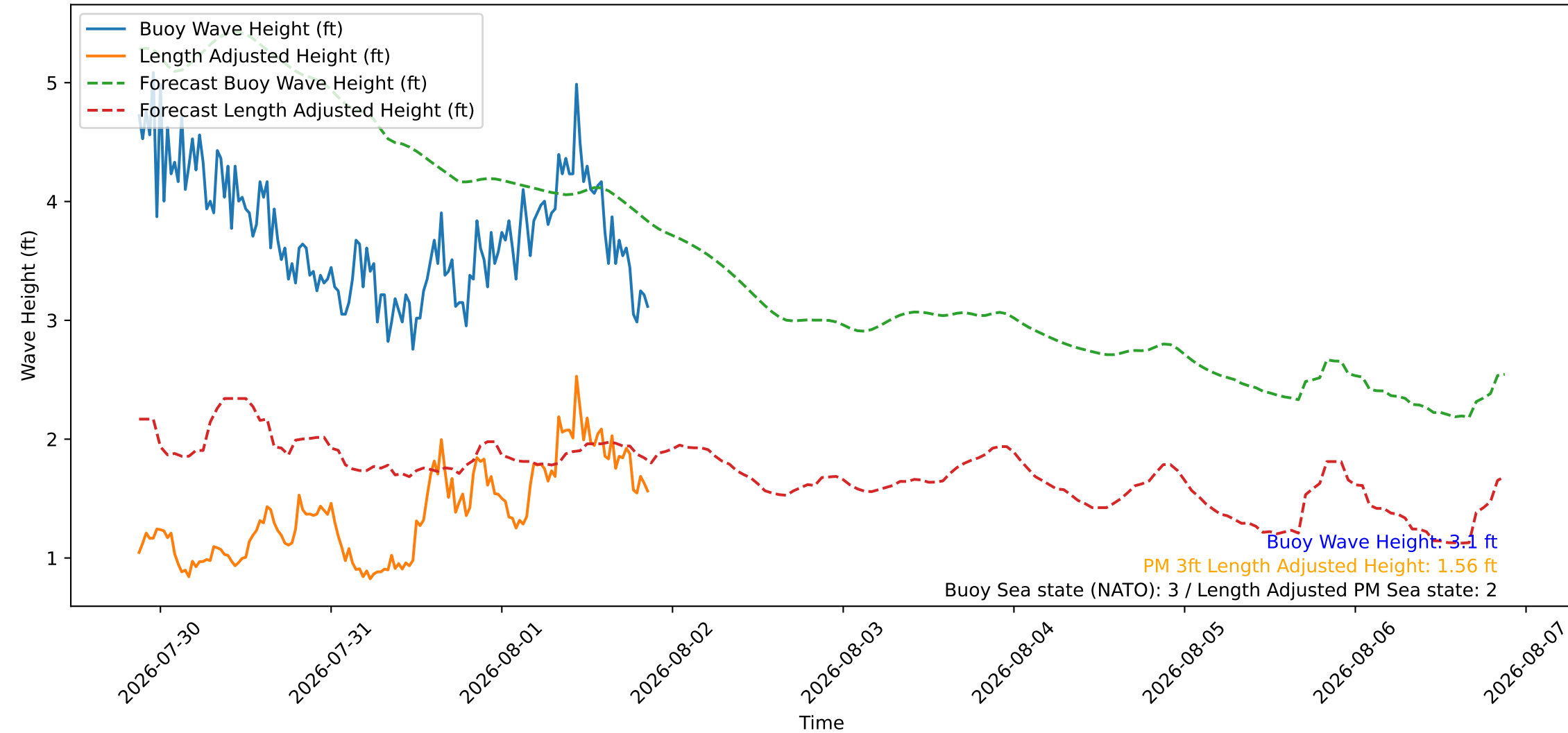
Wave Heights over Time for Green Beach at 2026-08-01 21:11:08
