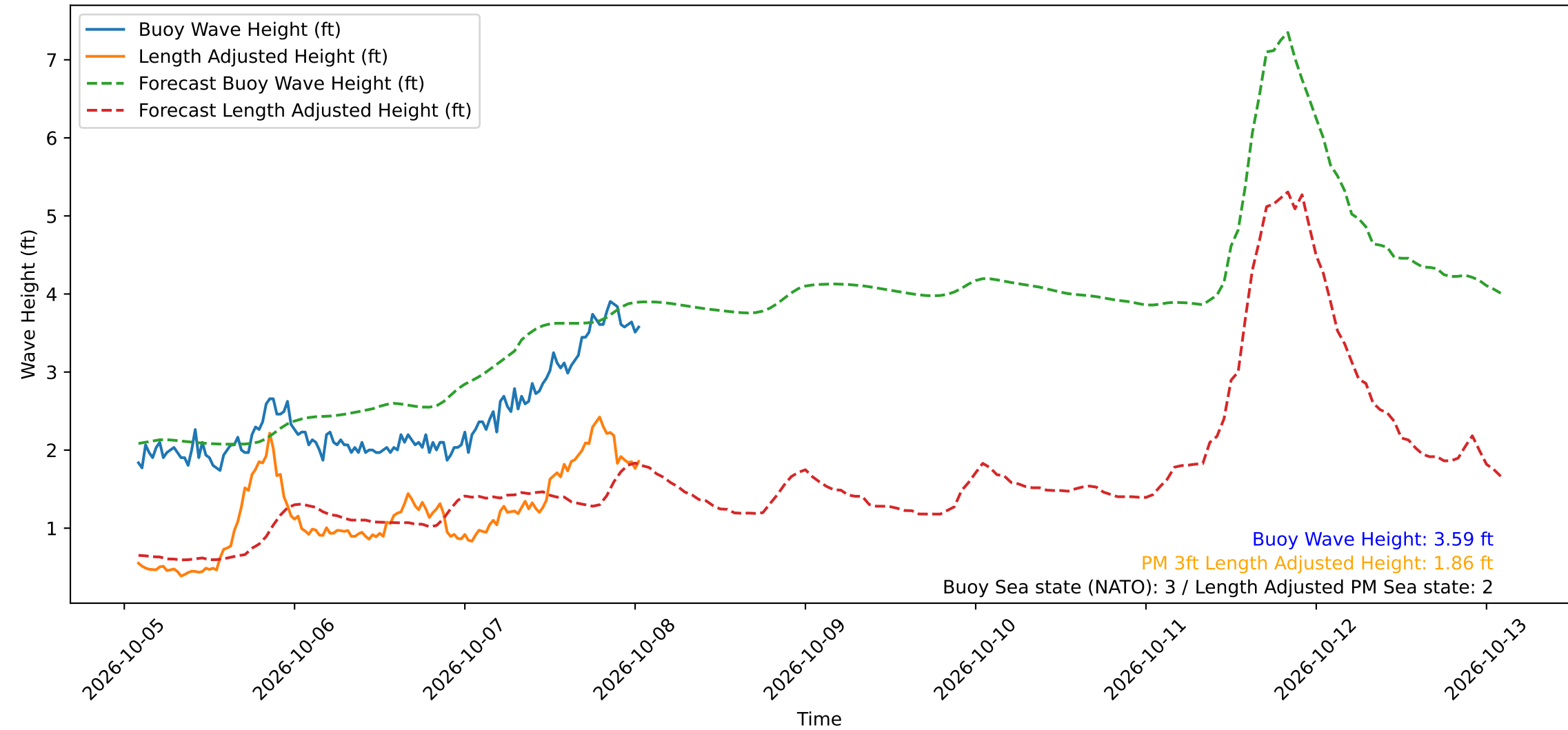
Wave Heights over Time for Red Beach at 2026-10-08 01:30:50
