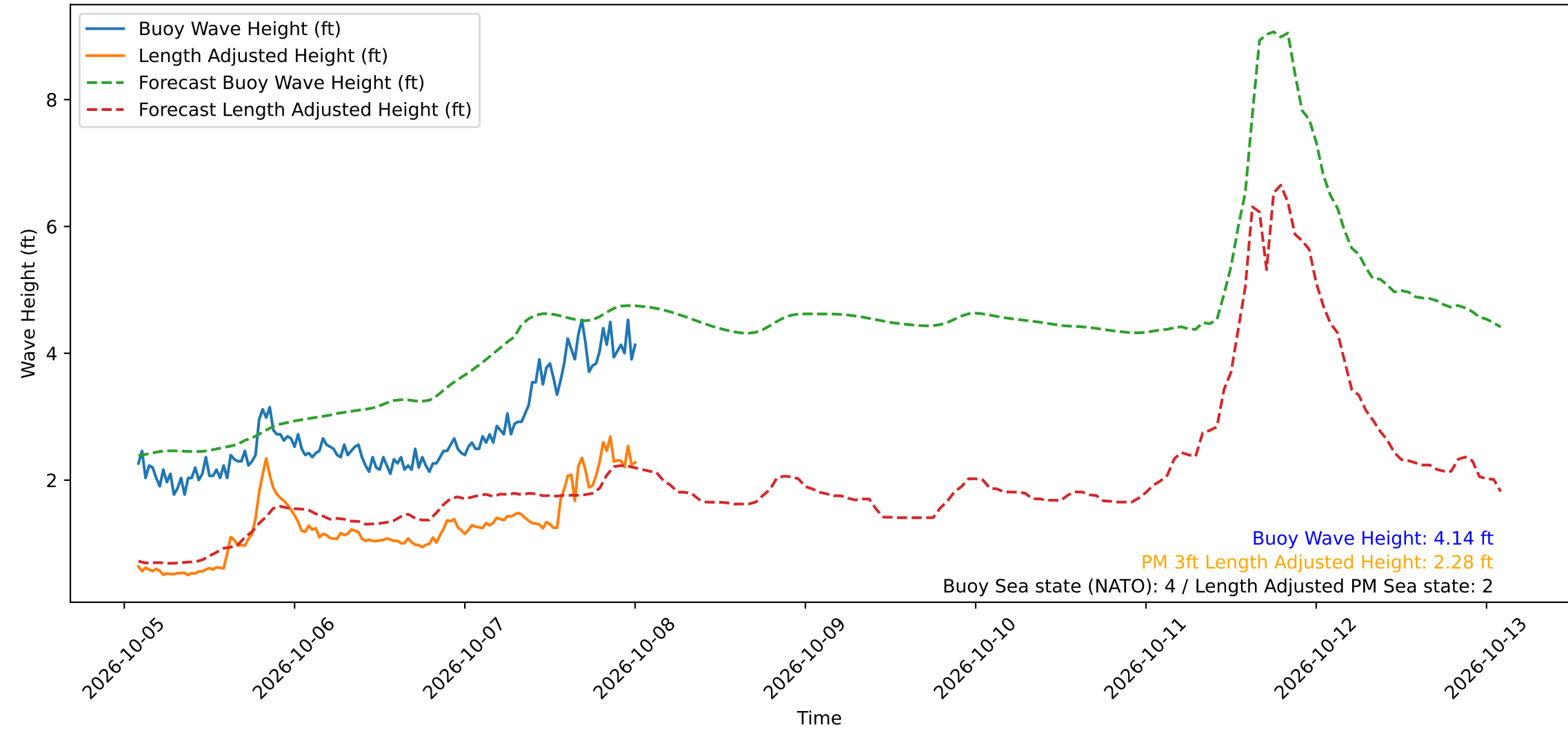
Wave Heights over Time for Green Beach at 2026-10-08 01:31:13
