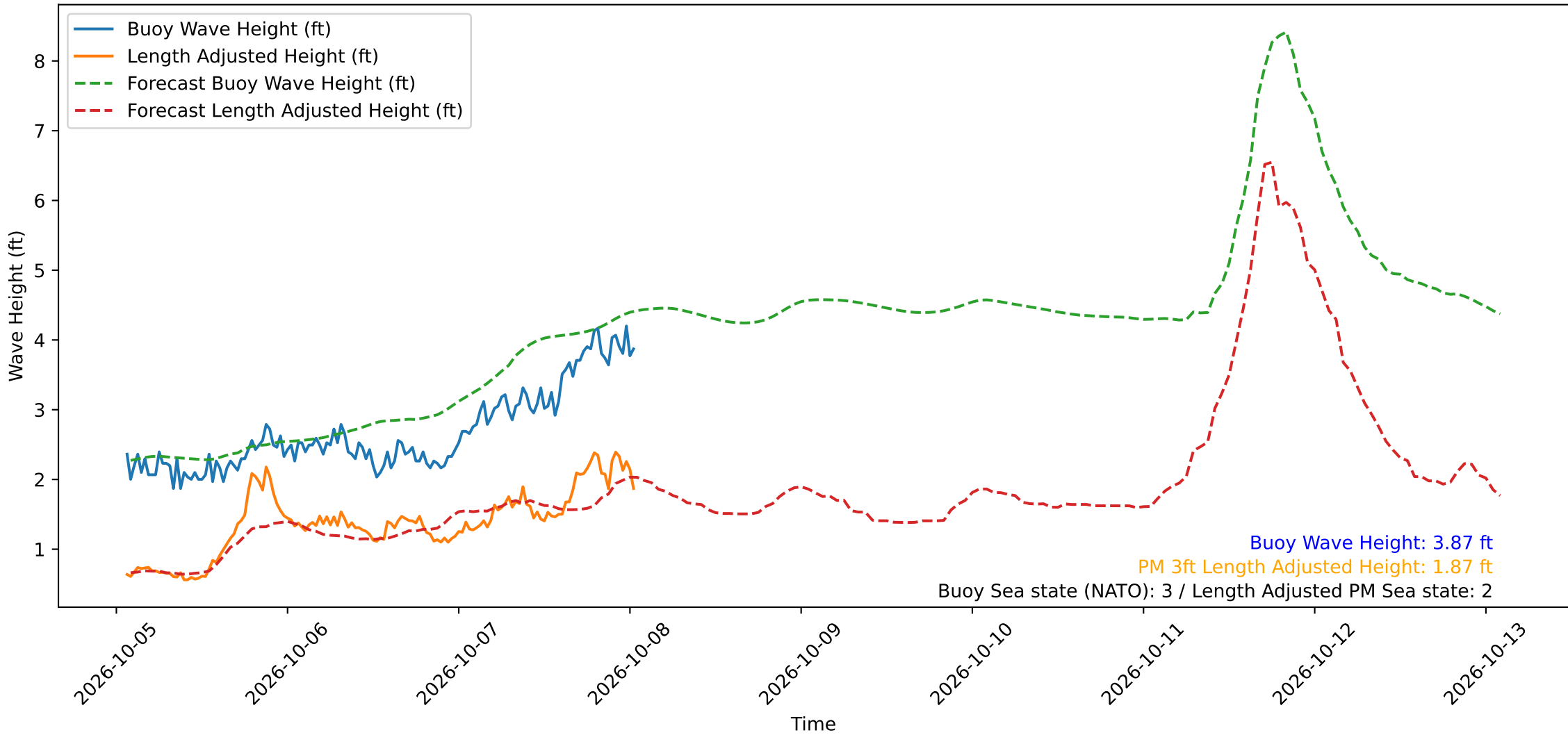
Wave Heights over Time for Oceanside Harbor at 2026-10-08 01:30:30
