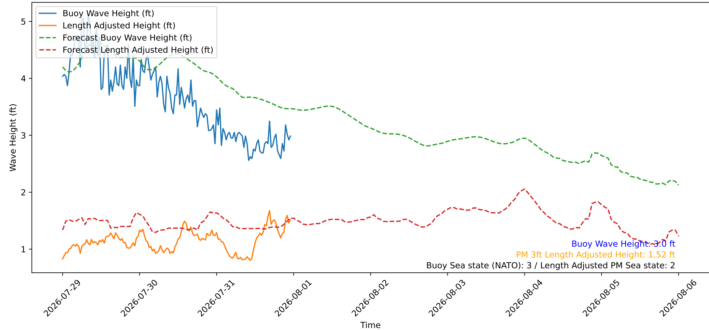
Wave Heights over Time for Red Beach at 2026-07-31 23:50:48
