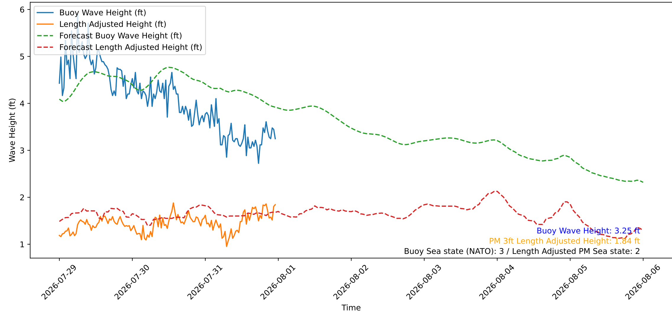
Wave Heights over Time for Oceanside Harbor at 2026-07-31 23:50:27
