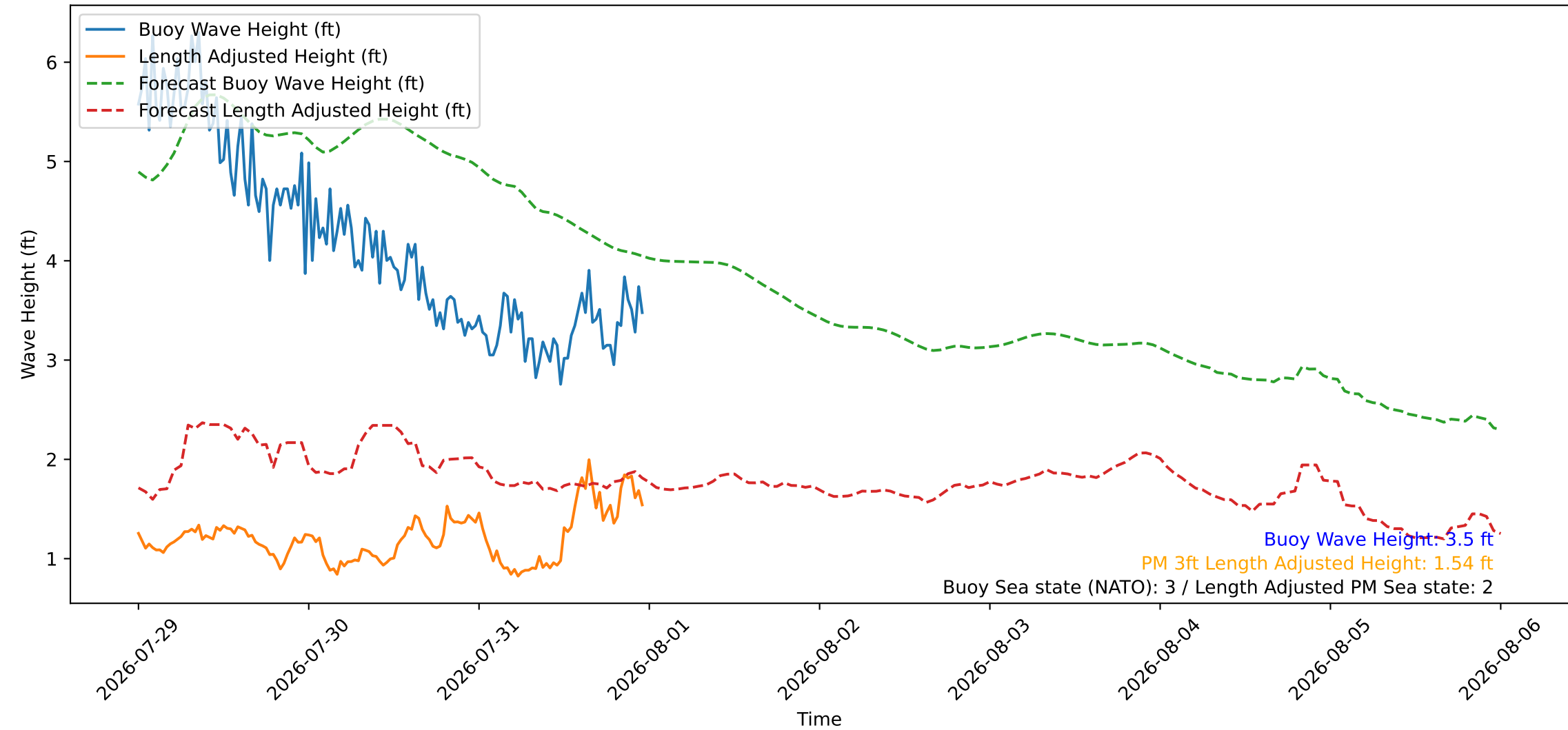
Wave Heights over Time for Green Beach at 2026-07-31 23:51:11
