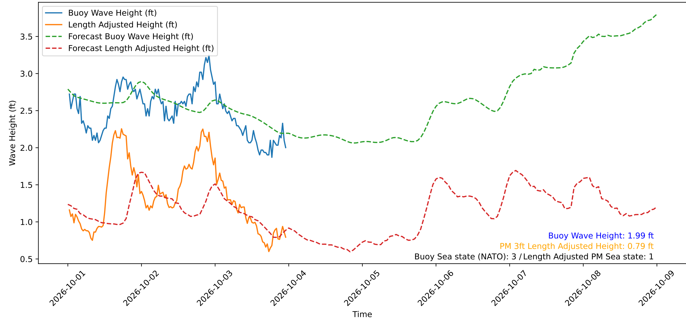
Wave Heights over Time for Red Beach at 2026-10-04 00:00:49
