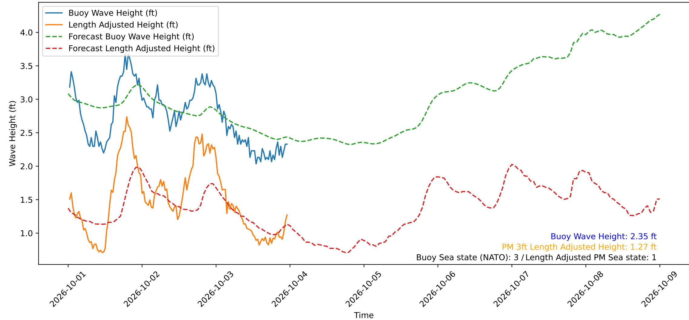
Wave Heights over Time for Green Beach at 2026-10-04 00:01:11
