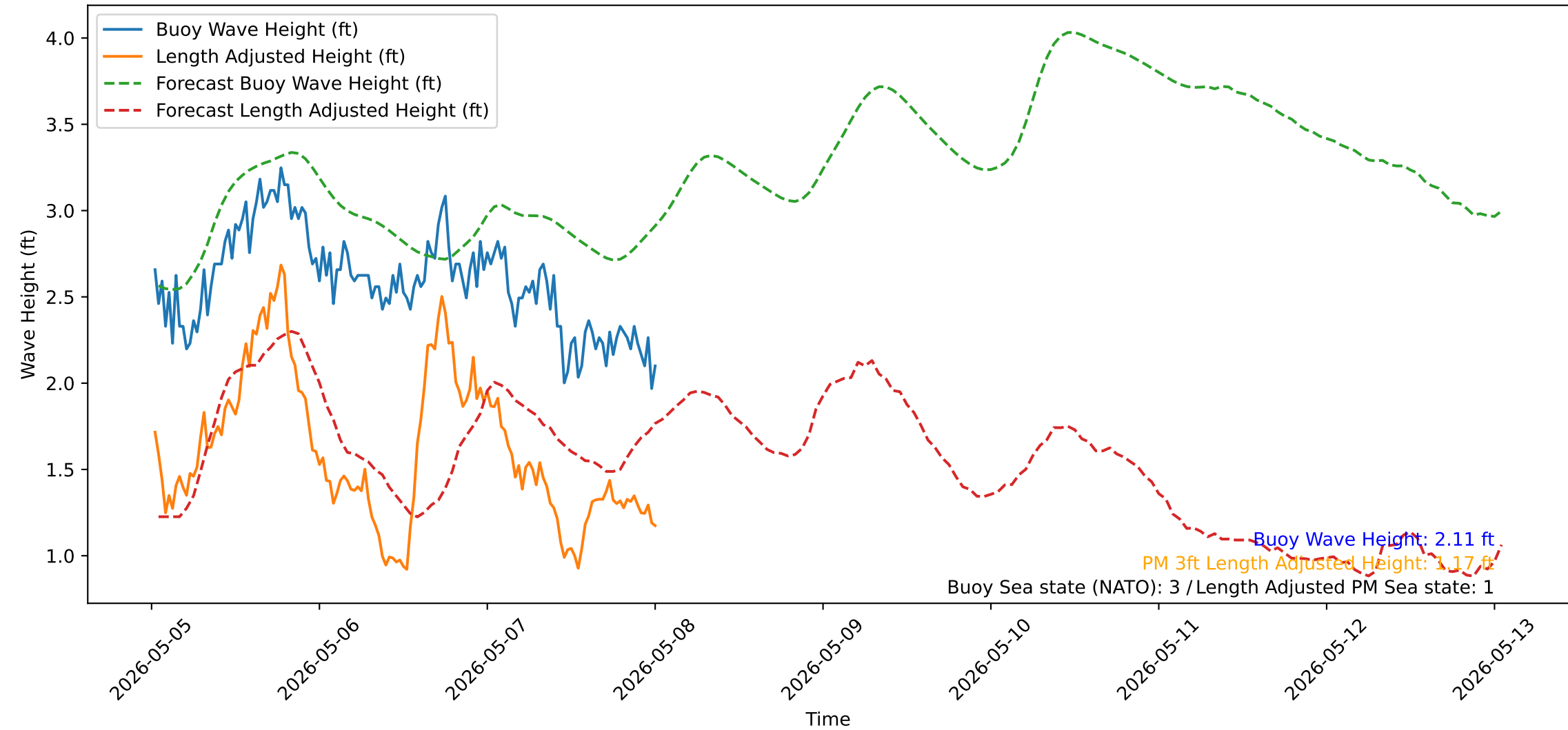
Wave Heights over Time for Oceanside Harbor at 2026-05-08 00:40:31
