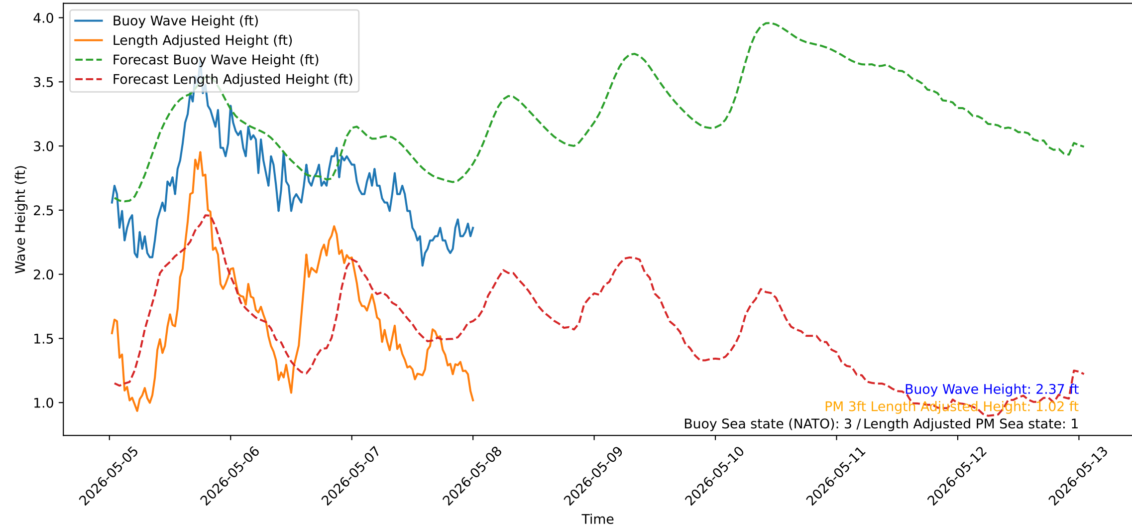
Wave Heights over Time for Green Beach at 2026-05-08 00:41:12
