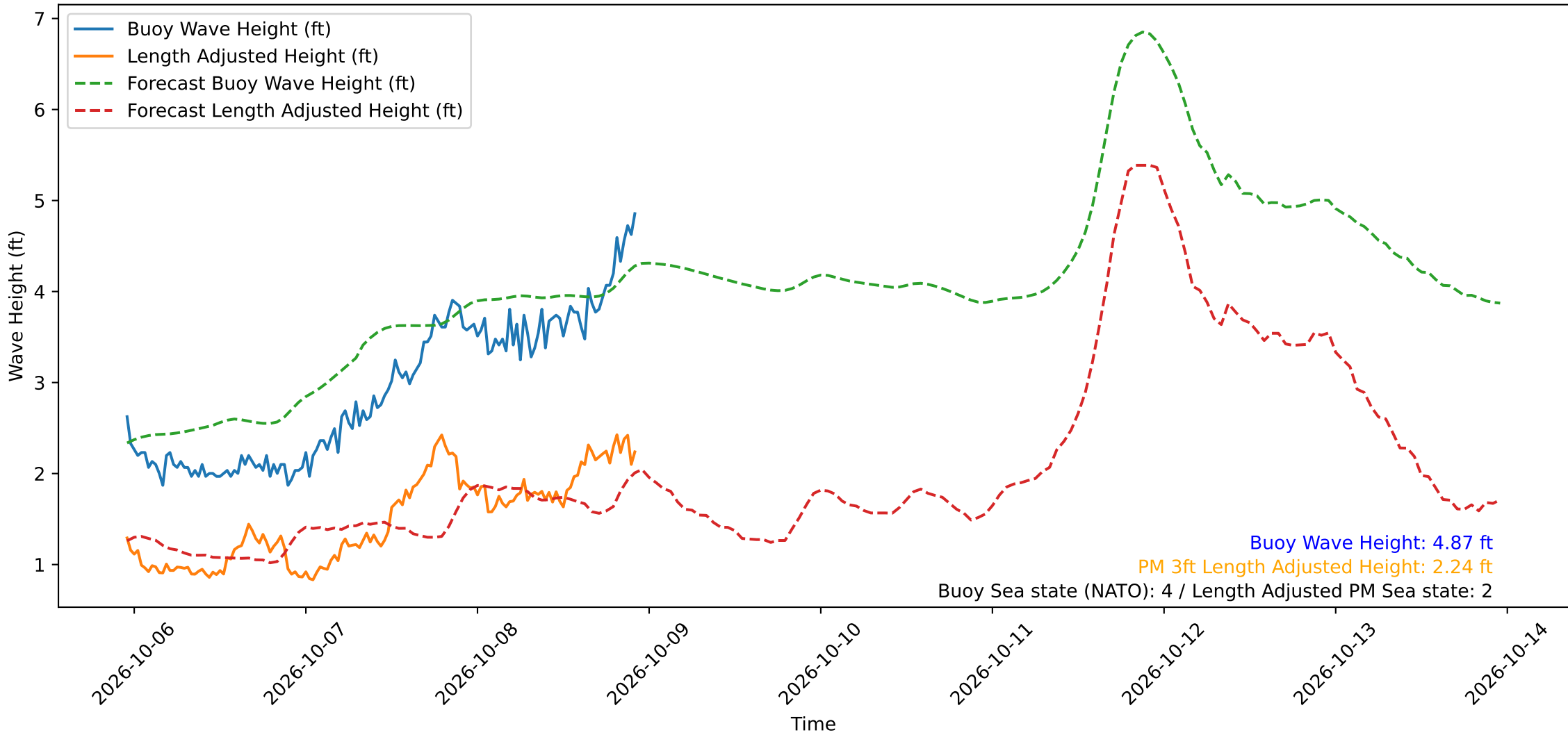
Wave Heights over Time for Red Beach at 2026-10-08 22:50:50
