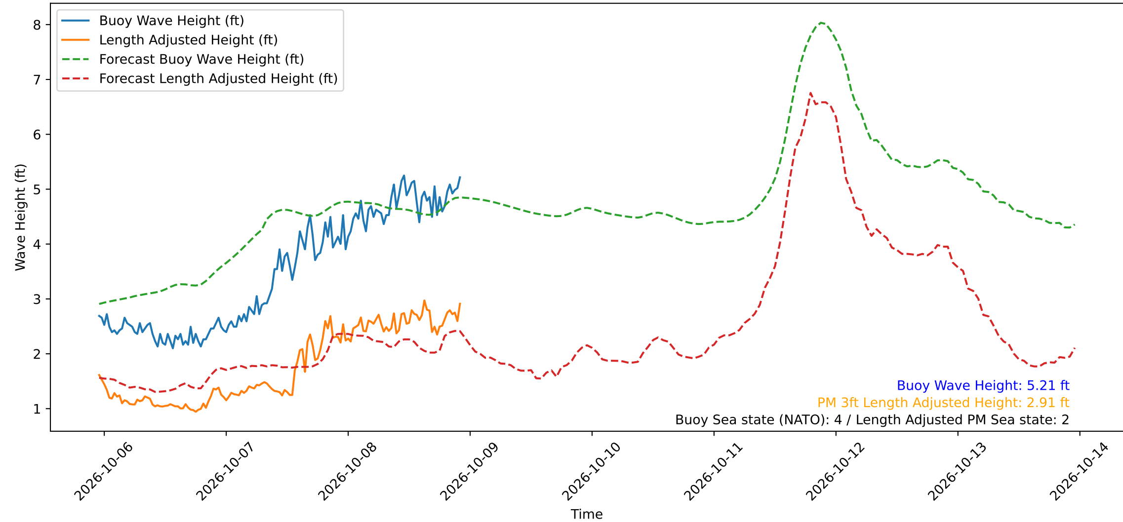
Wave Heights over Time for Green Beach at 2026-10-08 22:51:14
