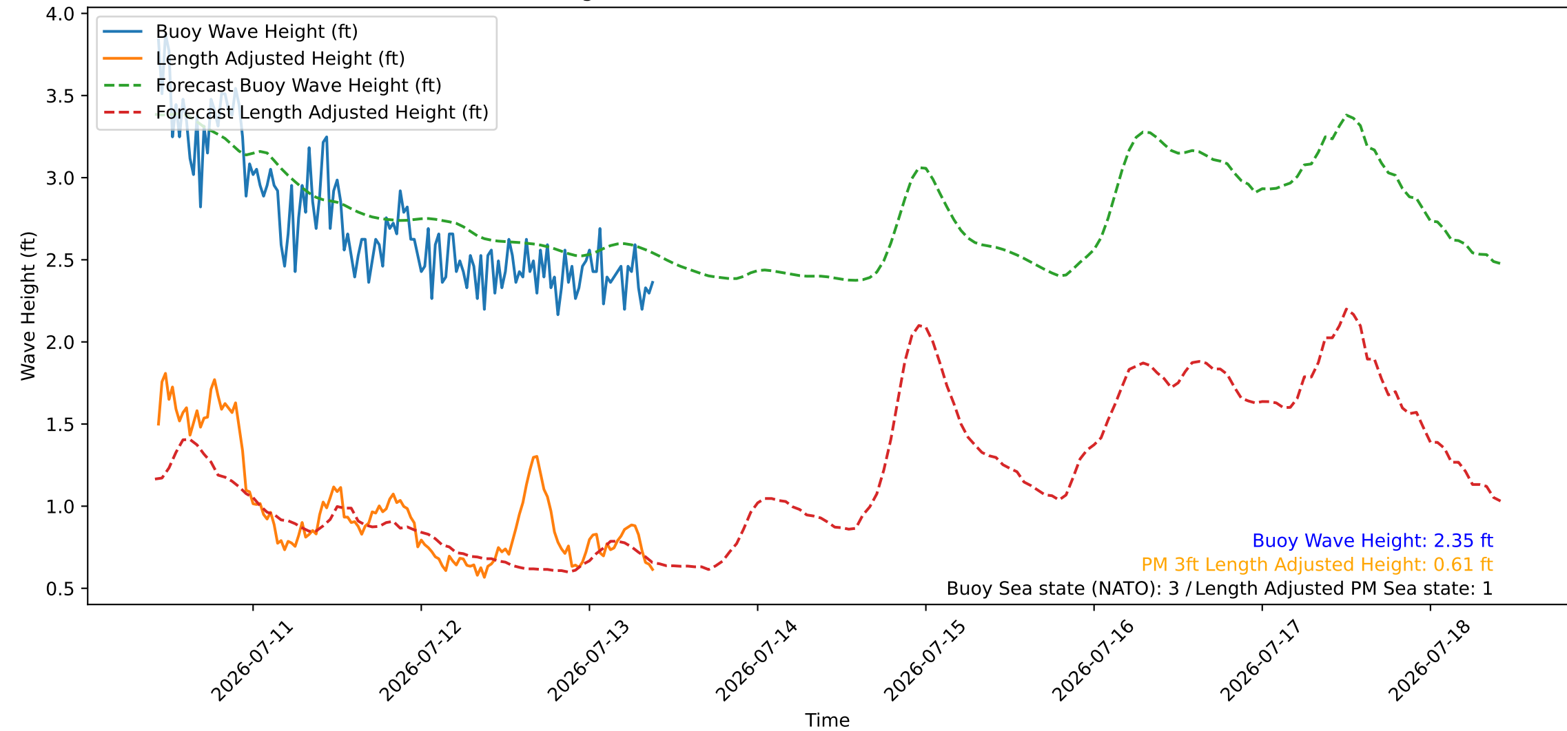
Wave Heights over Time for Red Beach at 2026-07-13 10:10:46
