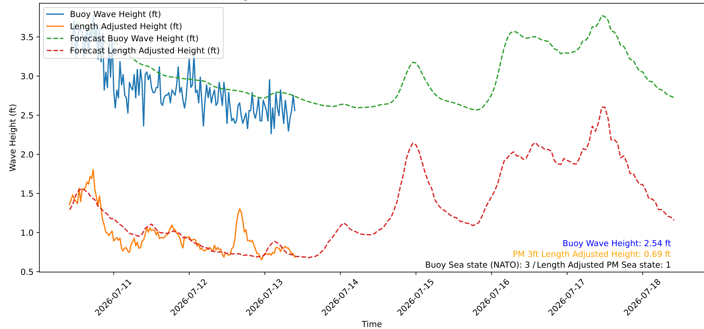
Wave Heights over Time for Oceanside Harbor at 2026-07-13 10:10:27
