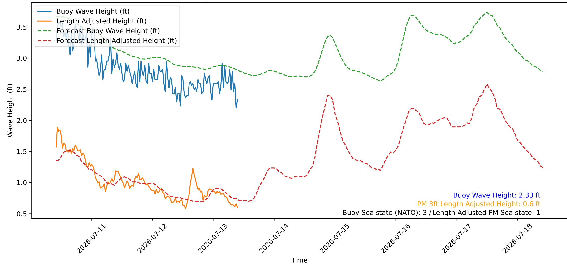
Wave Heights over Time for Green Beach at 2026-07-13 10:11:09
