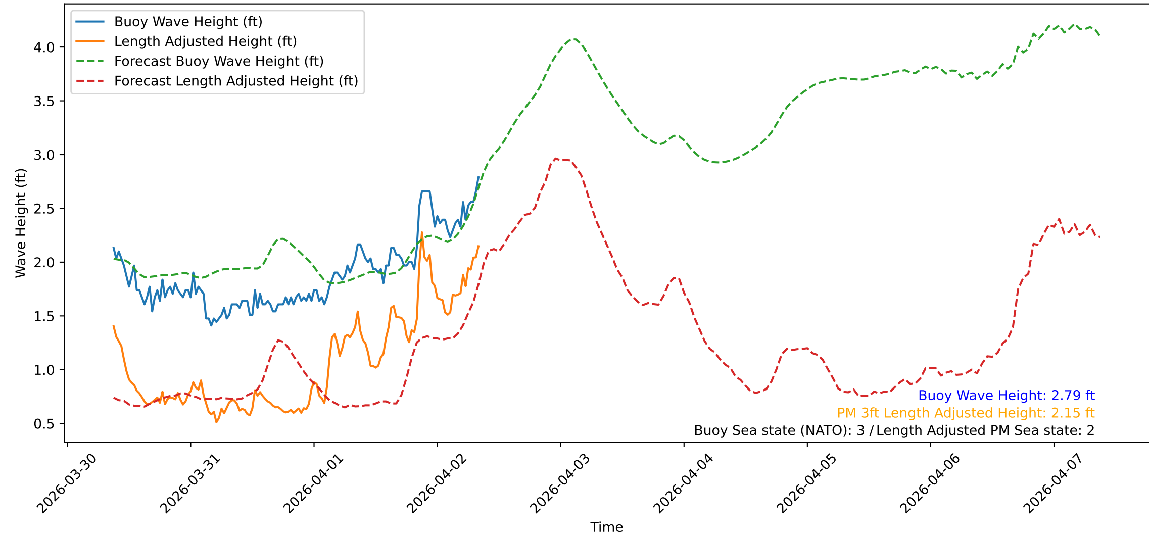
Wave Heights over Time for Green Beach at 2026-04-02 08:51:10
