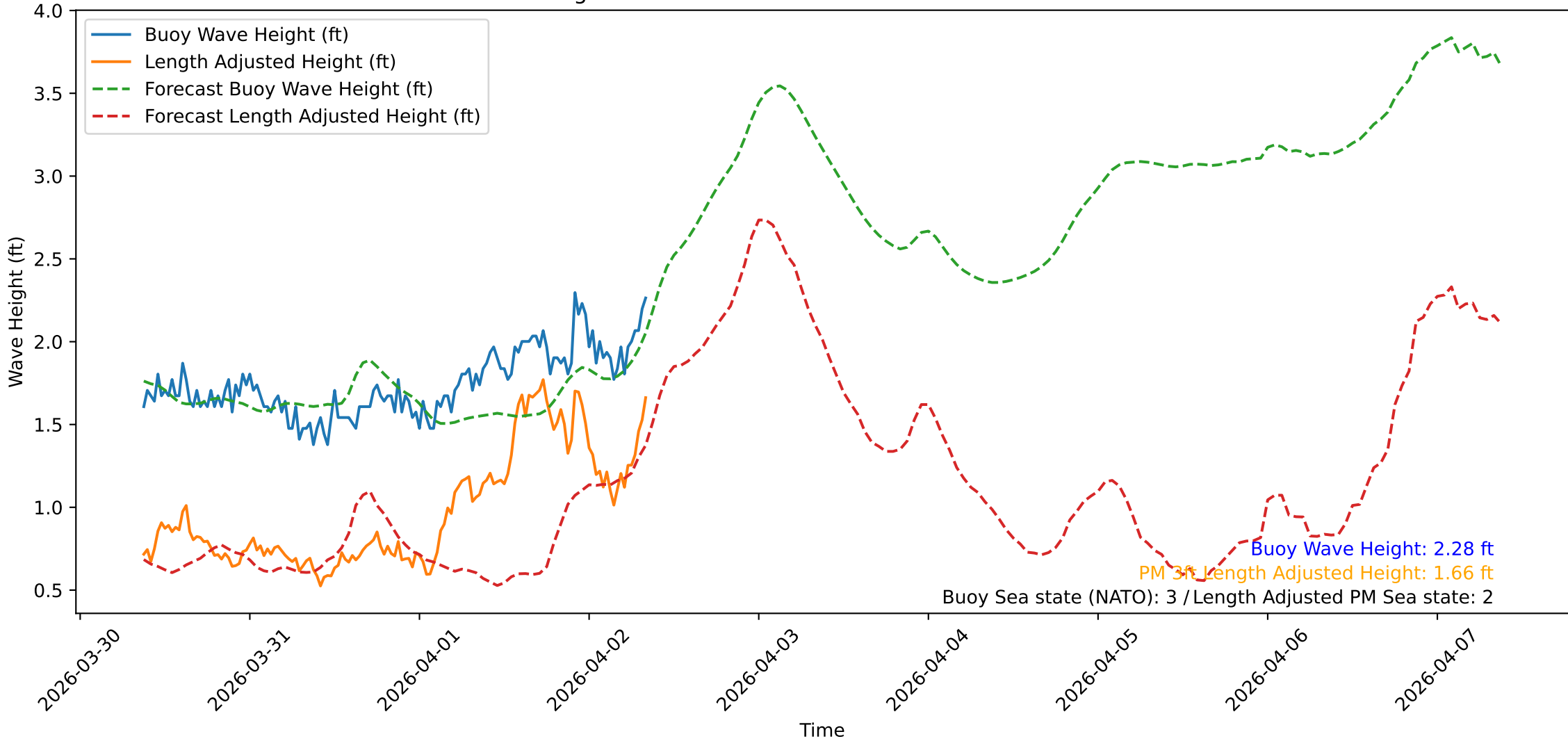
Wave Heights over Time for Red Beach at 2026-04-02 08:50:48
