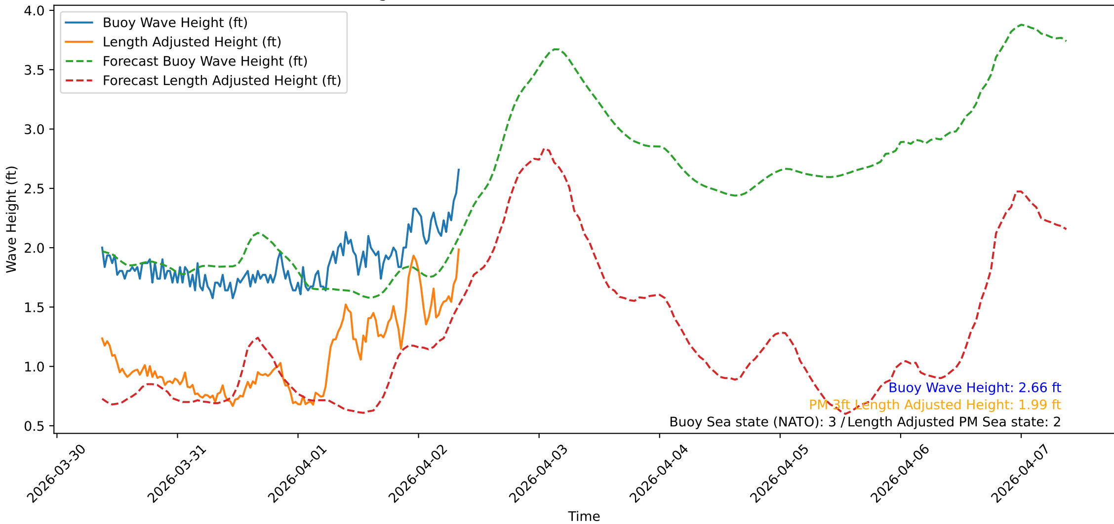
Wave Heights over Time for Oceanside Harbor at 2026-04-02 08:50:31
