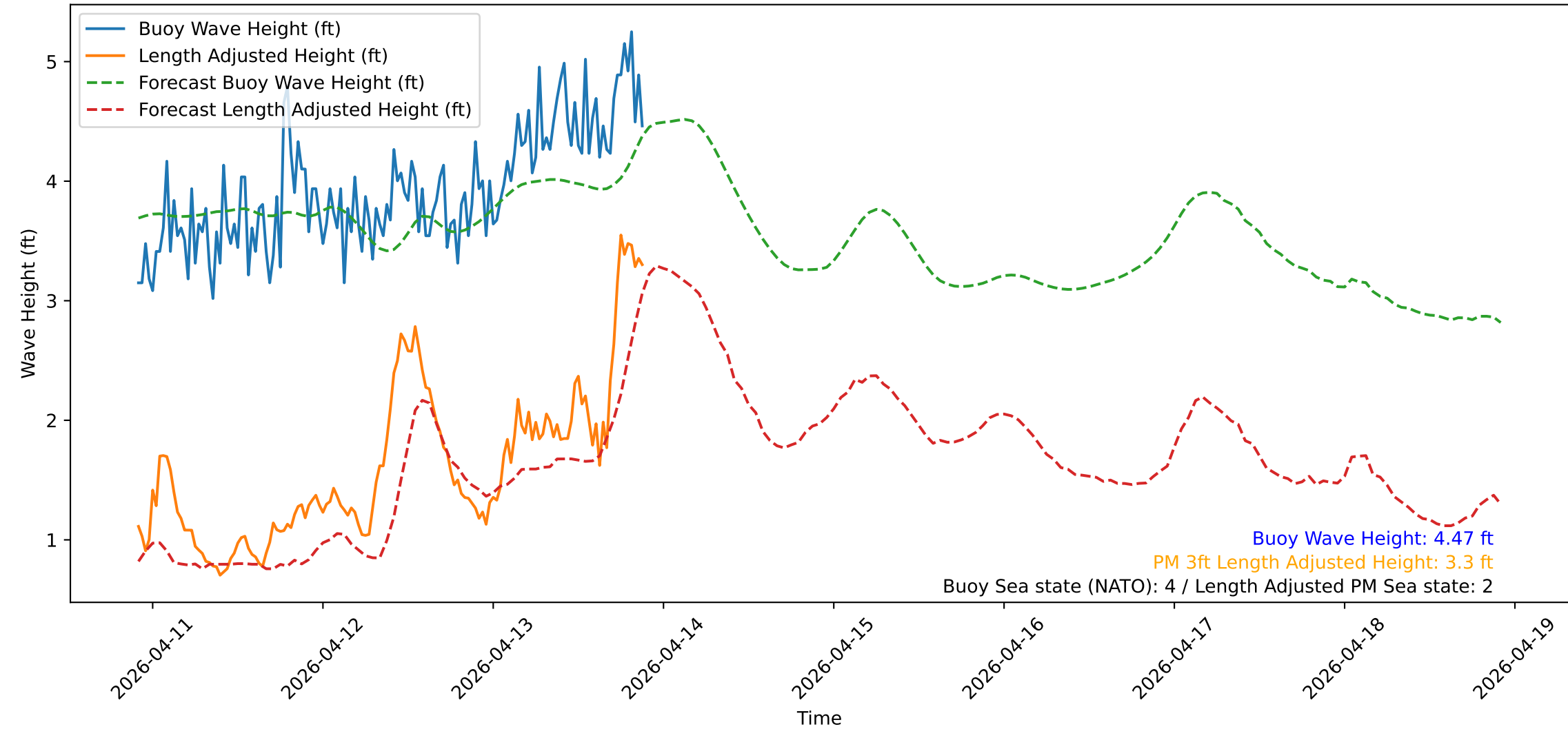
Wave Heights over Time for Oceanside Harbor at 2026-04-13 21:50:31
