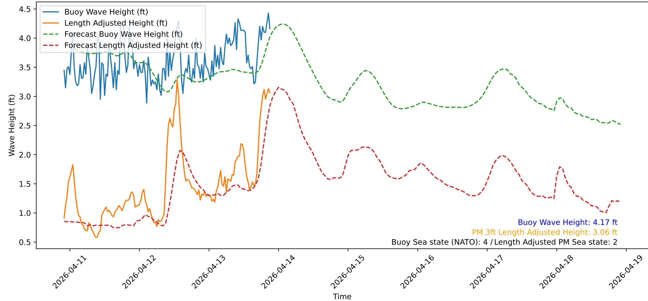
Wave Heights over Time for Red Beach at 2026-04-13 21:50:50
