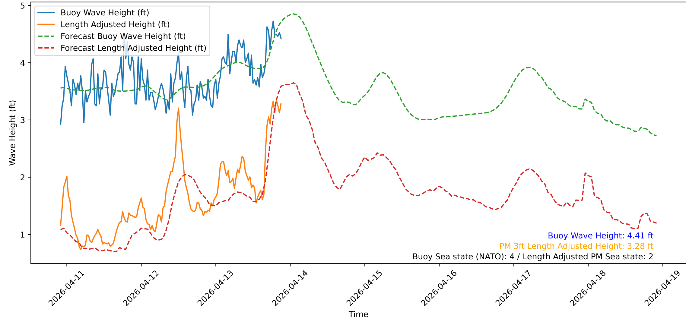
Wave Heights over Time for Green Beach at 2026-04-13 21:51:12
