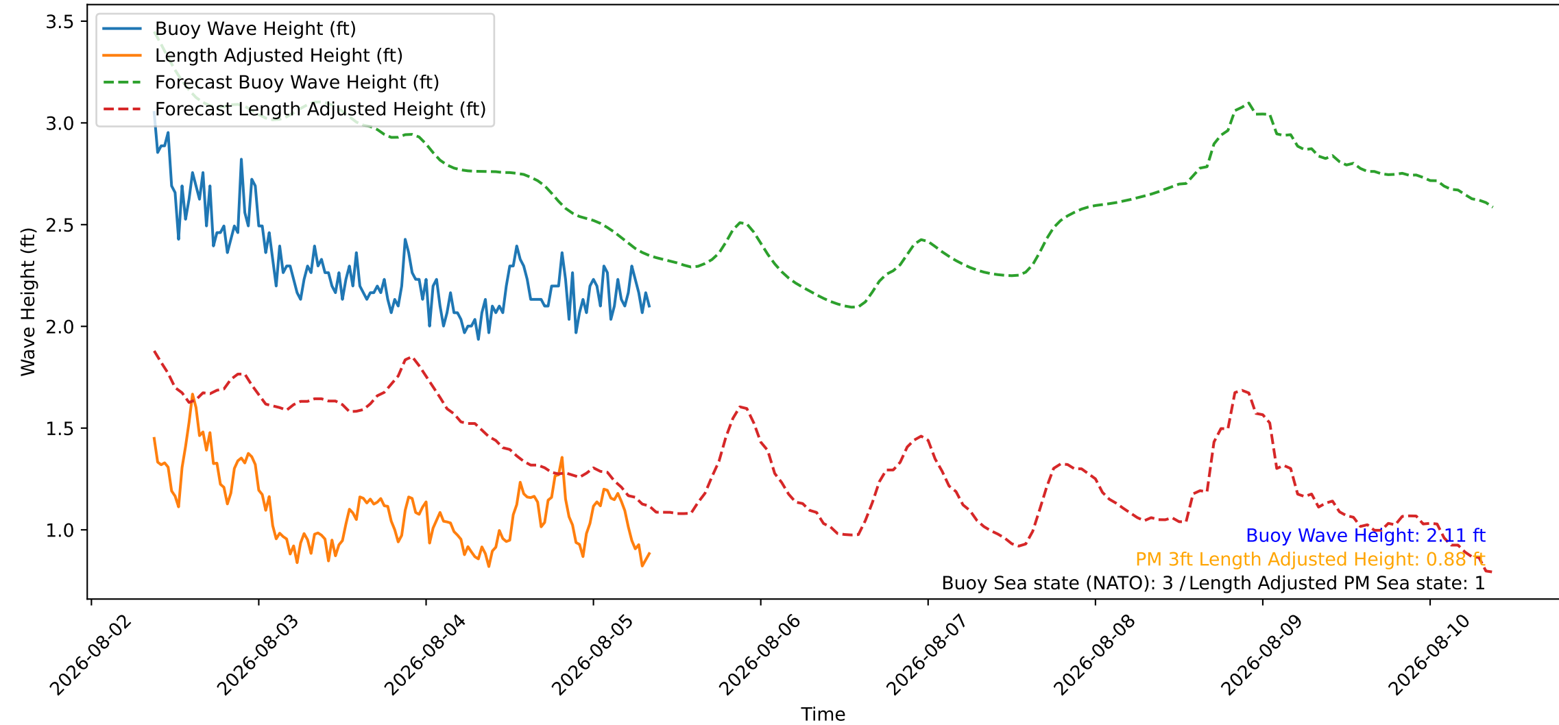
Wave Heights over Time for Green Beach at 2026-08-05 09:01:10
