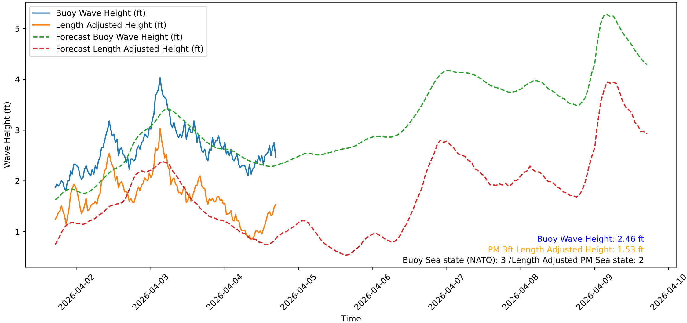
Wave Heights over Time for Oceanside Harbor at 2026-04-04 17:00:32
