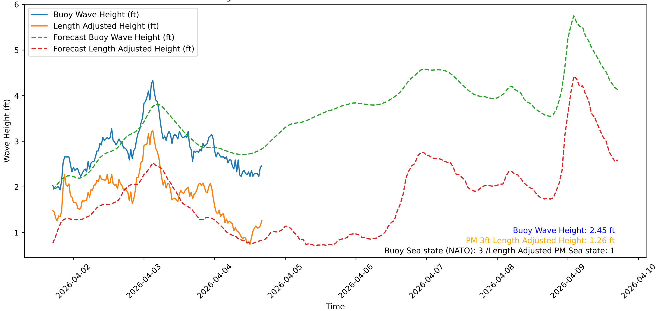
Wave Heights over Time for Green Beach at 2026-04-04 17:01:12
