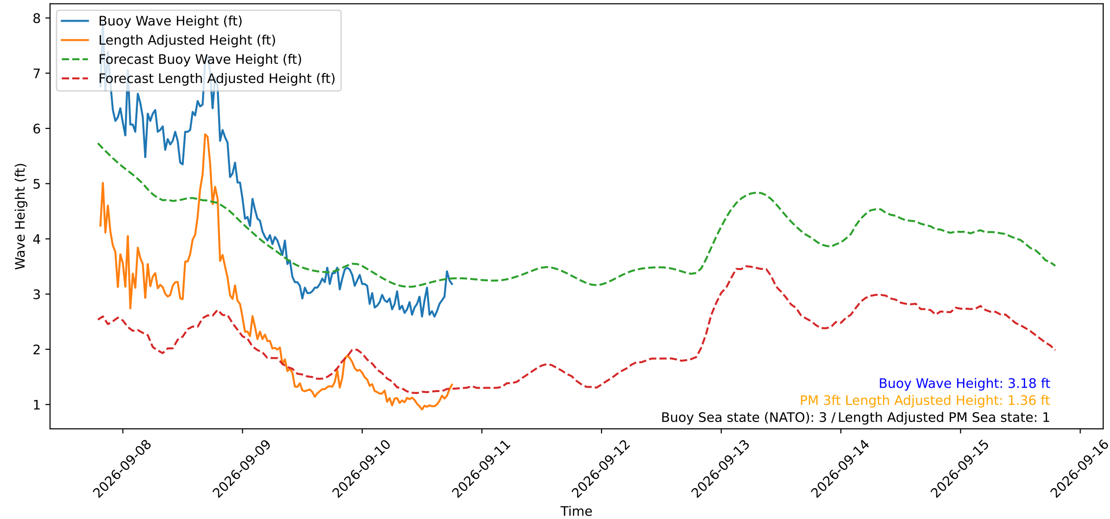
Wave Heights over Time for Green Beach at 2026-09-10 19:01:12
