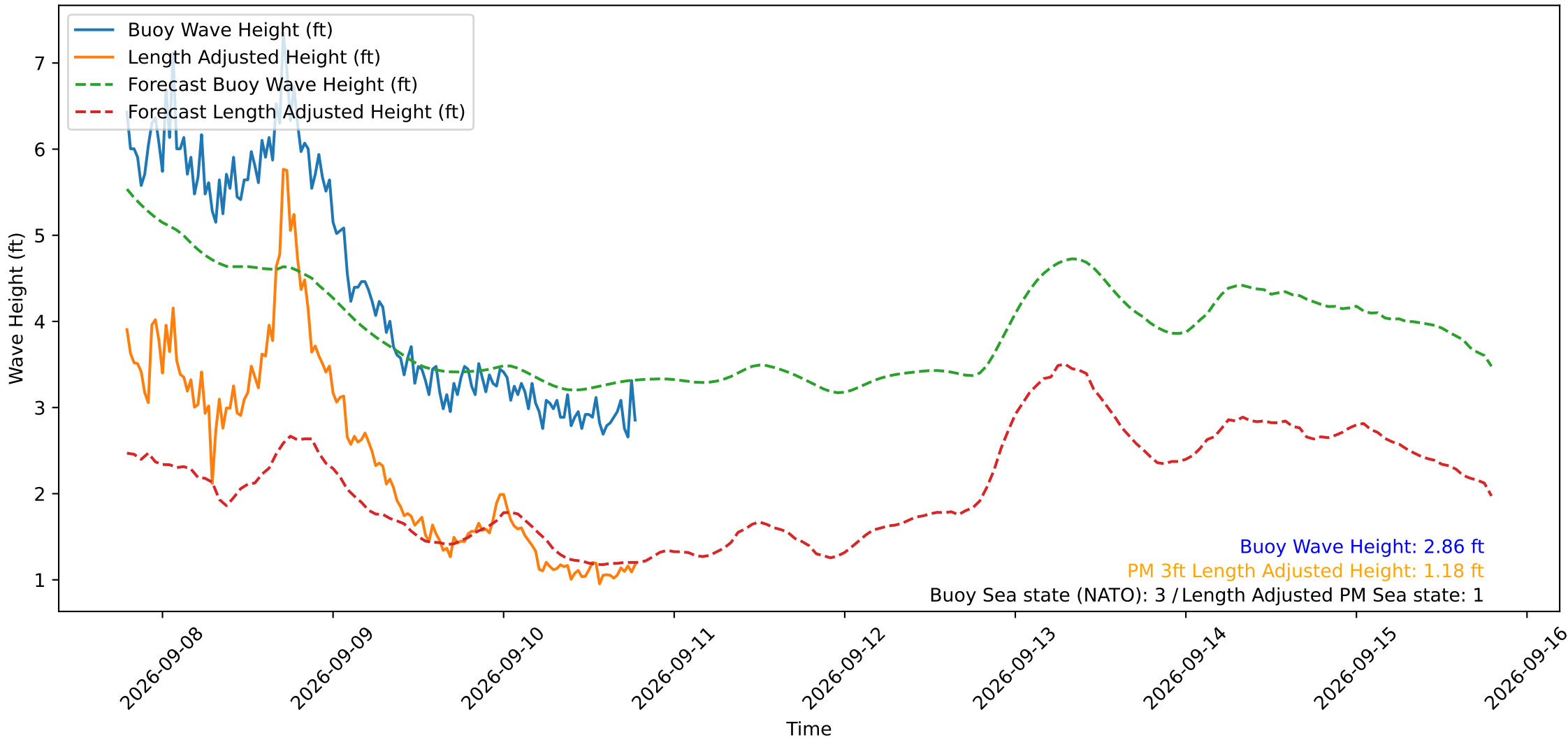
Wave Heights over Time for Oceanside Harbor at 2026-09-10 19:00:30
