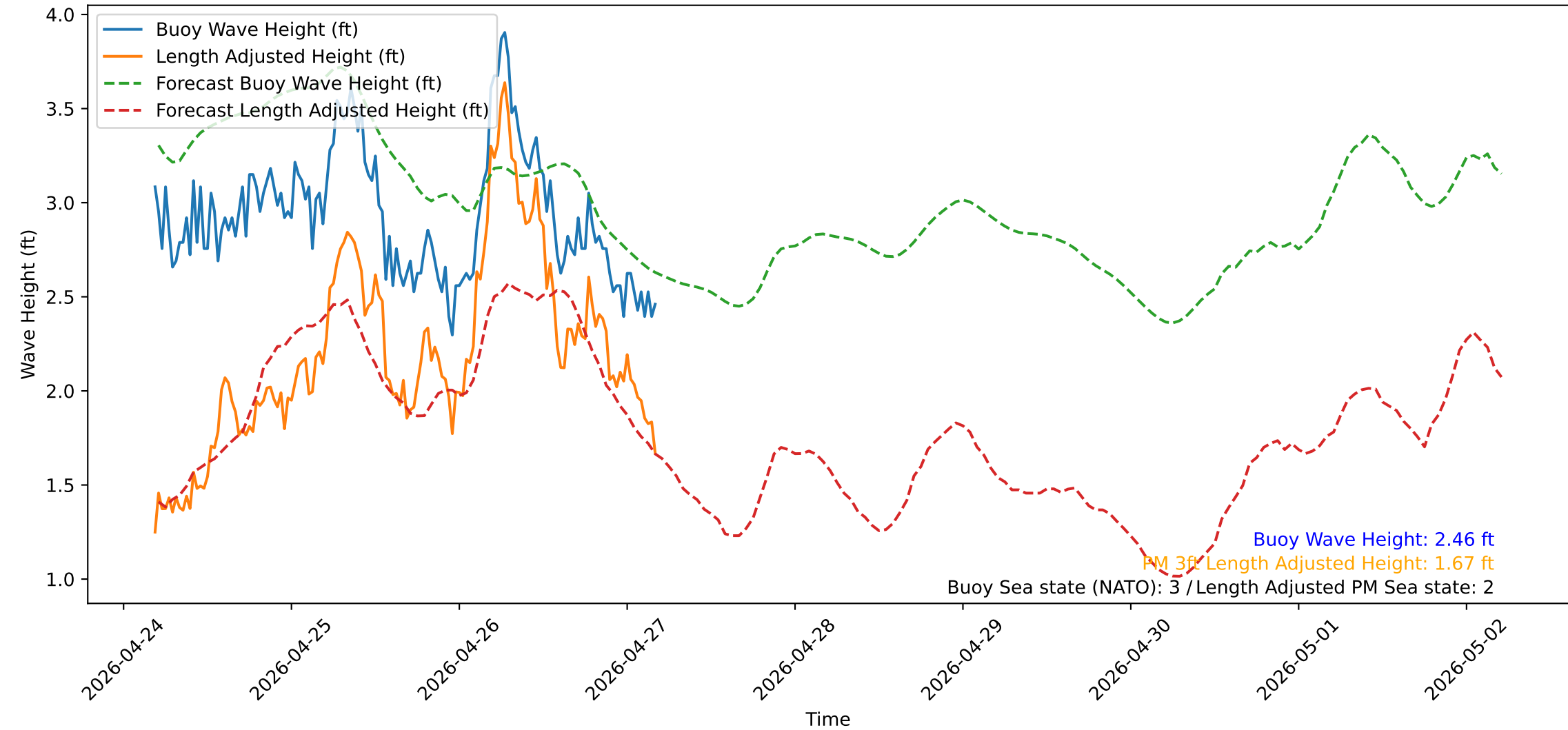
Wave Heights over Time for Oceanside Harbor at 2026-04-27 04:30:31
