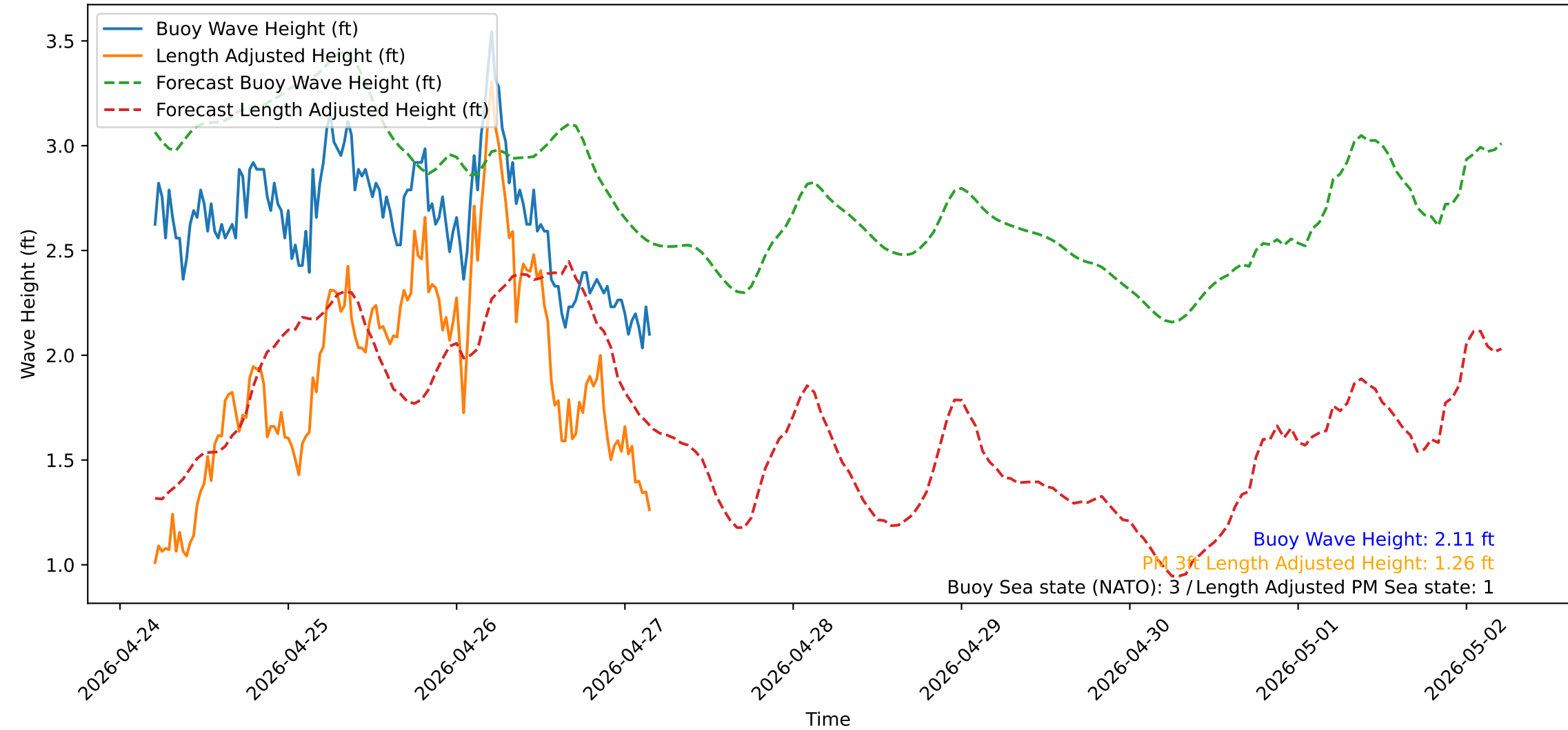
Wave Heights over Time for Red Beach at 2026-04-27 04:30:50
