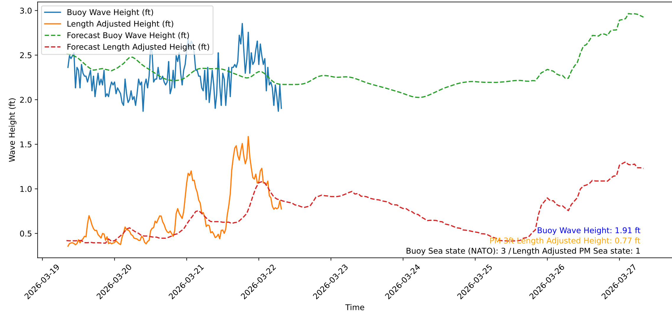
Wave Heights over Time for Red Beach at 2026-03-22 08:20:48
