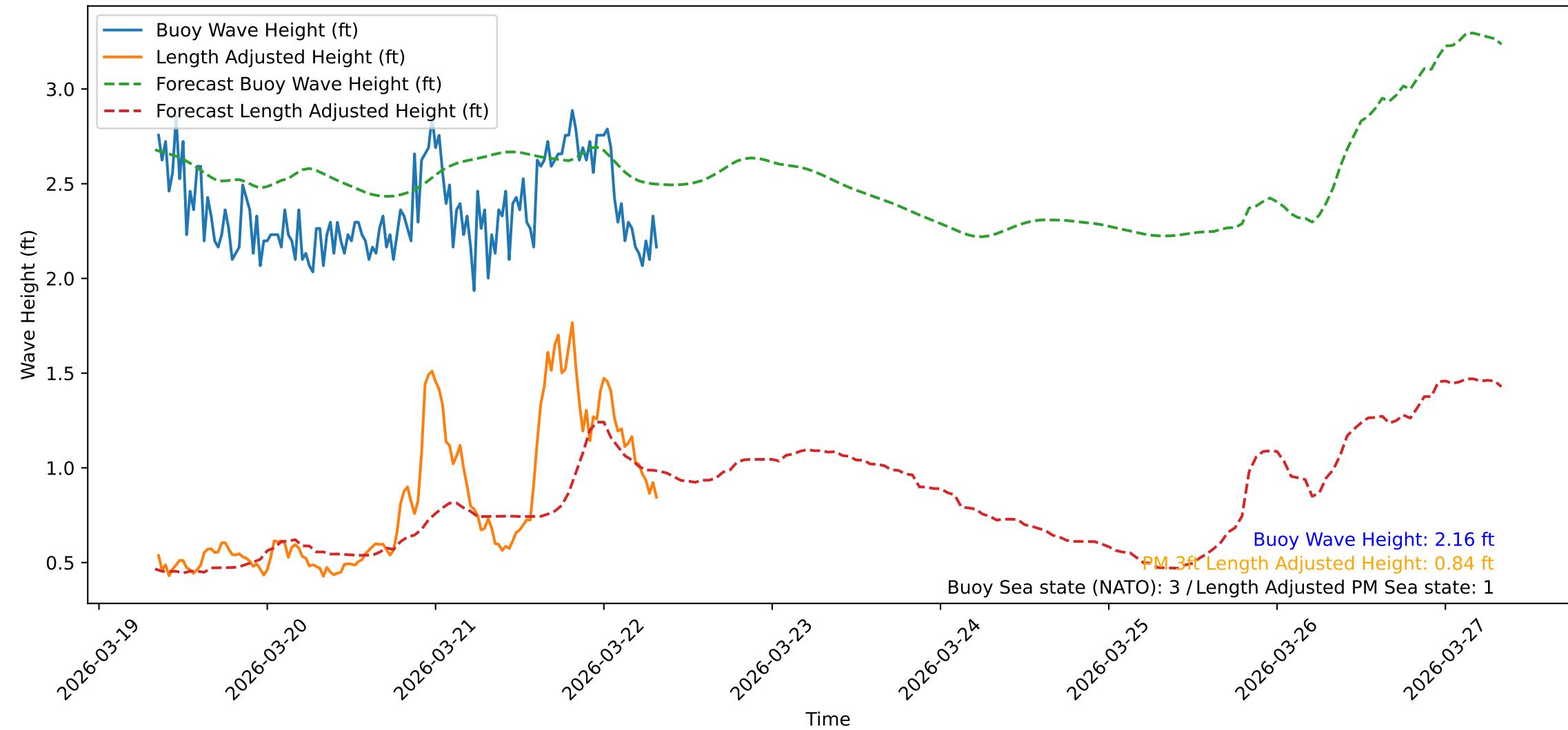
Wave Heights over Time for Green Beach at 2026-03-22 08:21:10
