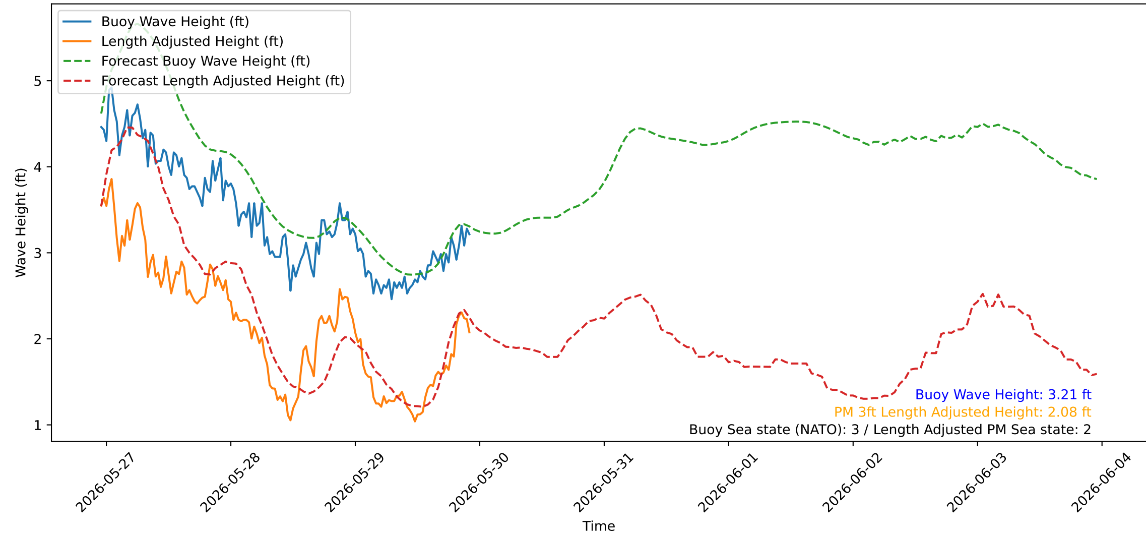
Wave Heights over Time for Green Beach at 2026-05-29 22:51:06
