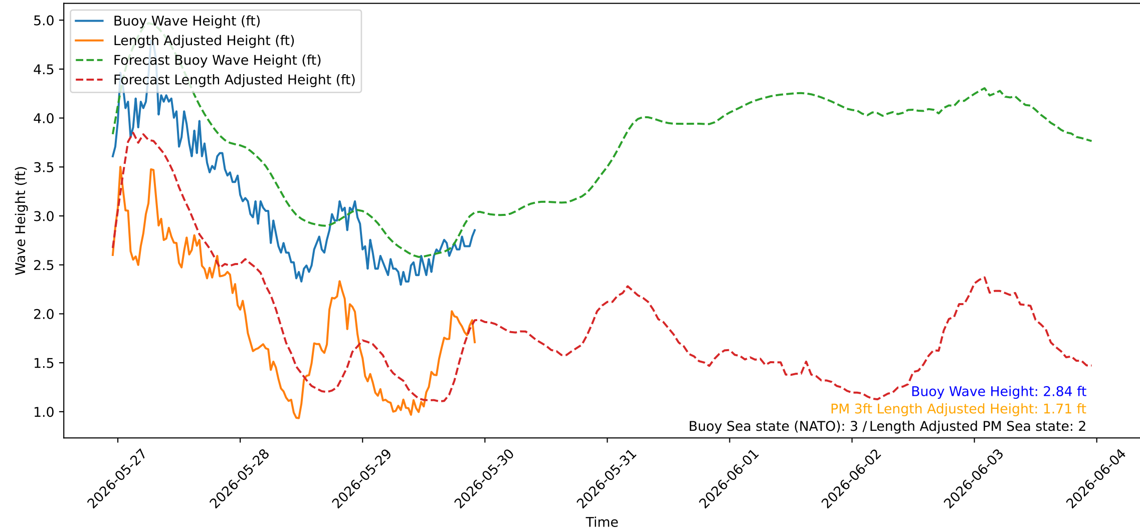
Wave Heights over Time for Red Beach at 2026-05-29 22:50:43
