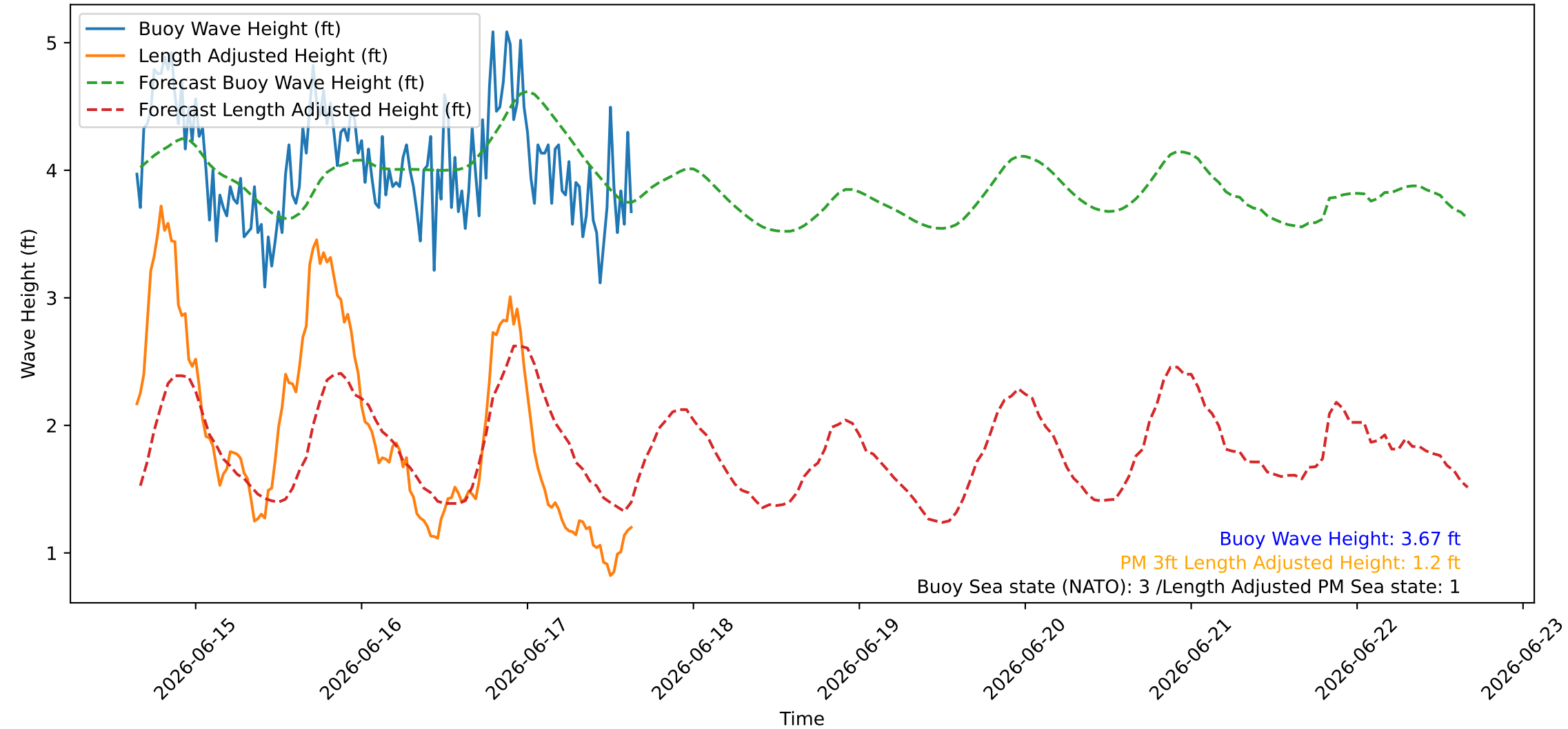
Wave Heights over Time for Green Beach at 2026-06-17 15:41:09
