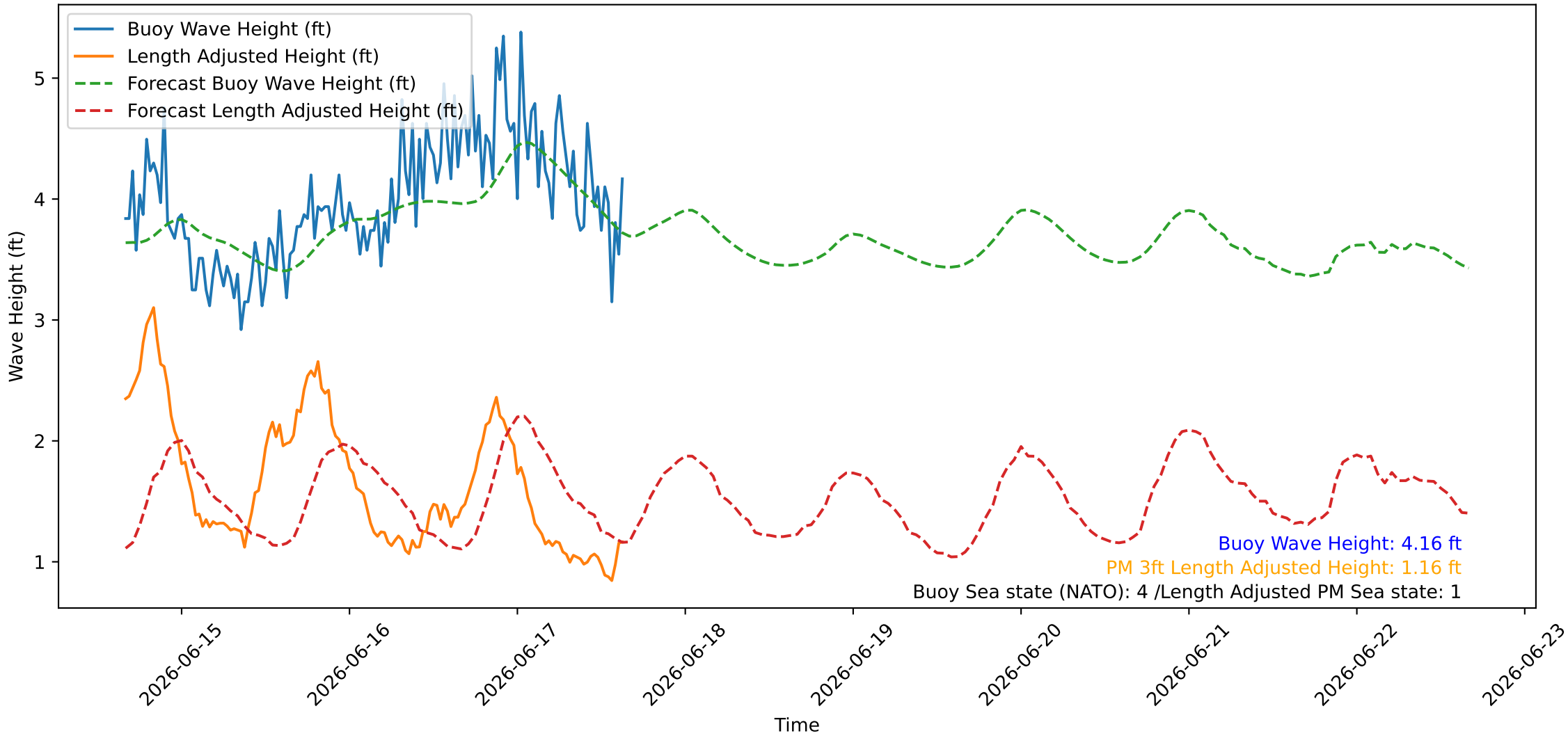
Wave Heights over Time for Red Beach at 2026-06-17 15:40:46
