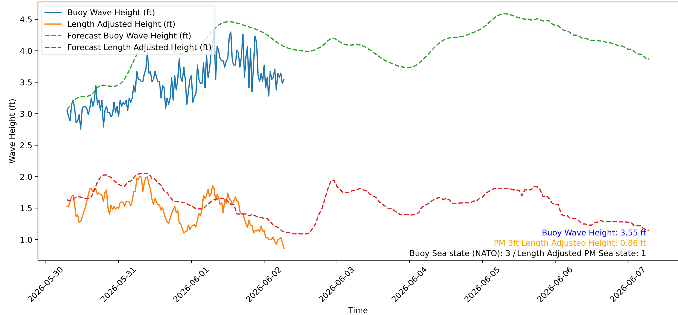
Wave Heights over Time for Green Beach at 2026-06-02 07:11:07
