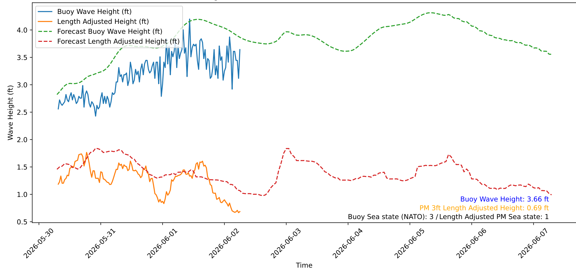
Wave Heights over Time for Red Beach at 2026-06-02 07:10:45
