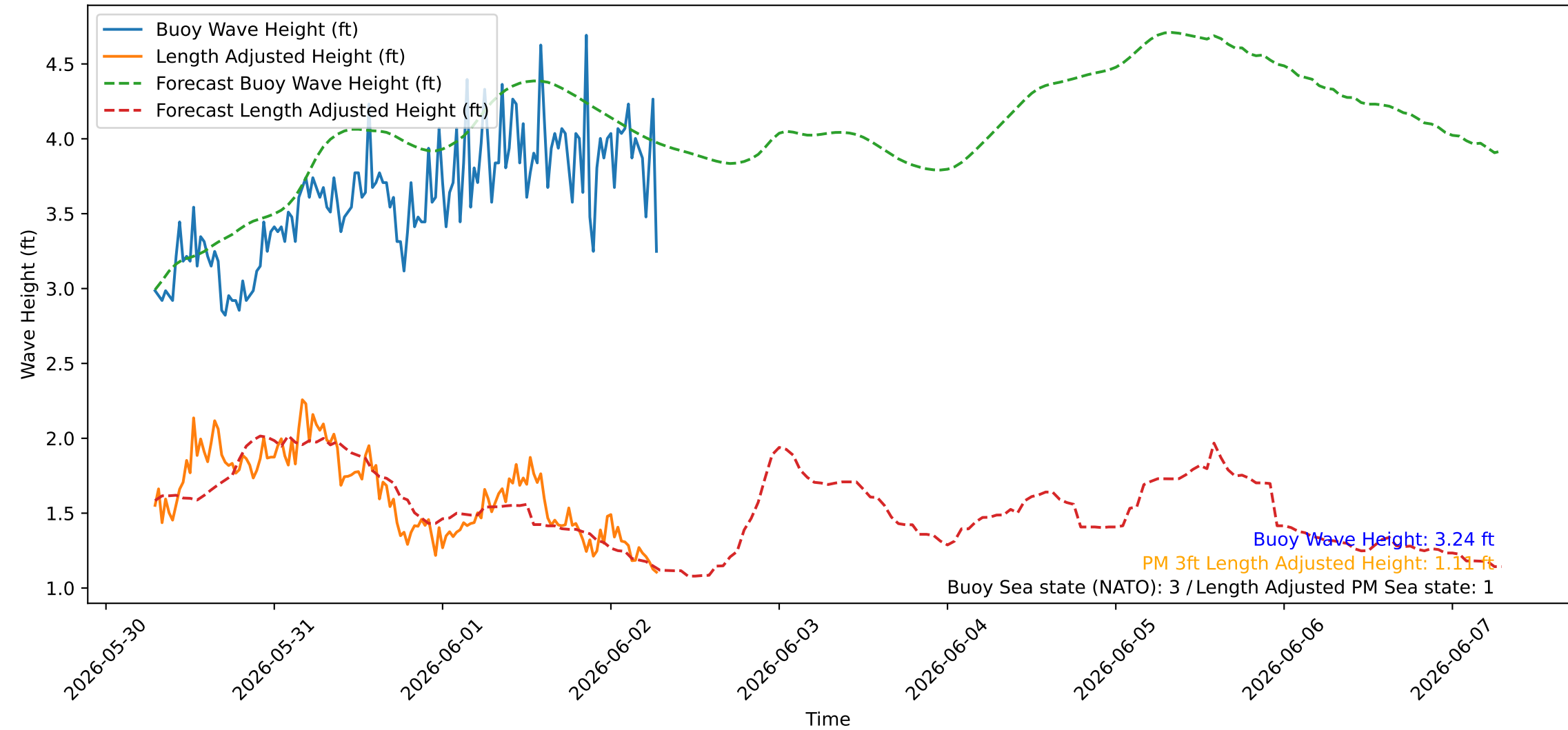
Wave Heights over Time for Oceanside Harbor at 2026-06-02 07:10:26
