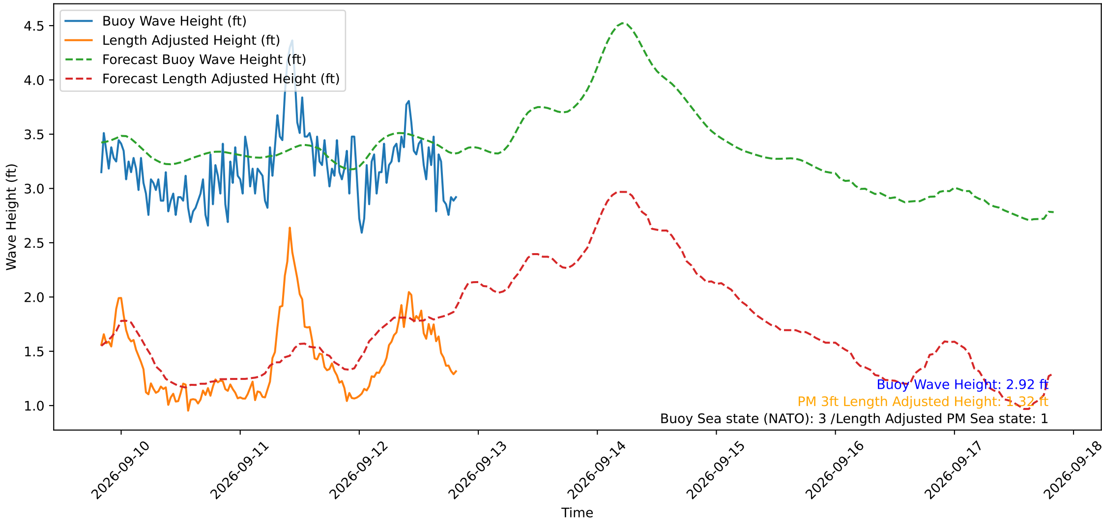
Wave Heights over Time for Oceanside Harbor at 2026-09-12 20:10:30
