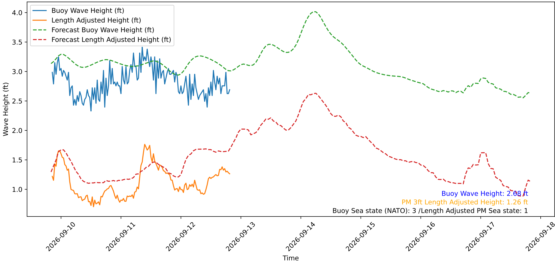
Wave Heights over Time for Red Beach at 2026-09-12 20:10:49
