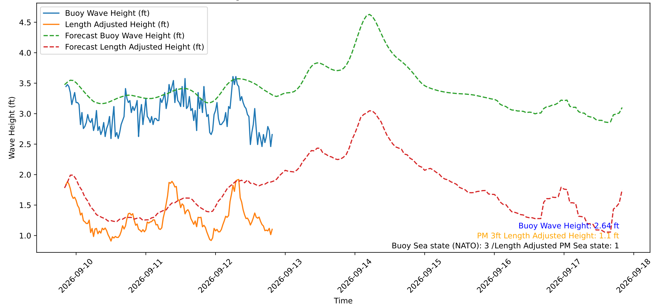
Wave Heights over Time for Green Beach at 2026-09-12 20:11:11
