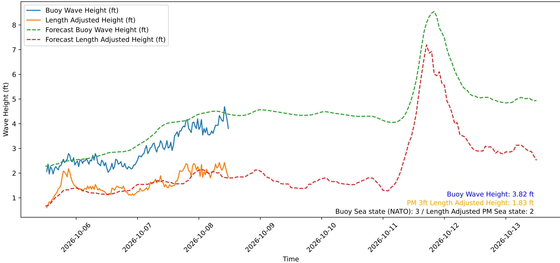
Wave Heights over Time for Oceanside Harbor at 2026-10-08 12:20:31
