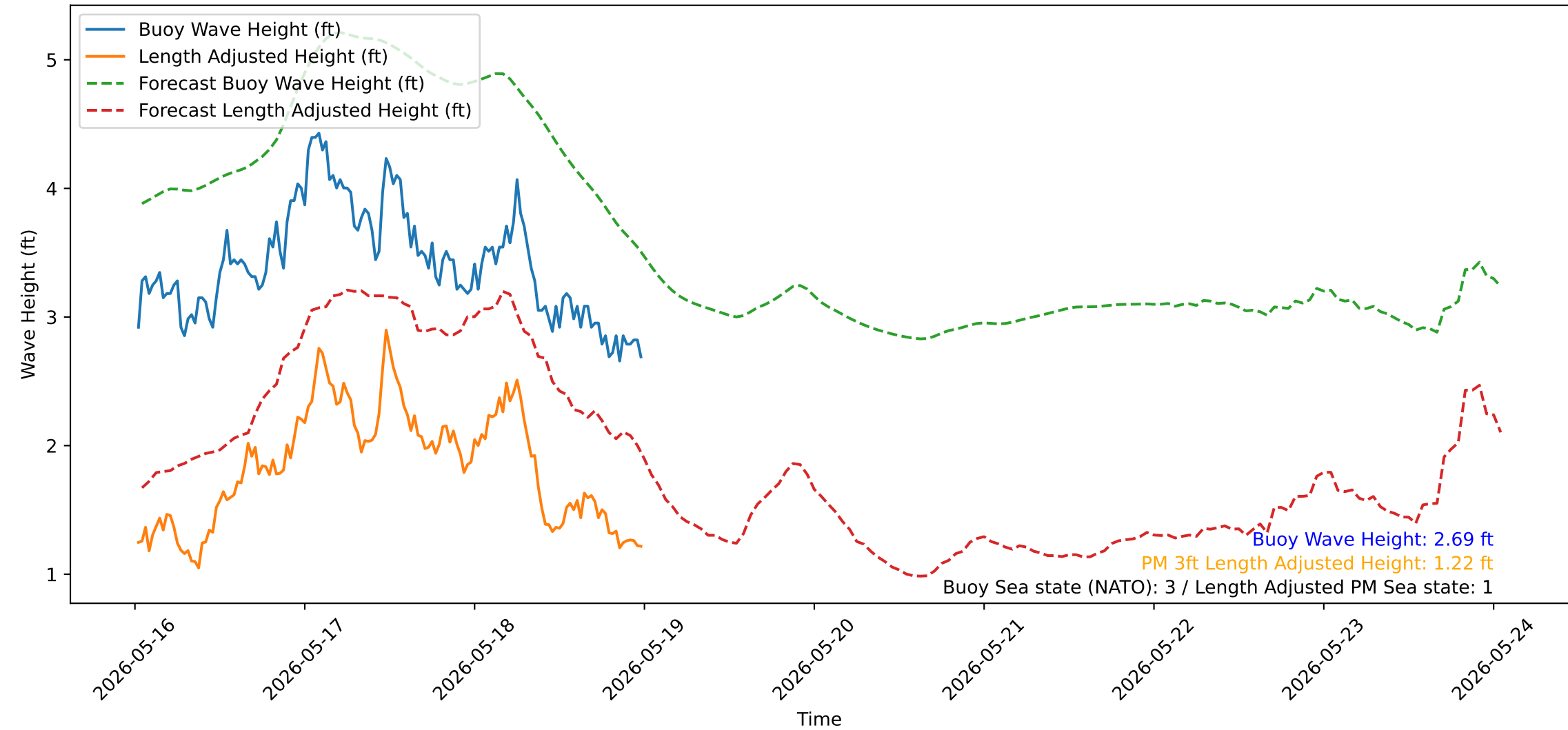
Wave Heights over Time for Green Beach at 2026-05-19 00:31:14
