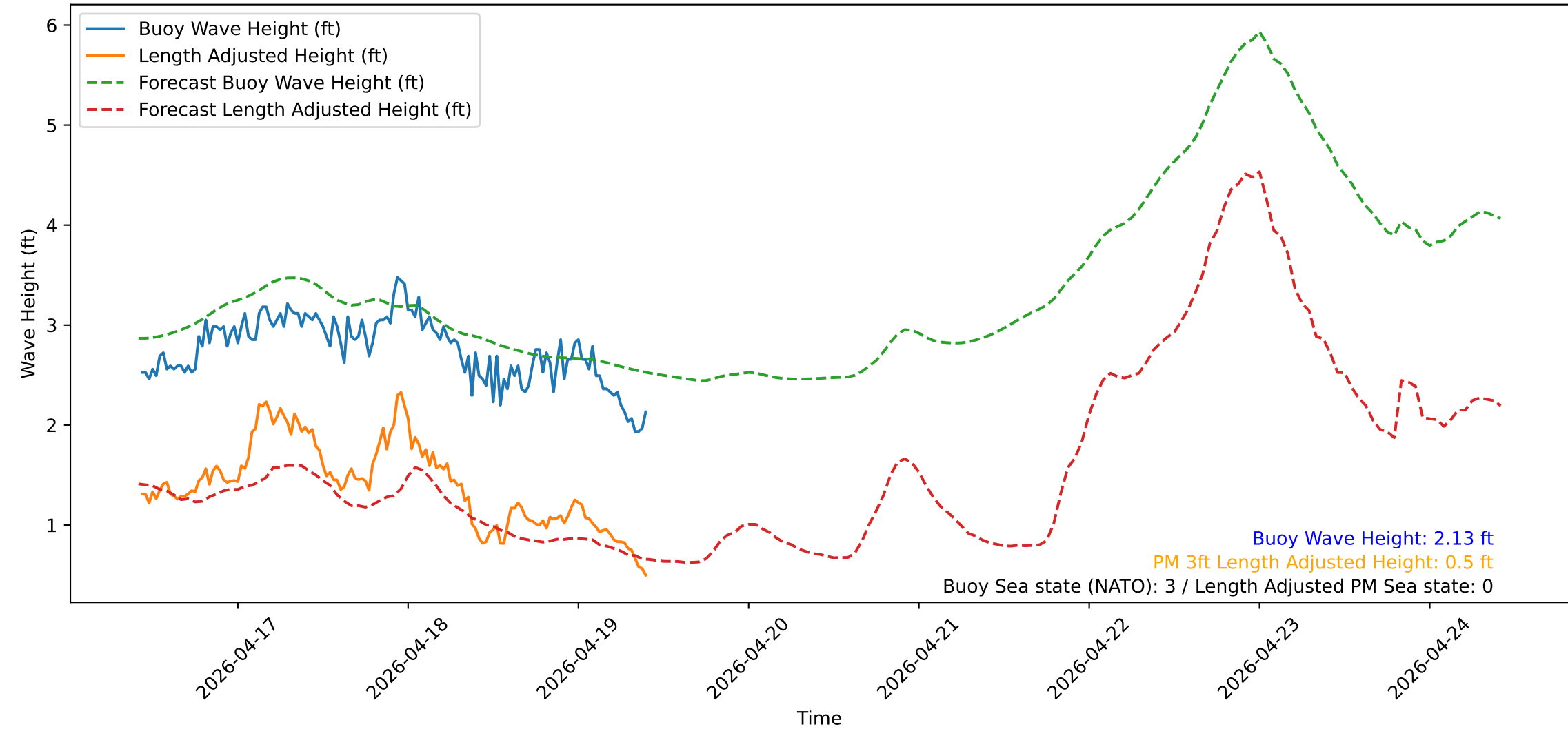
Wave Heights over Time for Green Beach at 2026-04-19 10:21:14
