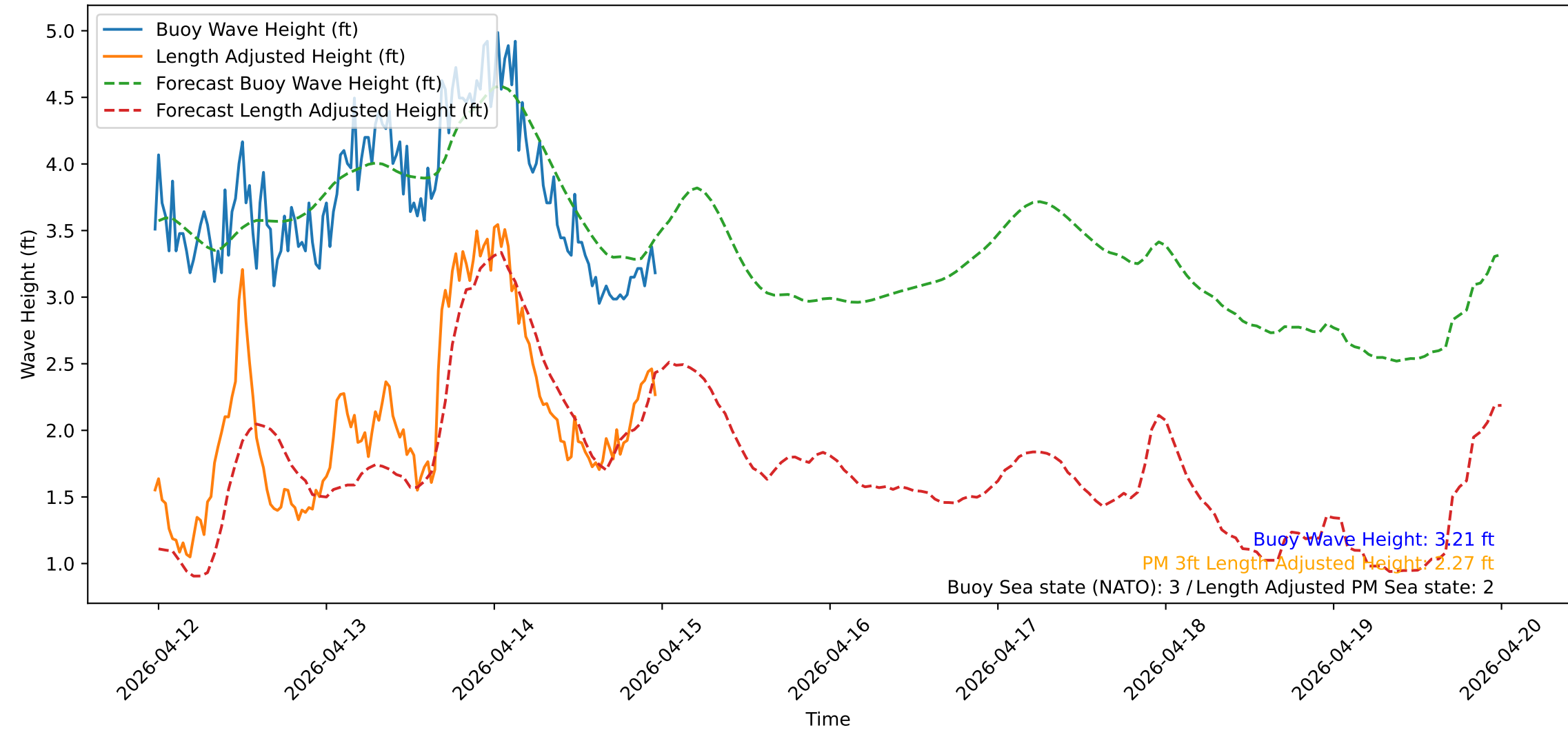
Wave Heights over Time for Green Beach at 2026-04-14 23:41:12
