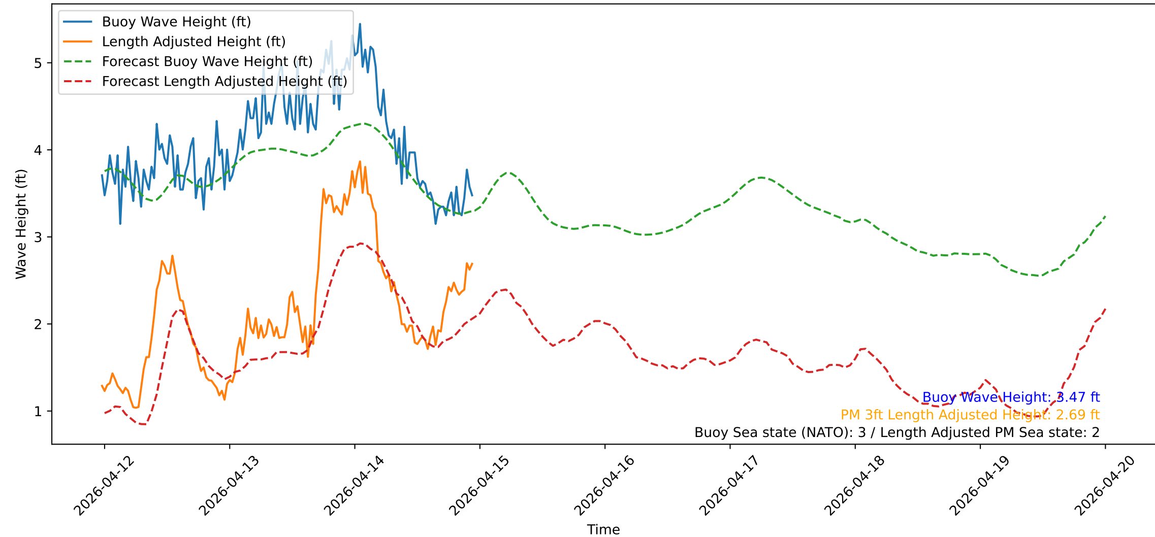
Wave Heights over Time for Oceanside Harbor at 2026-04-14 23:40:30
