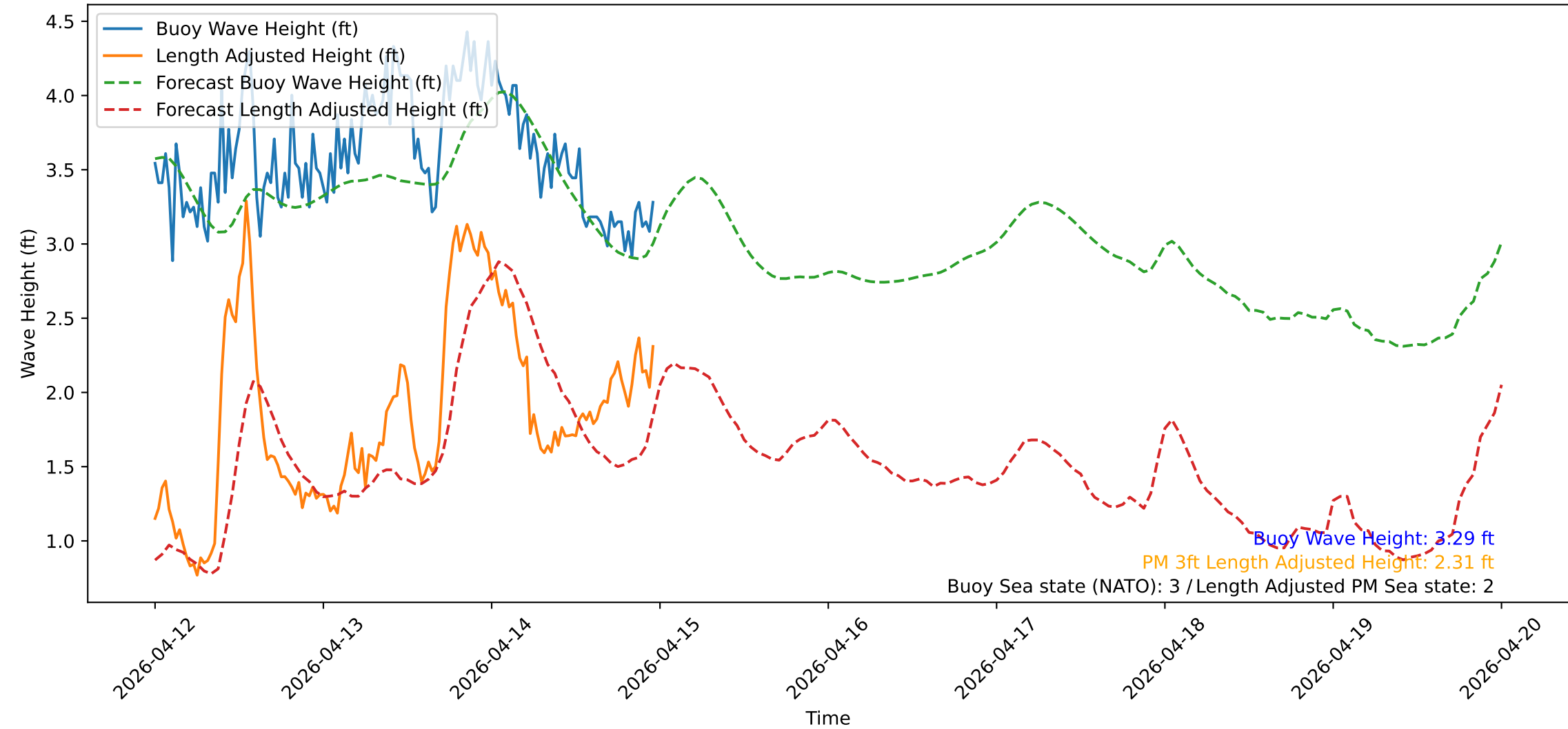
Wave Heights over Time for Red Beach at 2026-04-14 23:40:50
