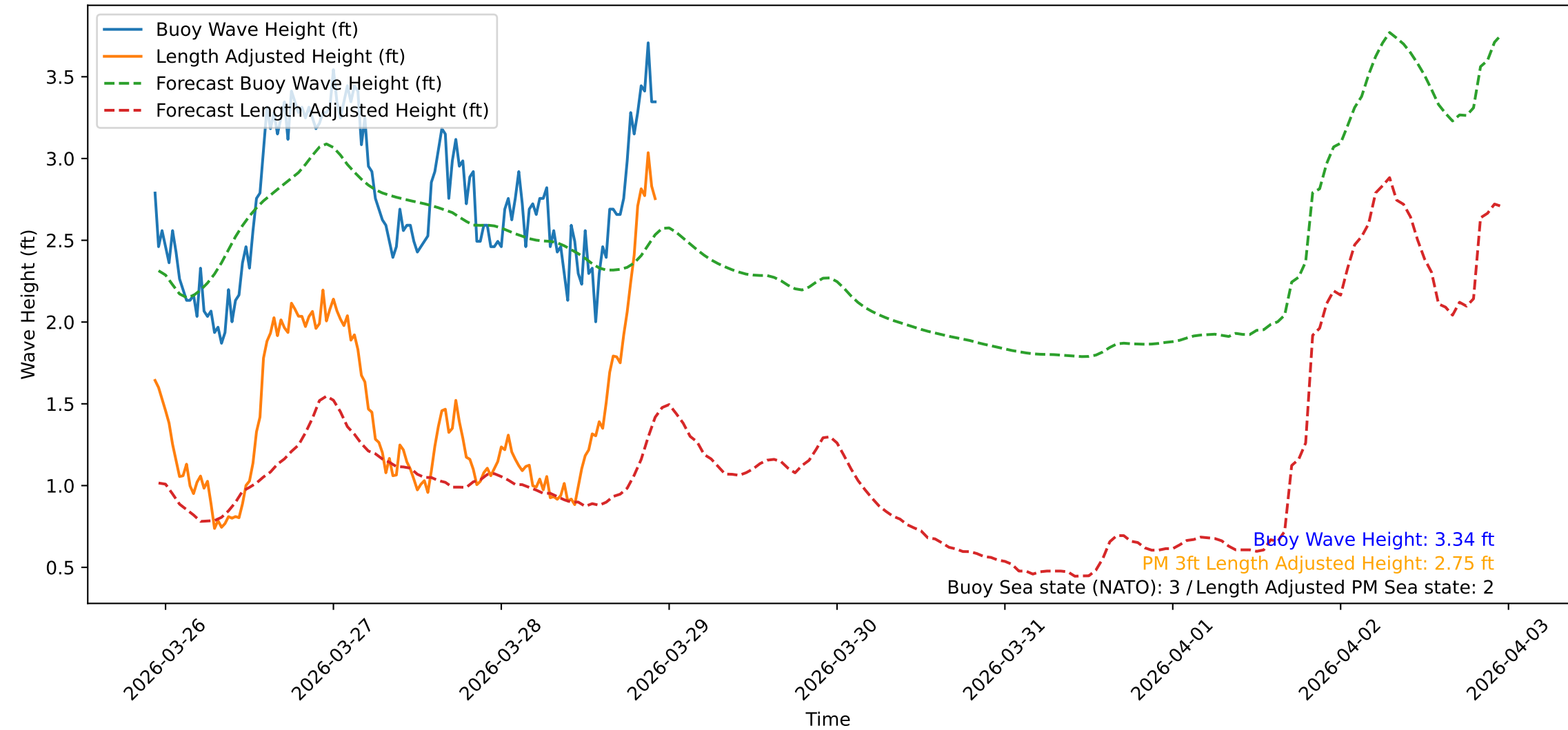
Wave Heights over Time for Green Beach at 2026-03-28 22:41:10
