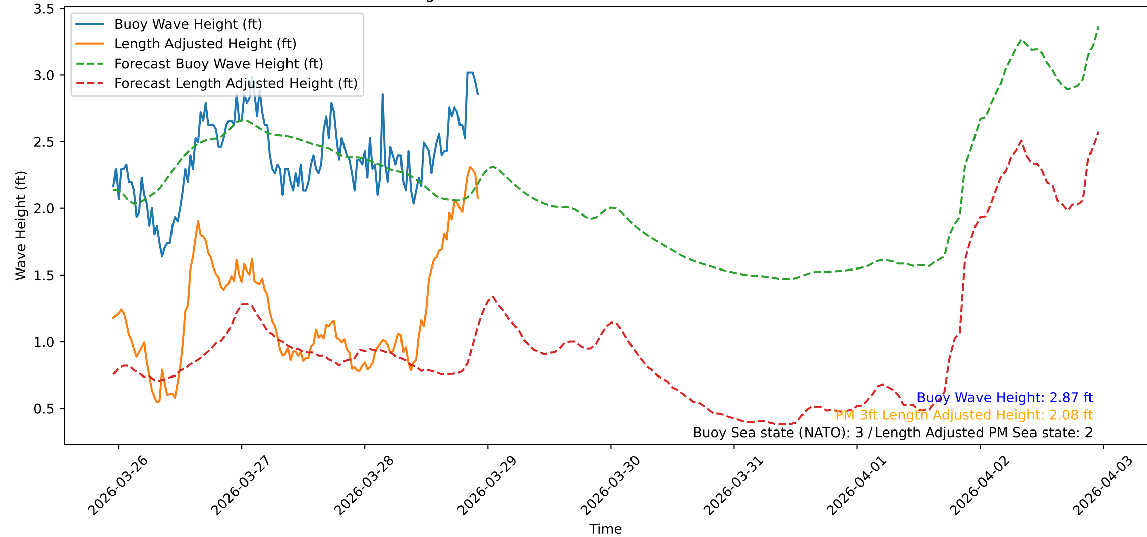
Wave Heights over Time for Red Beach at 2026-03-28 22:40:47
