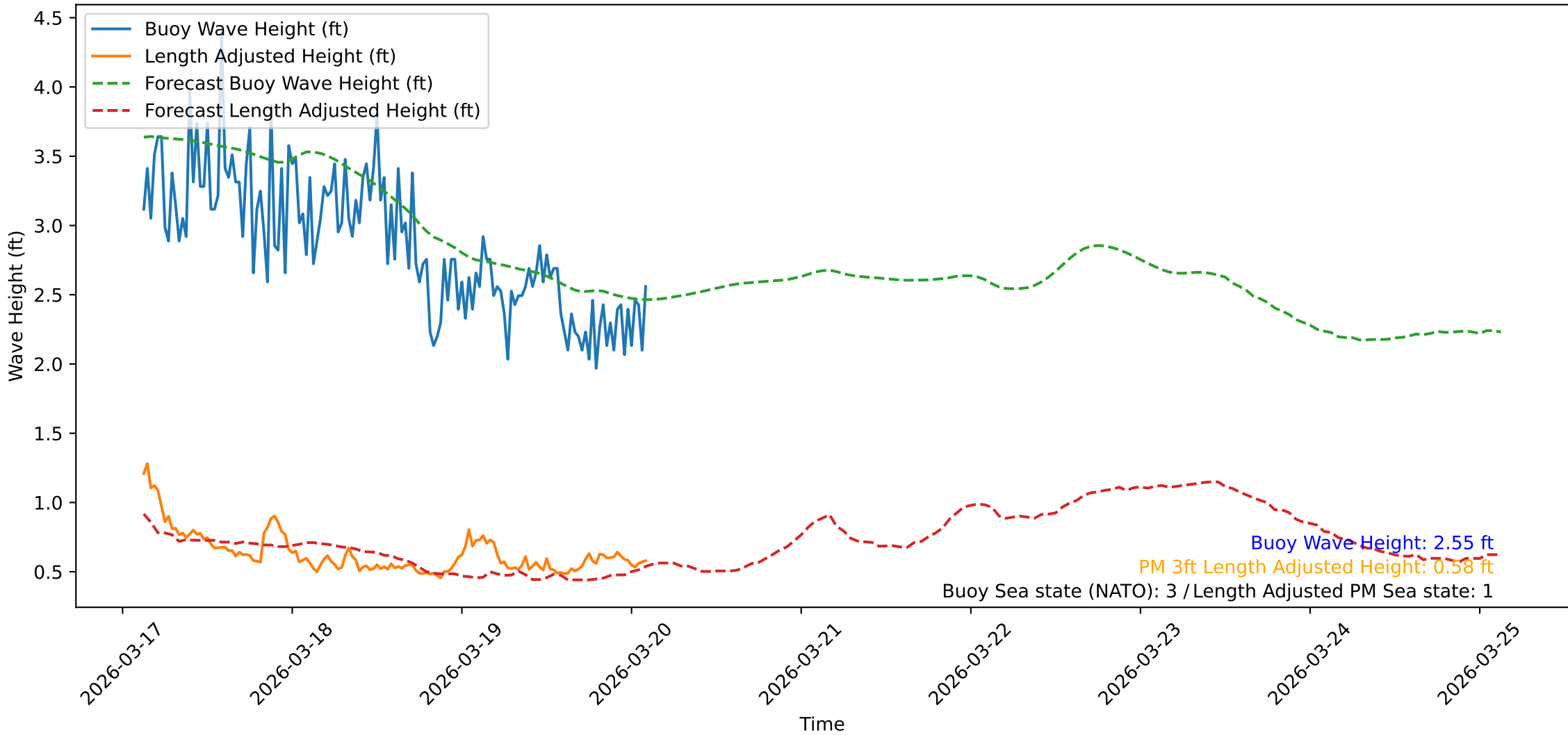
Wave Heights over Time for Oceanside Harbor at 2026-03-20 02:50:31
