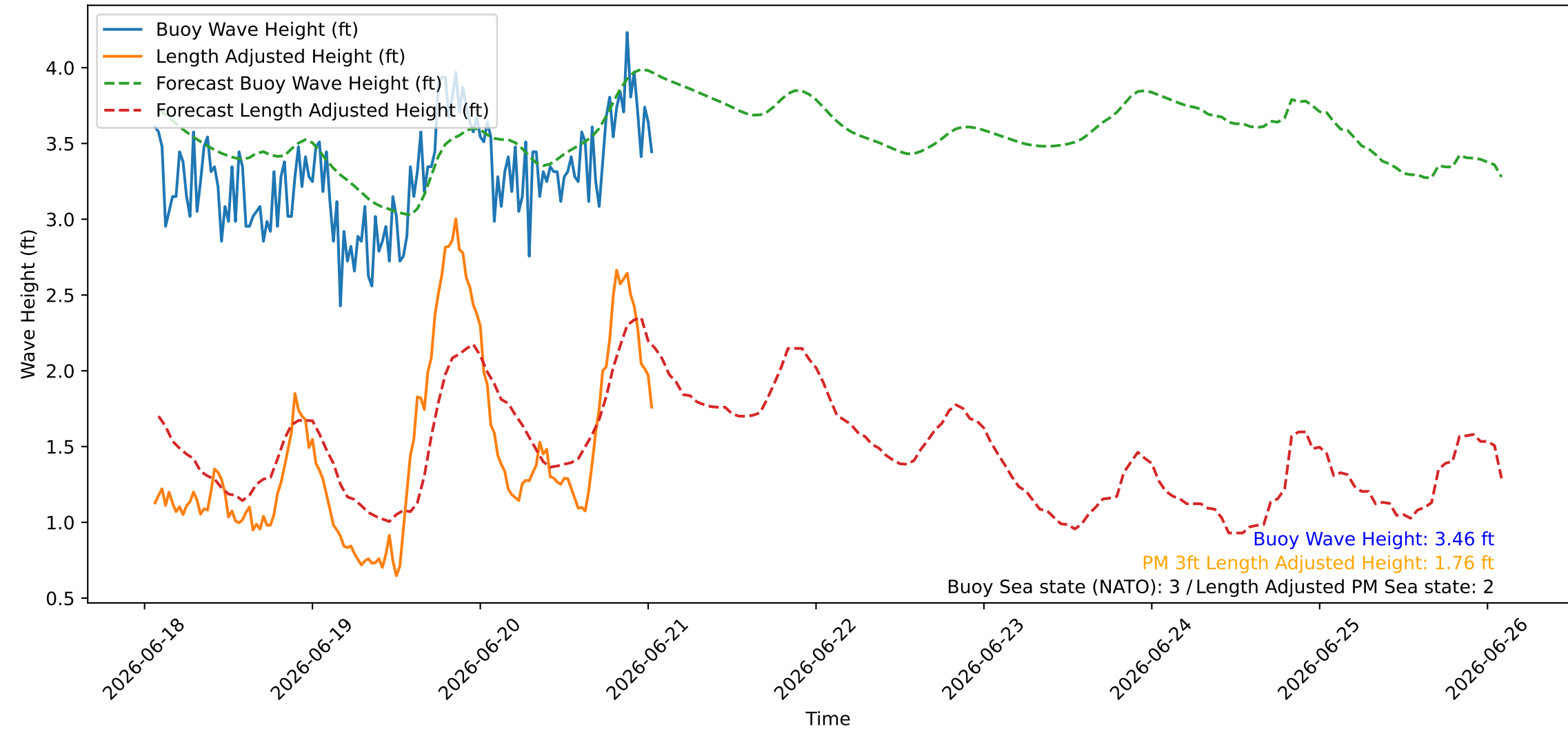
Wave Heights over Time for Green Beach at 2026-06-21 01:31:08
