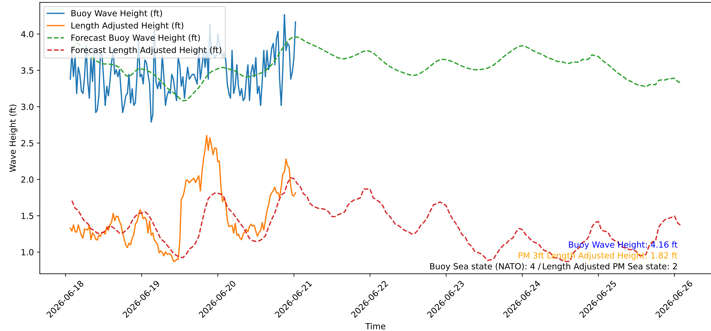
Wave Heights over Time for Oceanside Harbor at 2026-06-21 01:30:27
