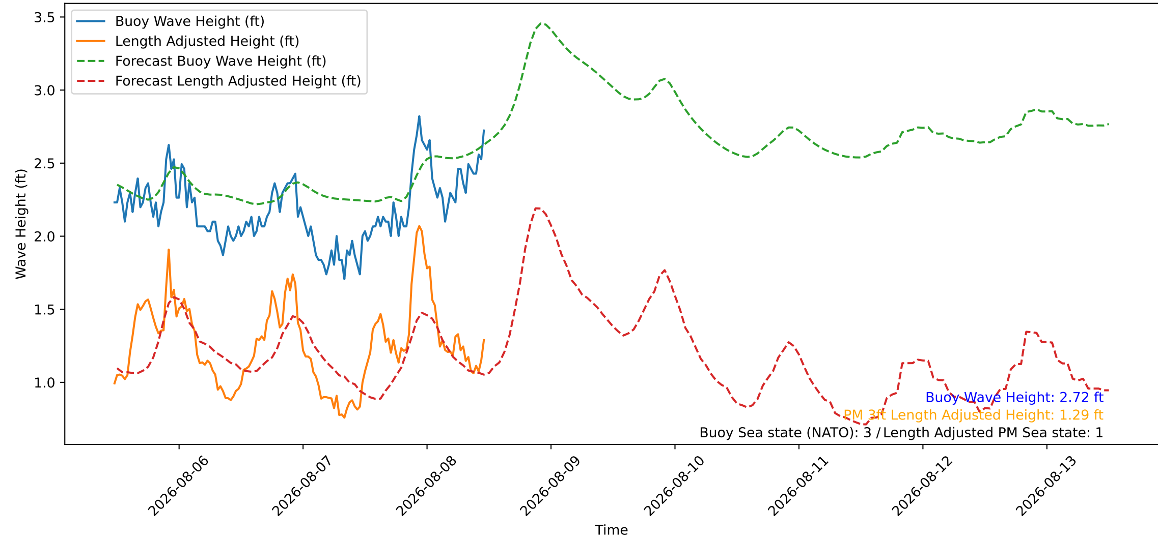
Wave Heights over Time for Green Beach at 2026-08-08 11:41:09
