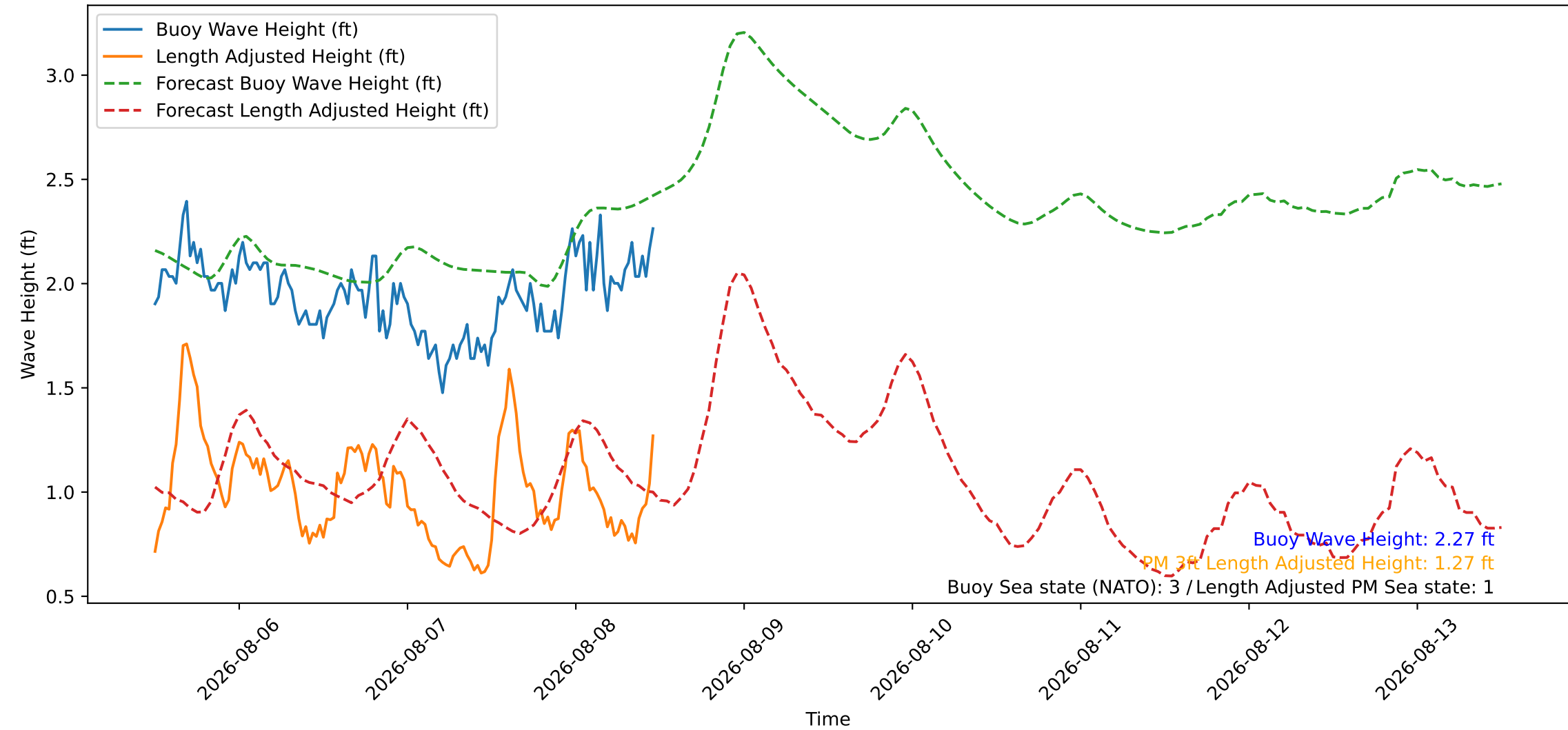
Wave Heights over Time for Red Beach at 2026-08-08 11:40:46
