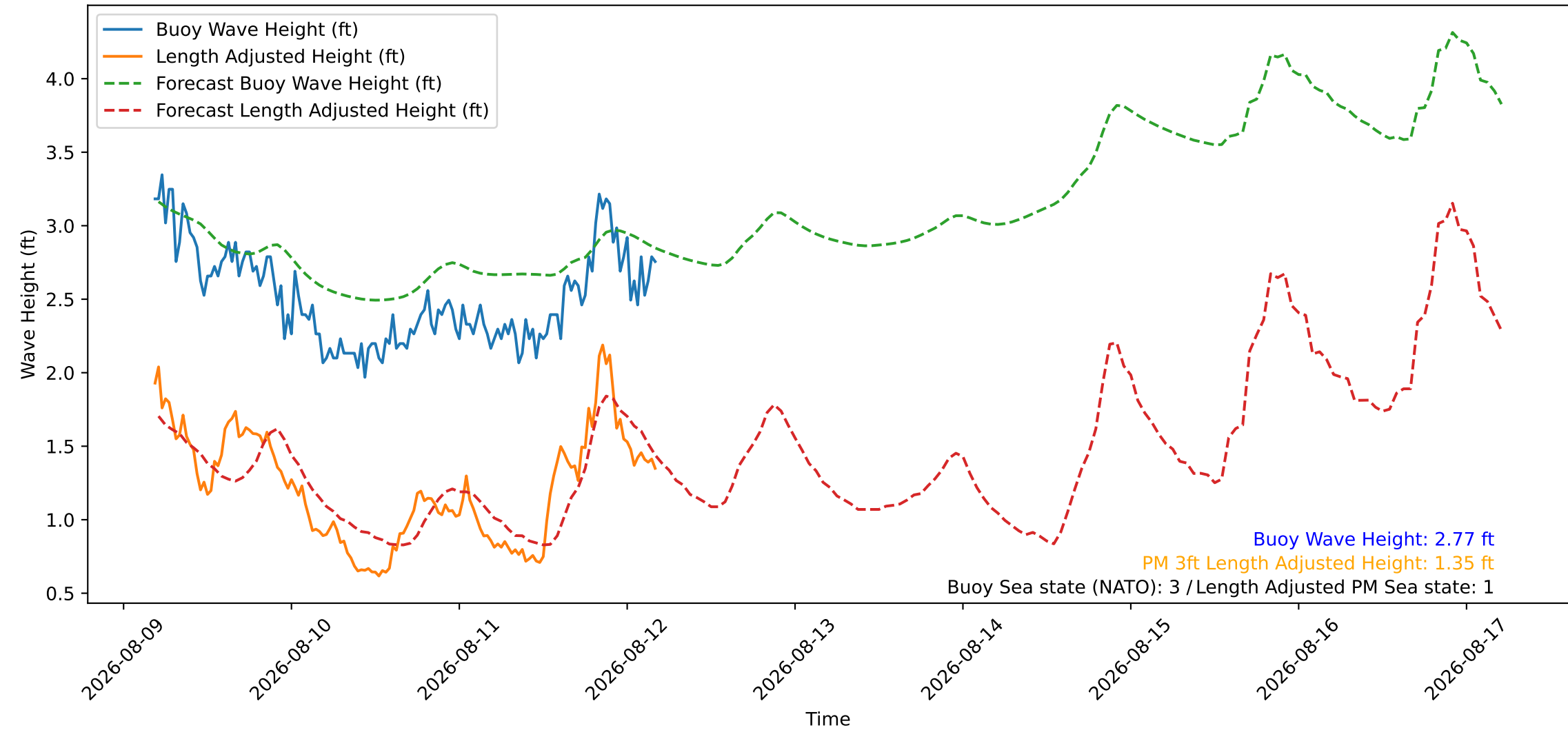
Wave Heights over Time for Green Beach at 2026-08-12 04:41:09
