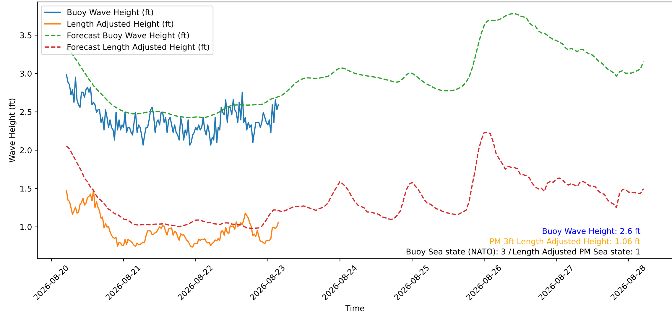
Wave Heights over Time for Red Beach at 2026-08-23 04:30:49
