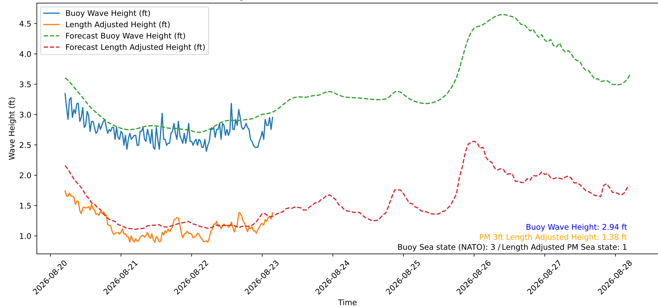
Wave Heights over Time for Green Beach at 2026-08-23 04:31:12
