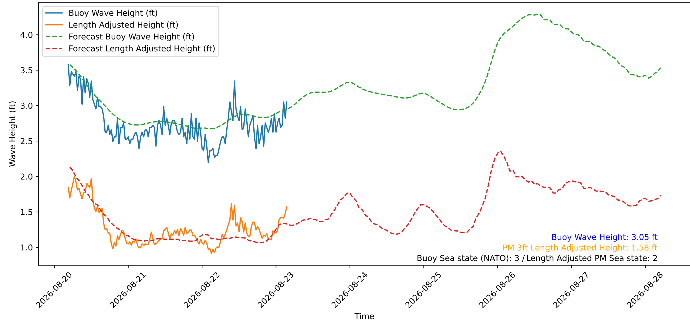
Wave Heights over Time for Oceanside Harbor at 2026-08-23 04:30:30
