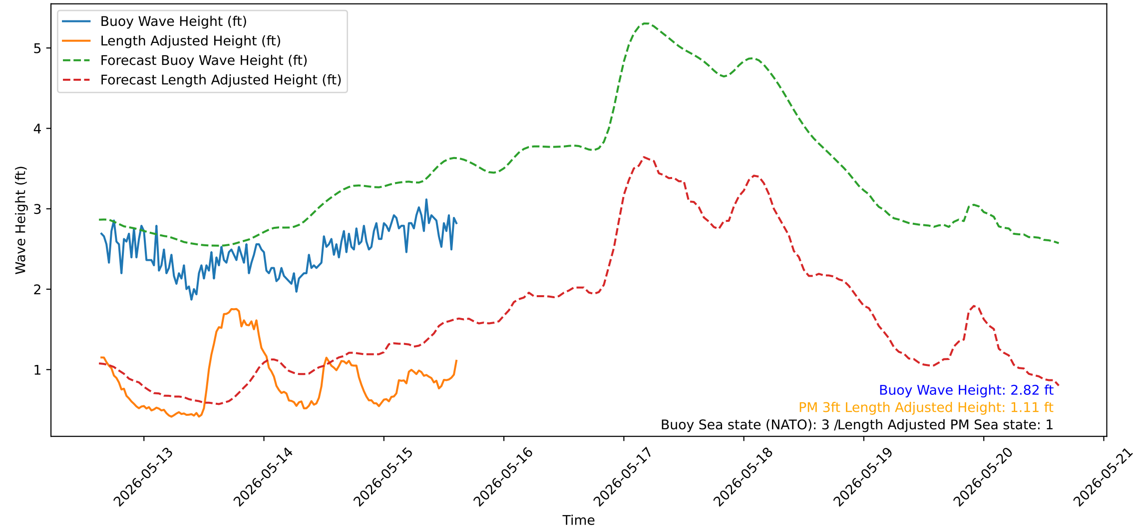
Wave Heights over Time for Red Beach at 2026-05-15 15:10:51
