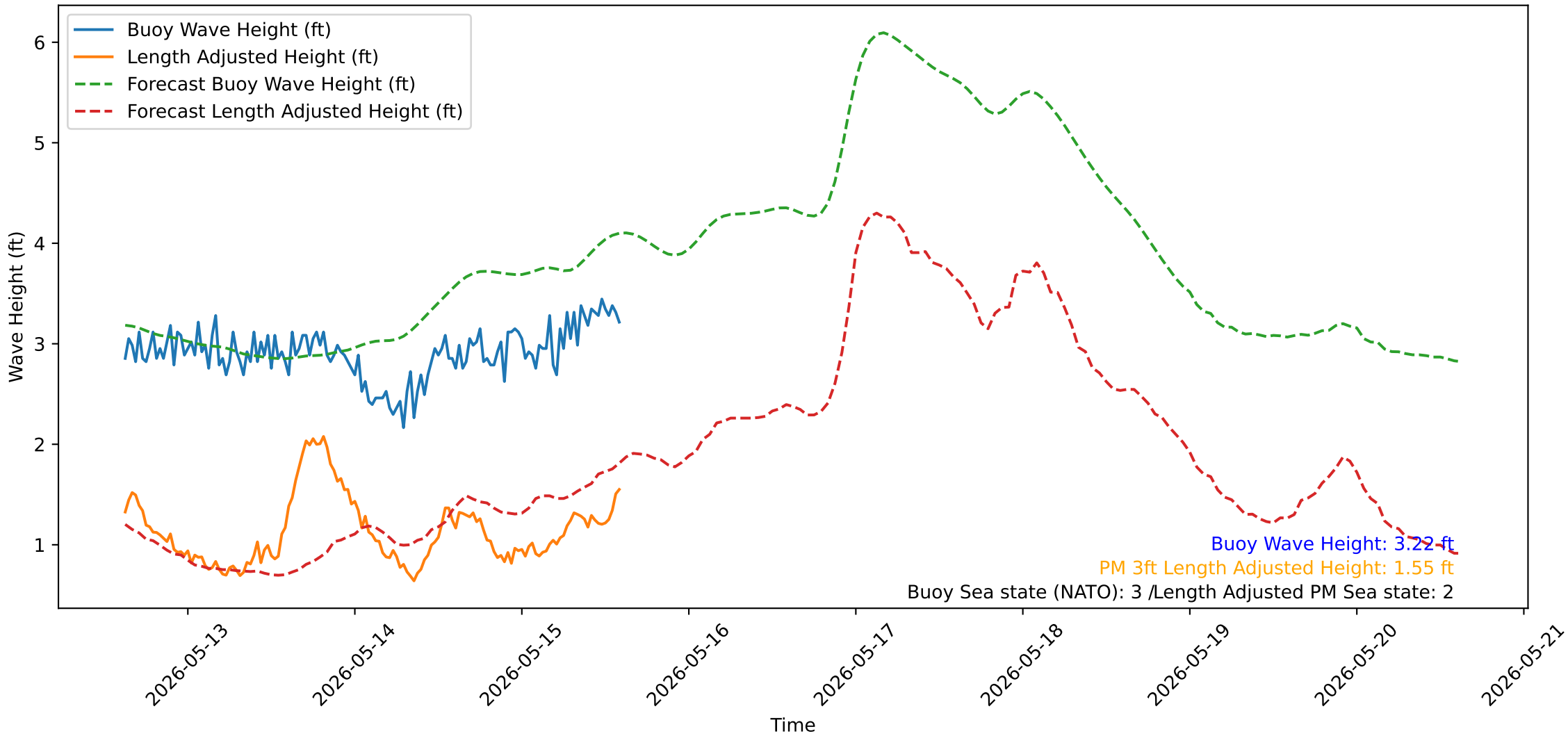
Wave Heights over Time for Oceanside Harbor at 2026-05-15 15:10:32
