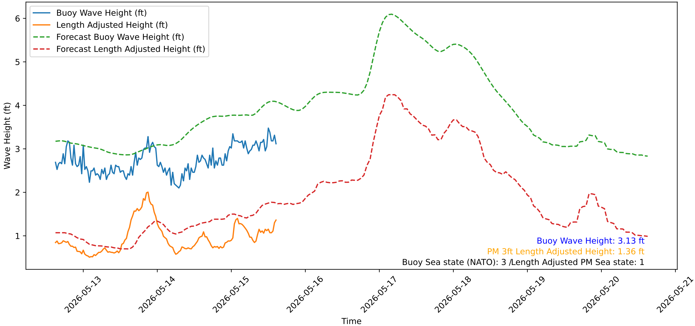
Wave Heights over Time for Green Beach at 2026-05-15 15:11:14
