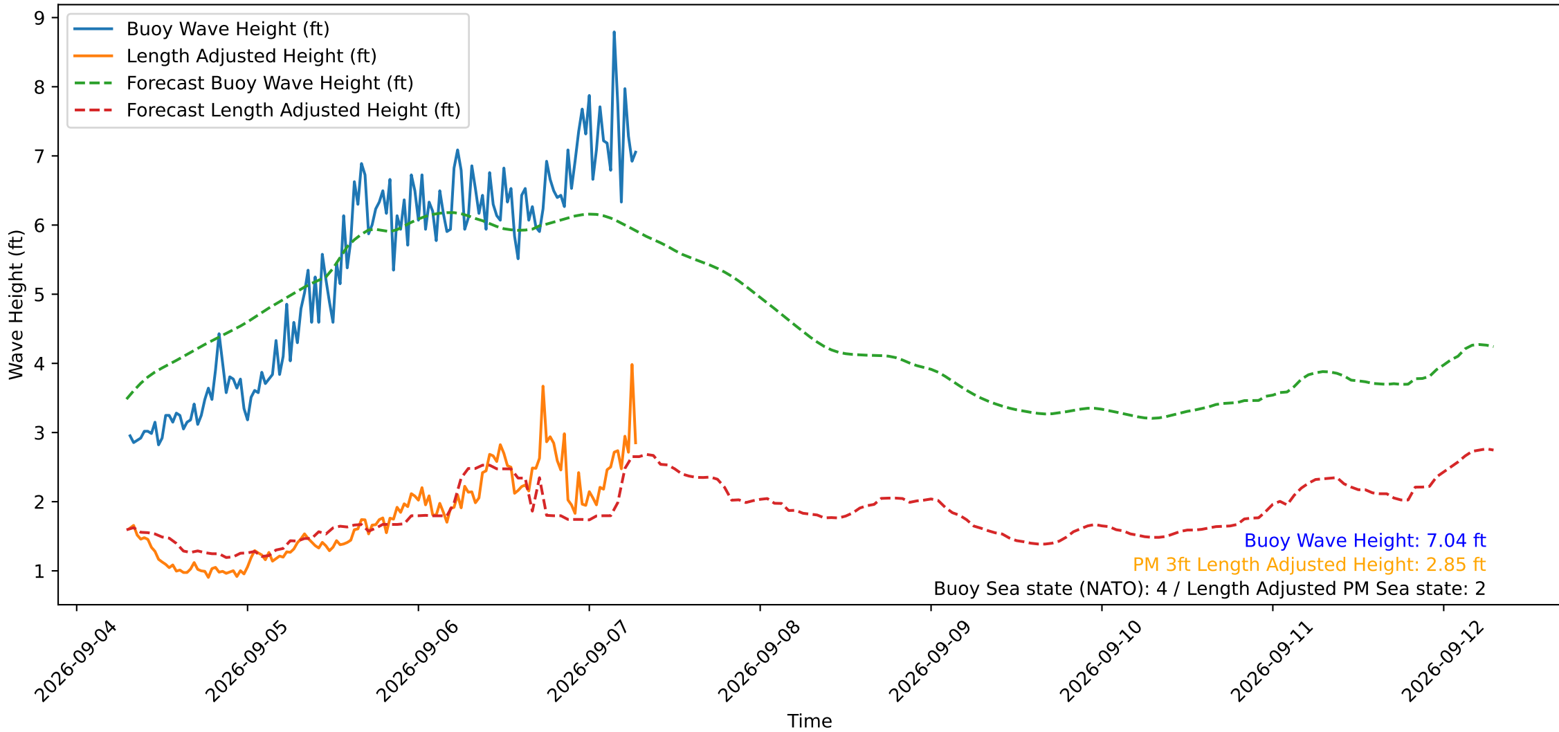
Wave Heights over Time for Green Beach at 2026-09-07 07:21:15
