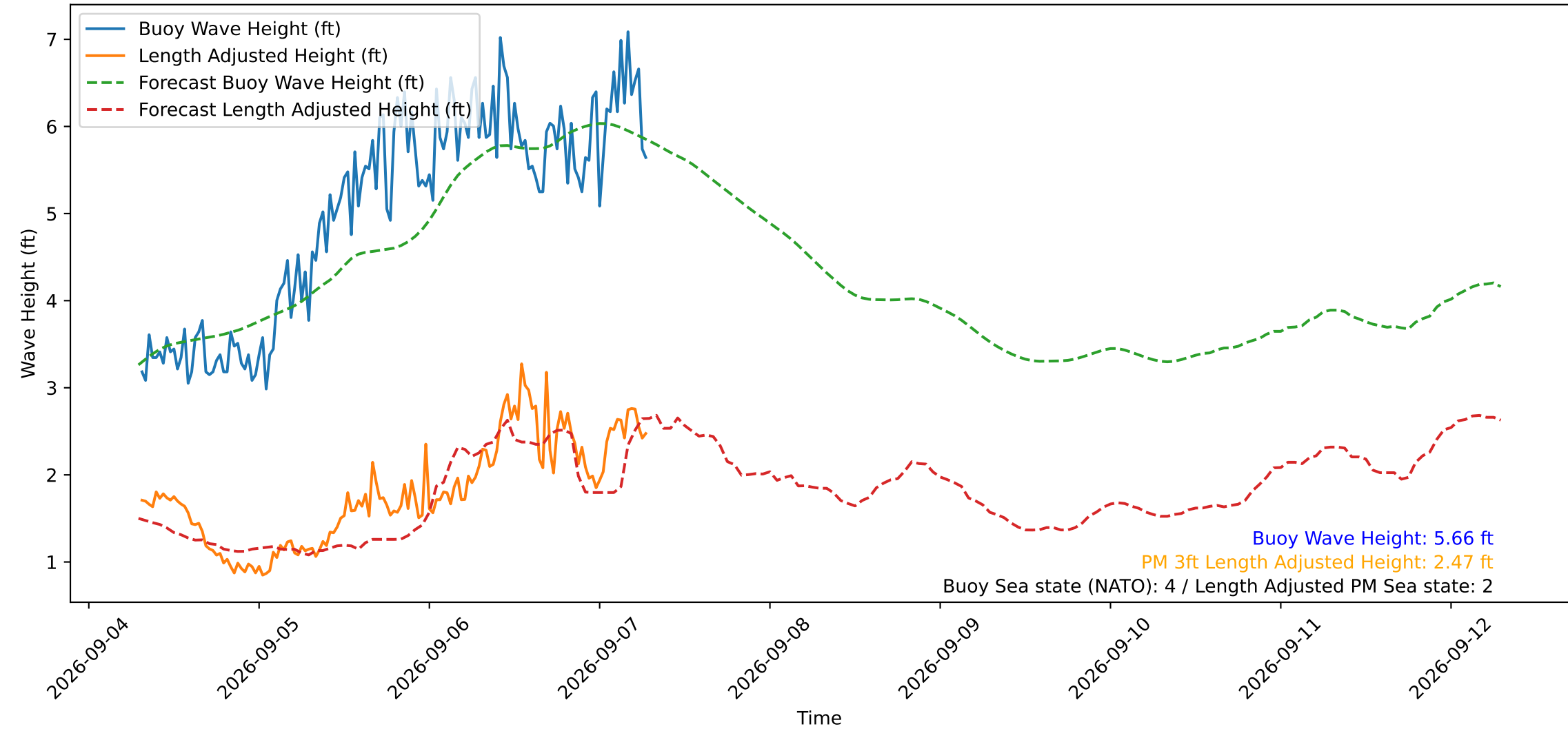
Wave Heights over Time for Oceanside Harbor at 2026-09-07 07:20:30
