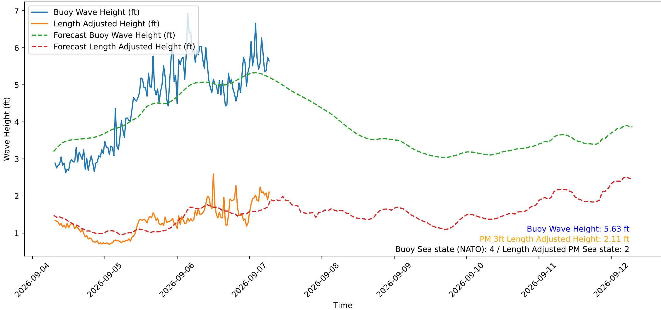
Wave Heights over Time for Red Beach at 2026-09-07 07:20:51
