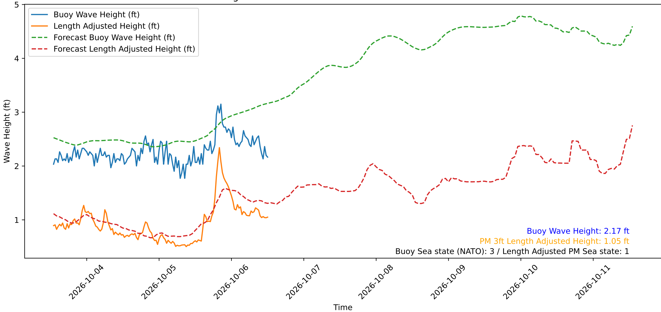
Wave Heights over Time for Green Beach at 2026-10-06 12:51:15
