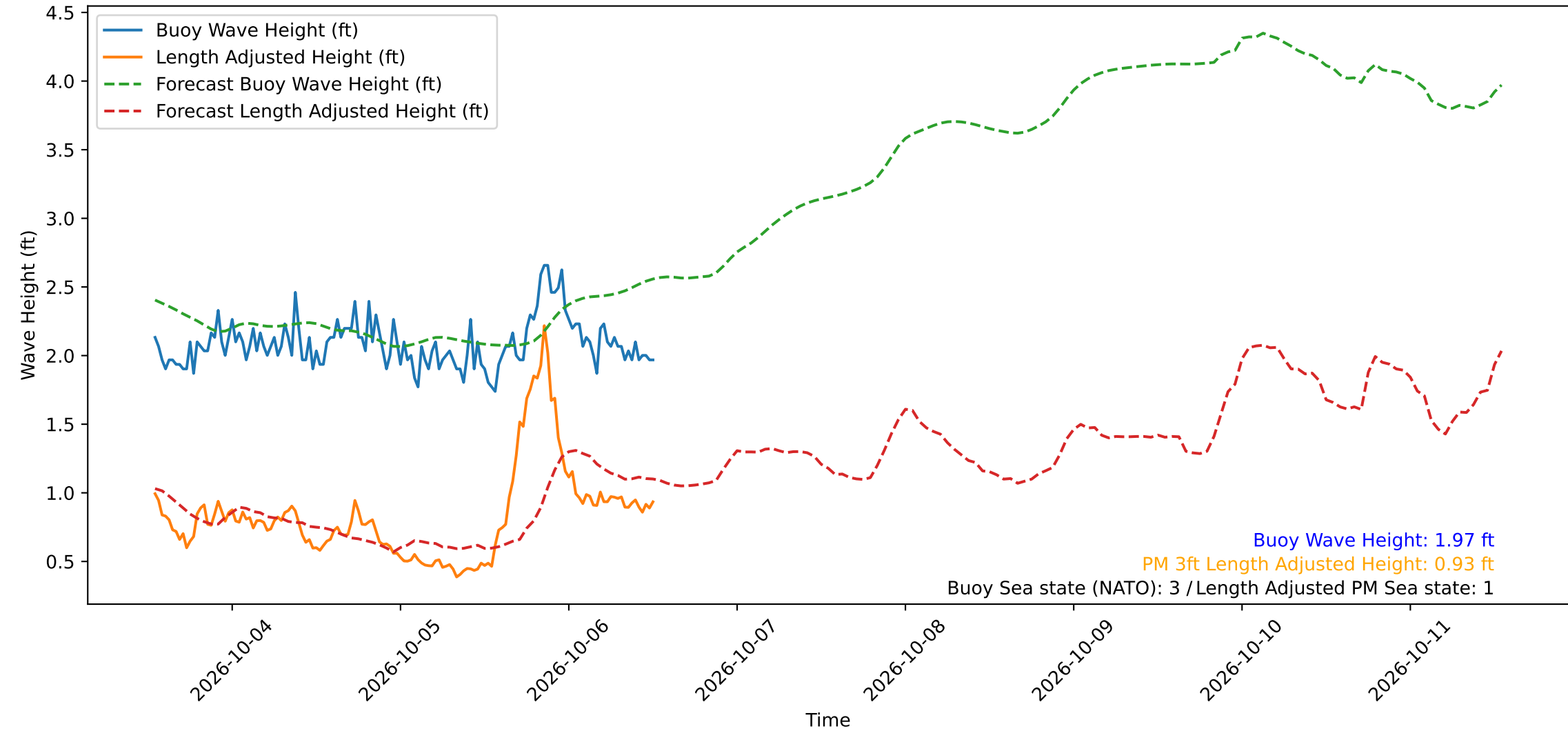
Wave Heights over Time for Red Beach at 2026-10-06 12:50:51
