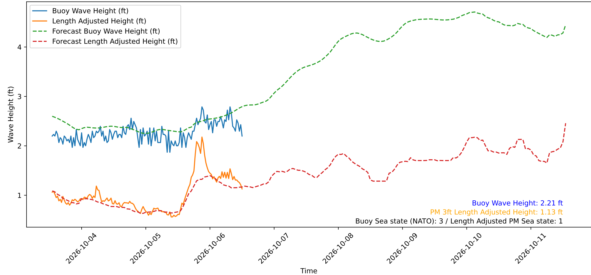
Wave Heights over Time for Oceanside Harbor at 2026-10-06 12:50:30
