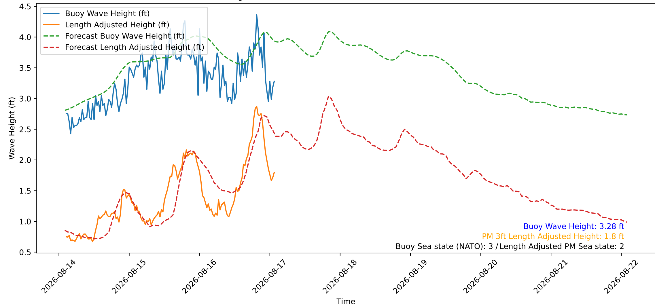
Wave Heights over Time for Green Beach at 2026-08-17 02:11:08
