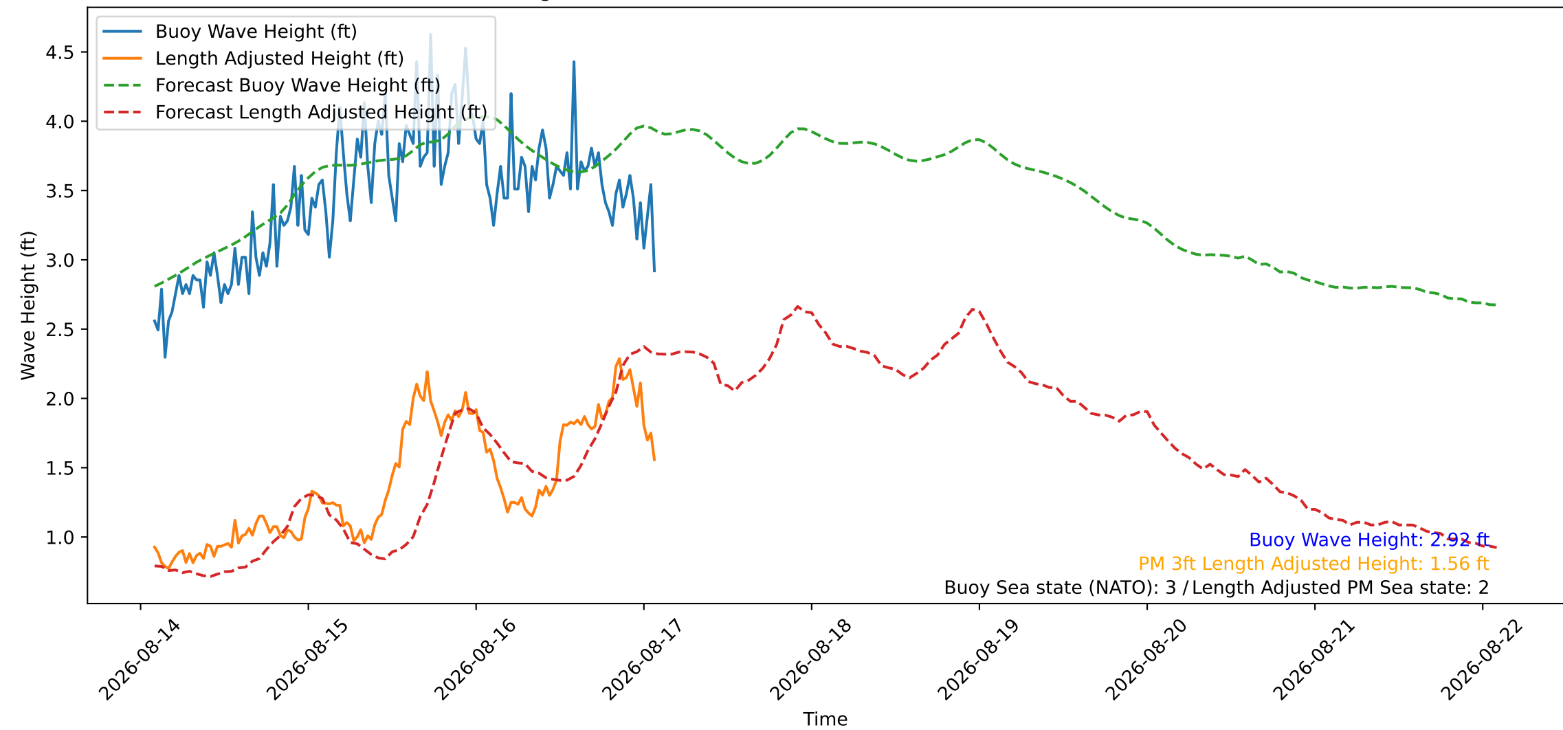
Wave Heights over Time for Oceanside Harbor at 2026-08-17 02:10:26
