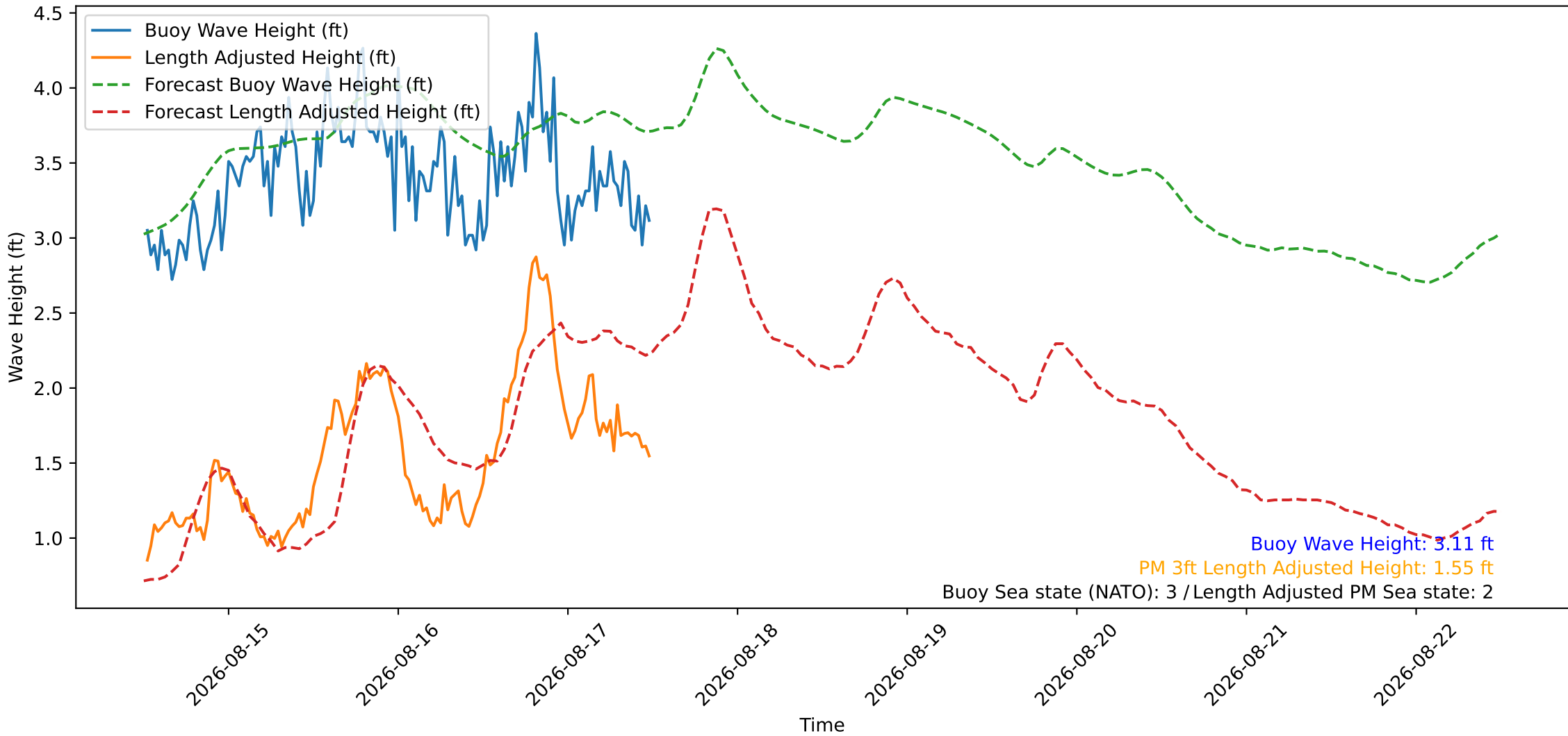
Wave Heights over Time for Green Beach at 2026-08-17 12:21:12
