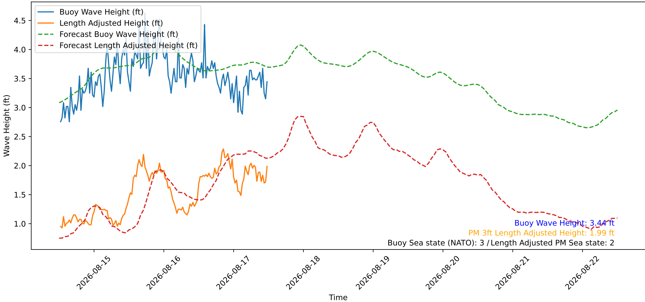
Wave Heights over Time for Oceanside Harbor at 2026-08-17 12:20:27
