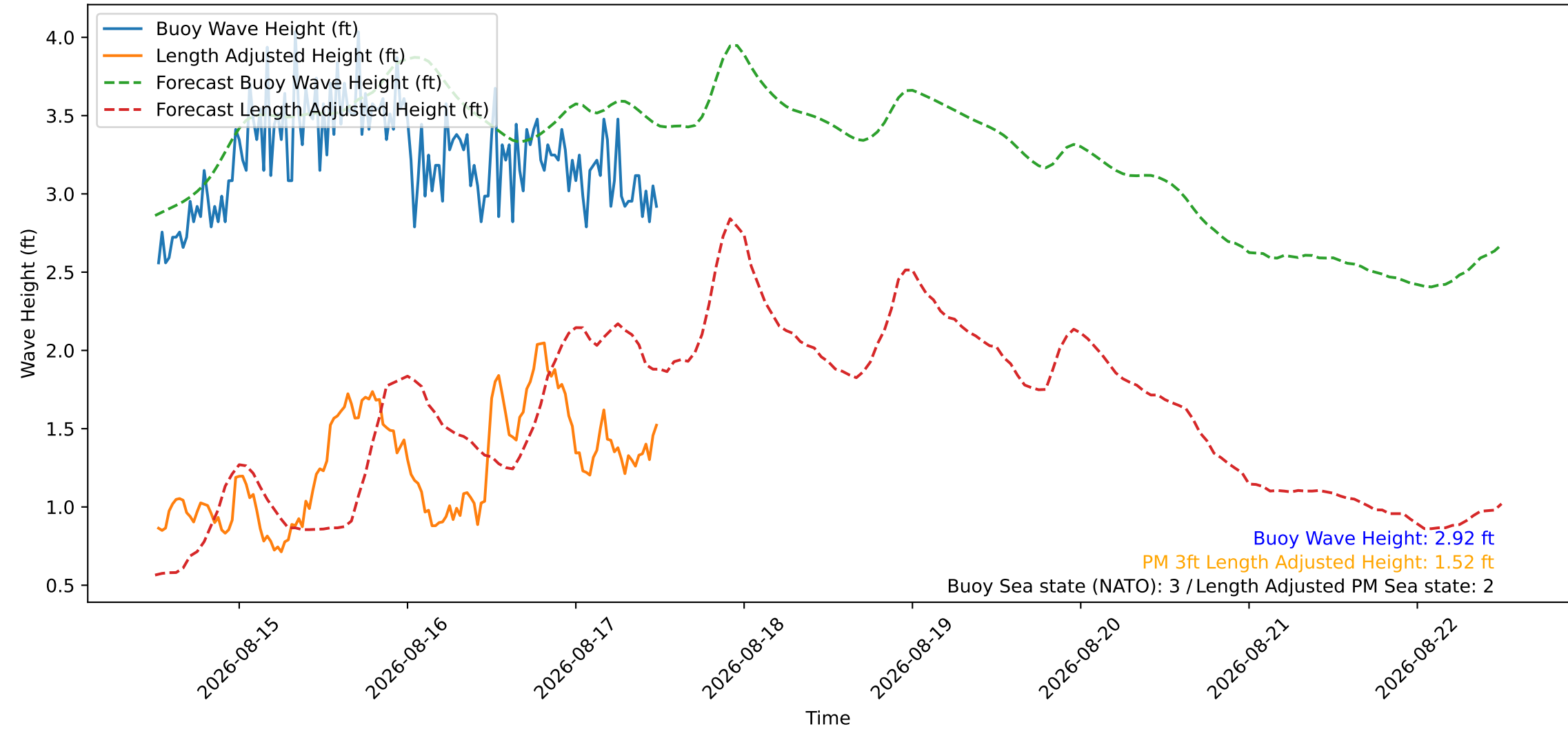
Wave Heights over Time for Red Beach at 2026-08-17 12:20:48
