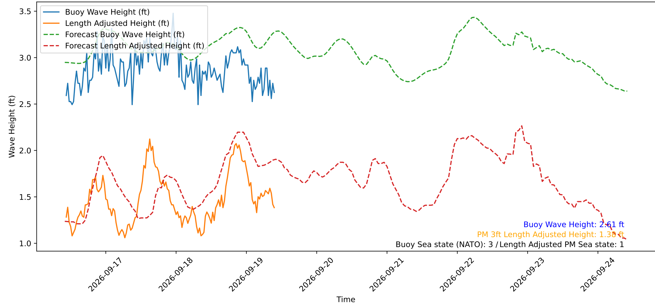
Wave Heights over Time for Green Beach at 2026-09-19 10:21:14
