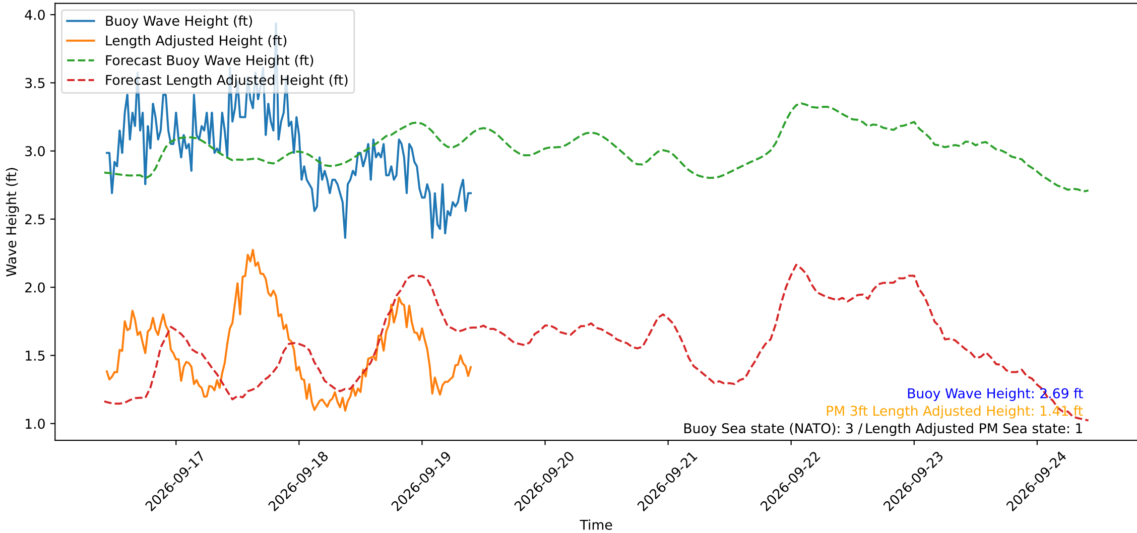
Wave Heights over Time for Oceanside Harbor at 2026-09-19 10:20:29
