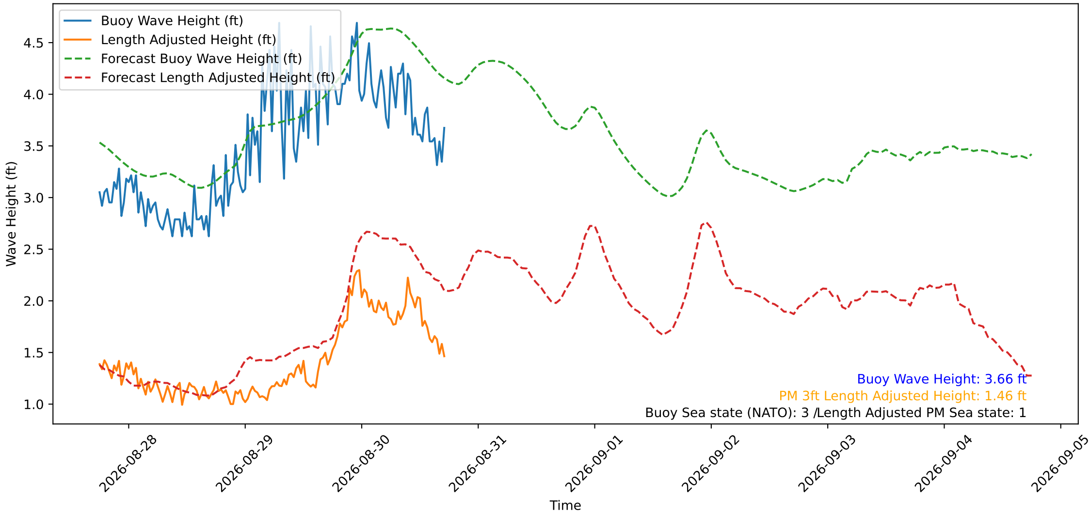
Wave Heights over Time for Red Beach at 2026-08-30 17:40:50
