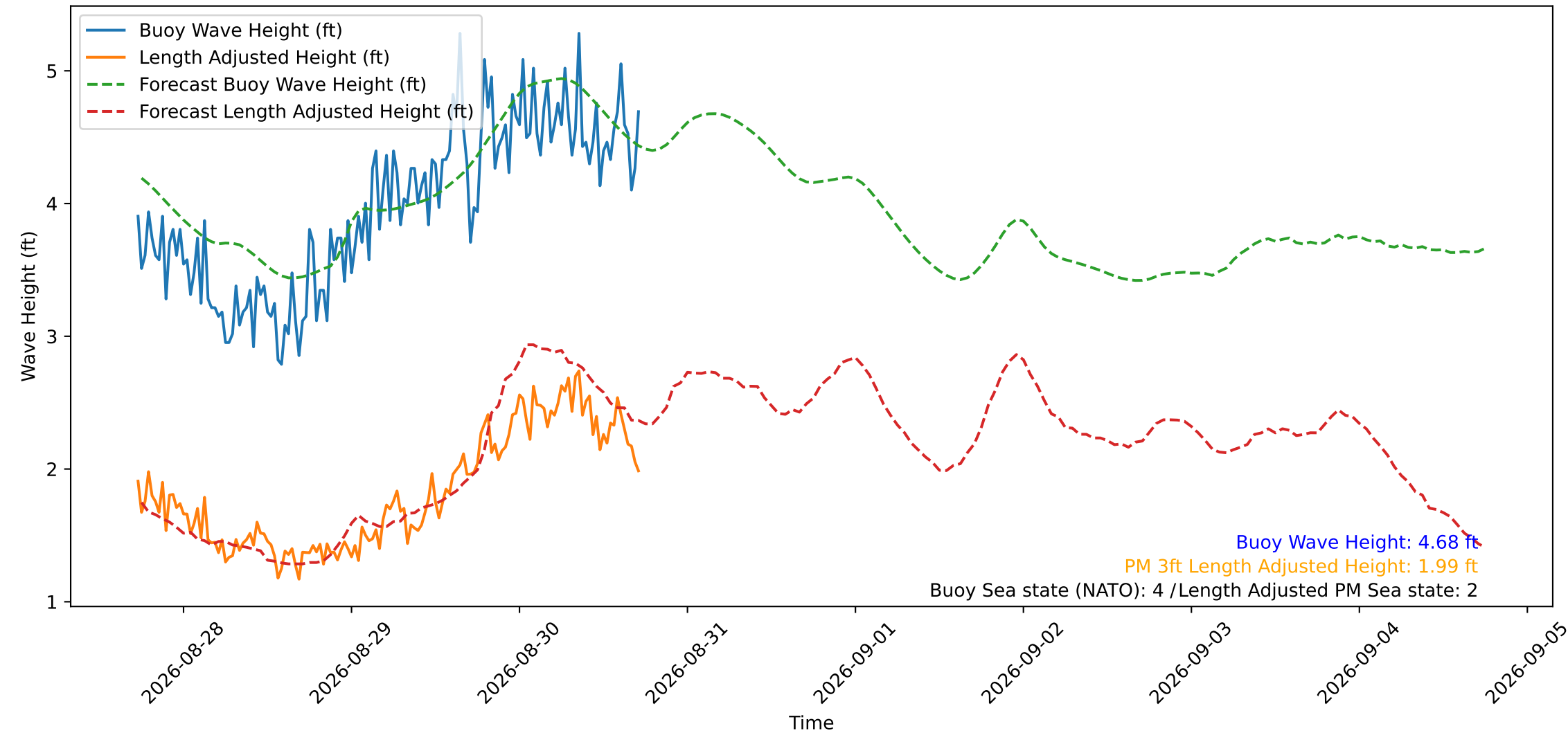
Wave Heights over Time for Oceanside Harbor at 2026-08-30 17:40:30
