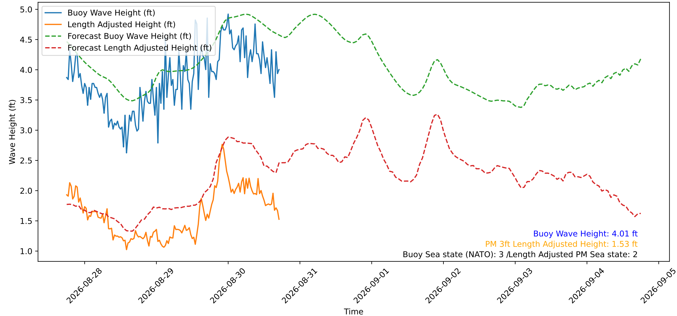
Wave Heights over Time for Green Beach at 2026-08-30 17:41:13
