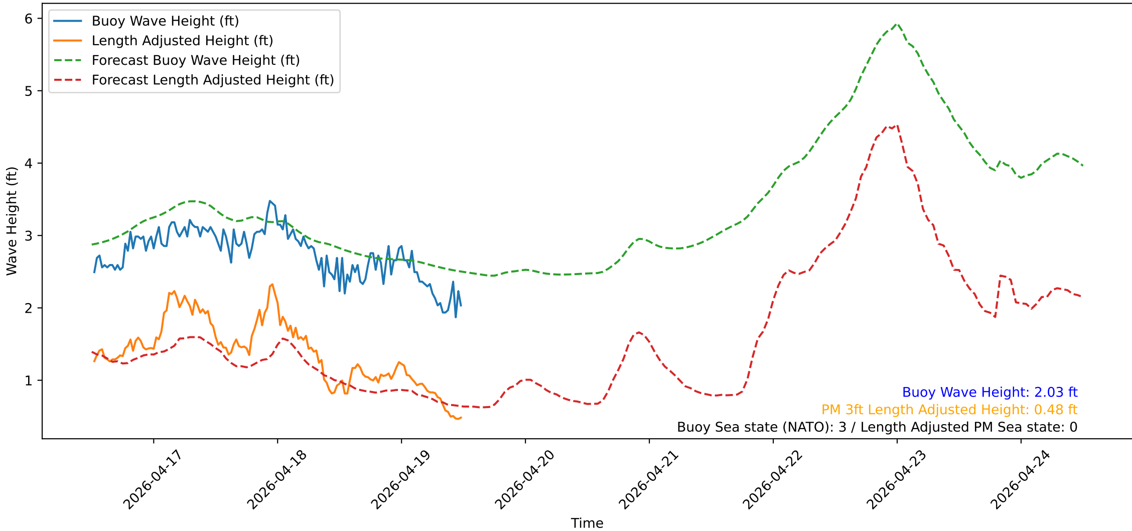
Wave Heights over Time for Green Beach at 2026-04-19 12:21:13
