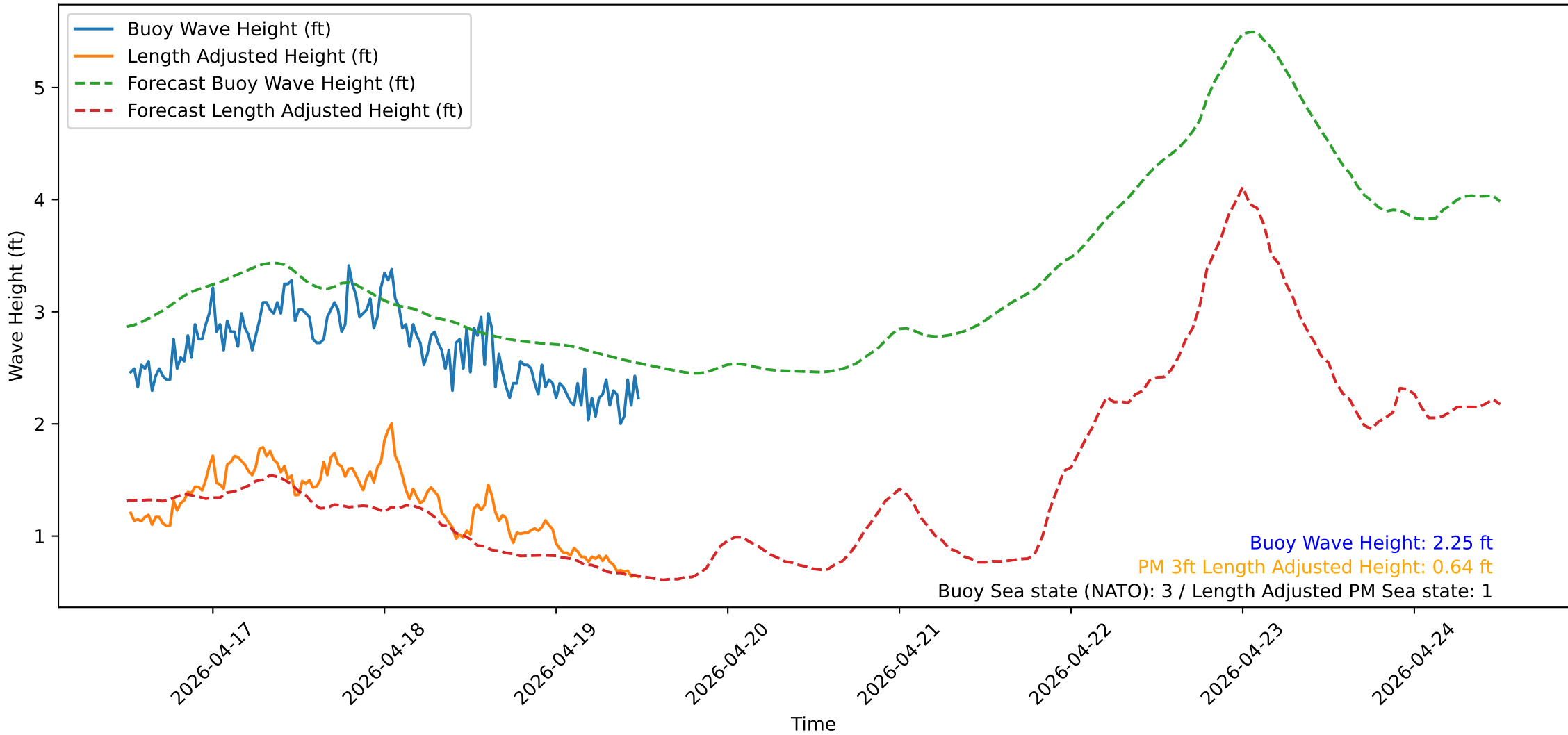
Wave Heights over Time for Oceanside Harbor at 2026-04-19 12:20:31
