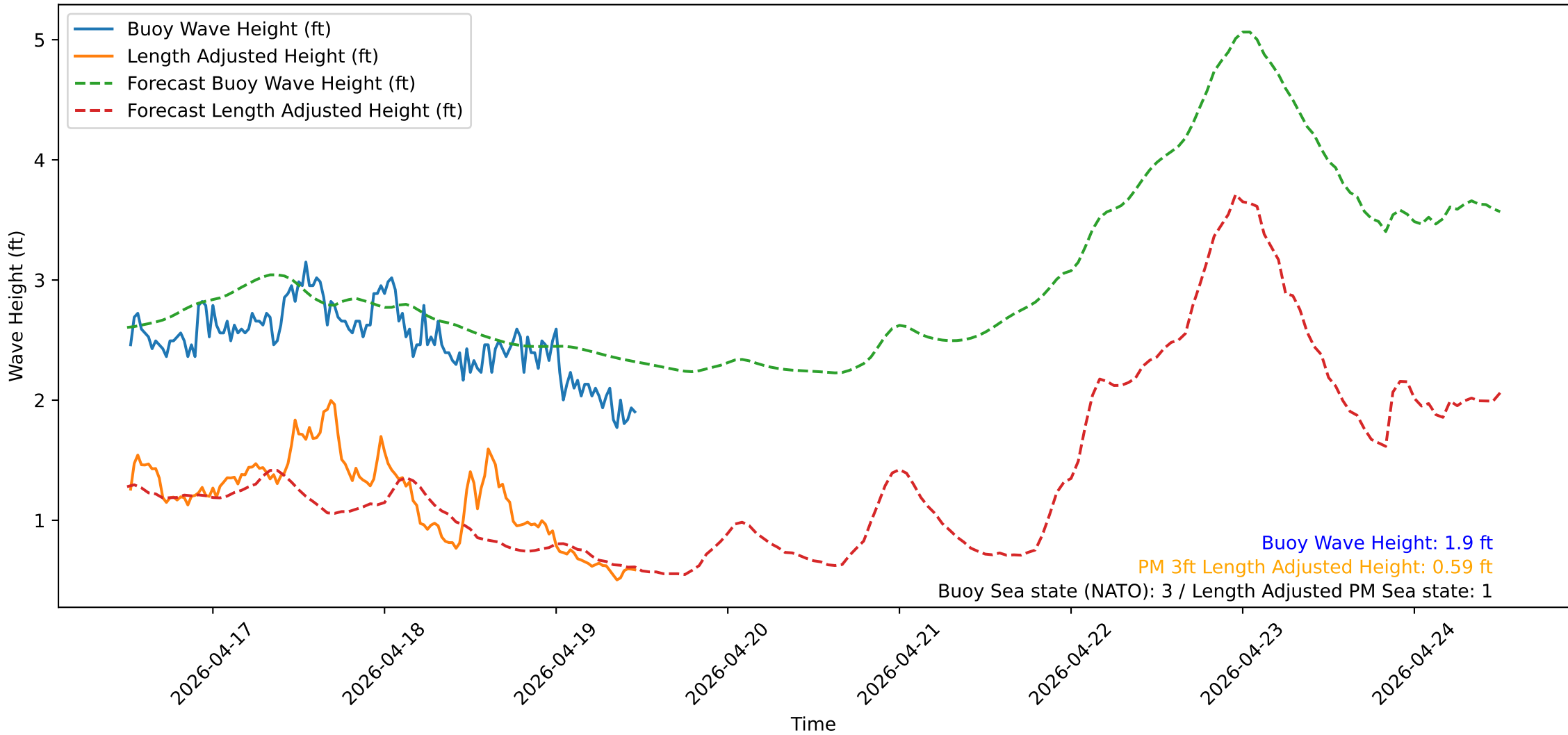
Wave Heights over Time for Red Beach at 2026-04-19 12:20:51
