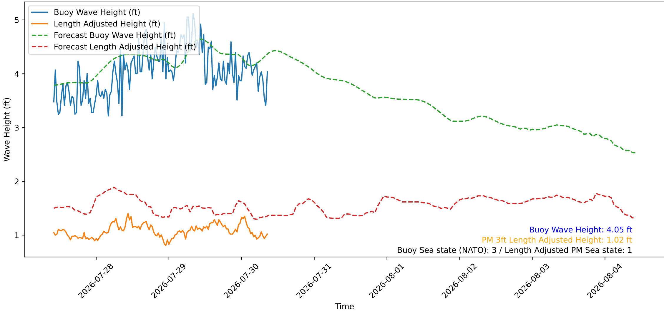
Wave Heights over Time for Red Beach at 2026-07-30 09:30:46
