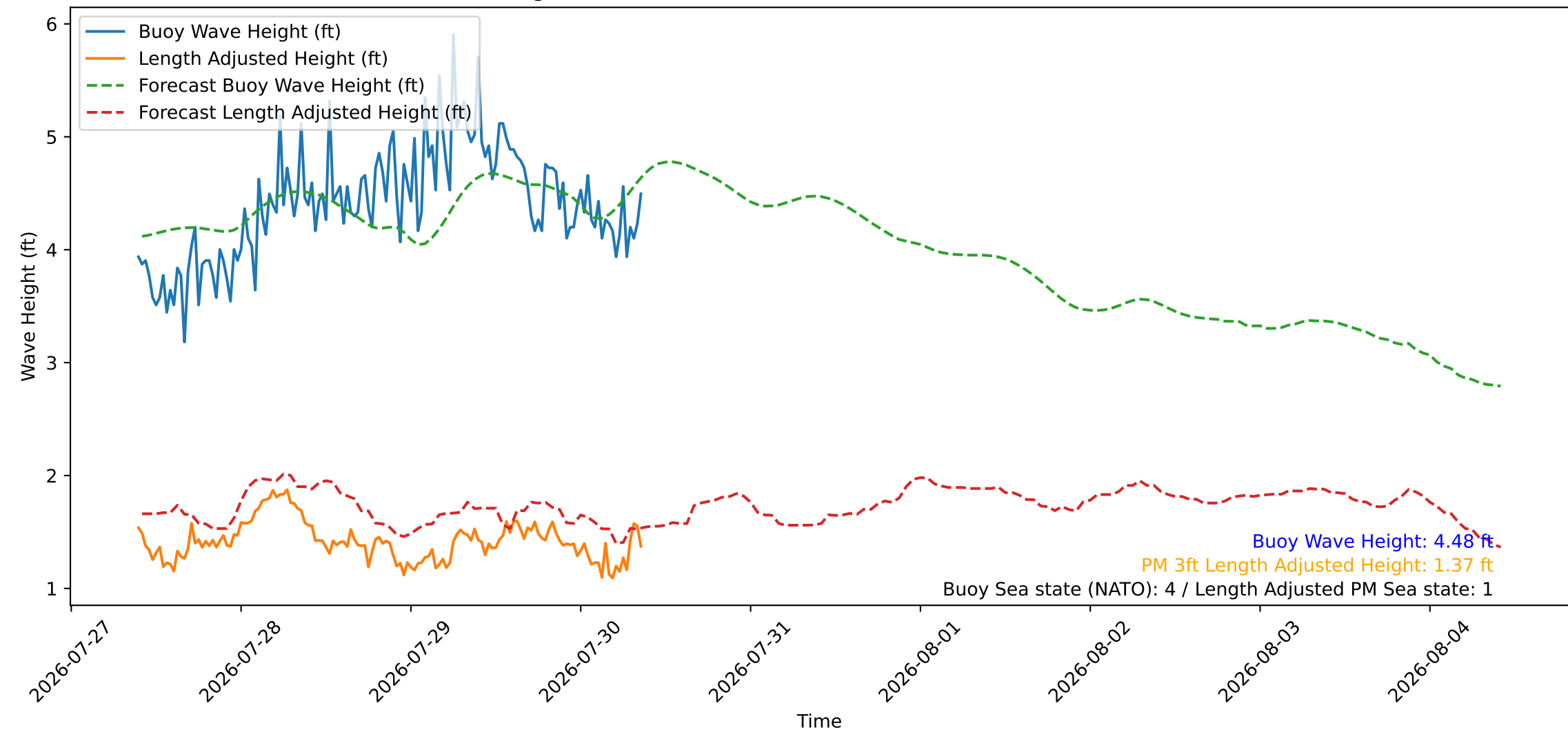
Wave Heights over Time for Oceanside Harbor at 2026-07-30 09:30:27
