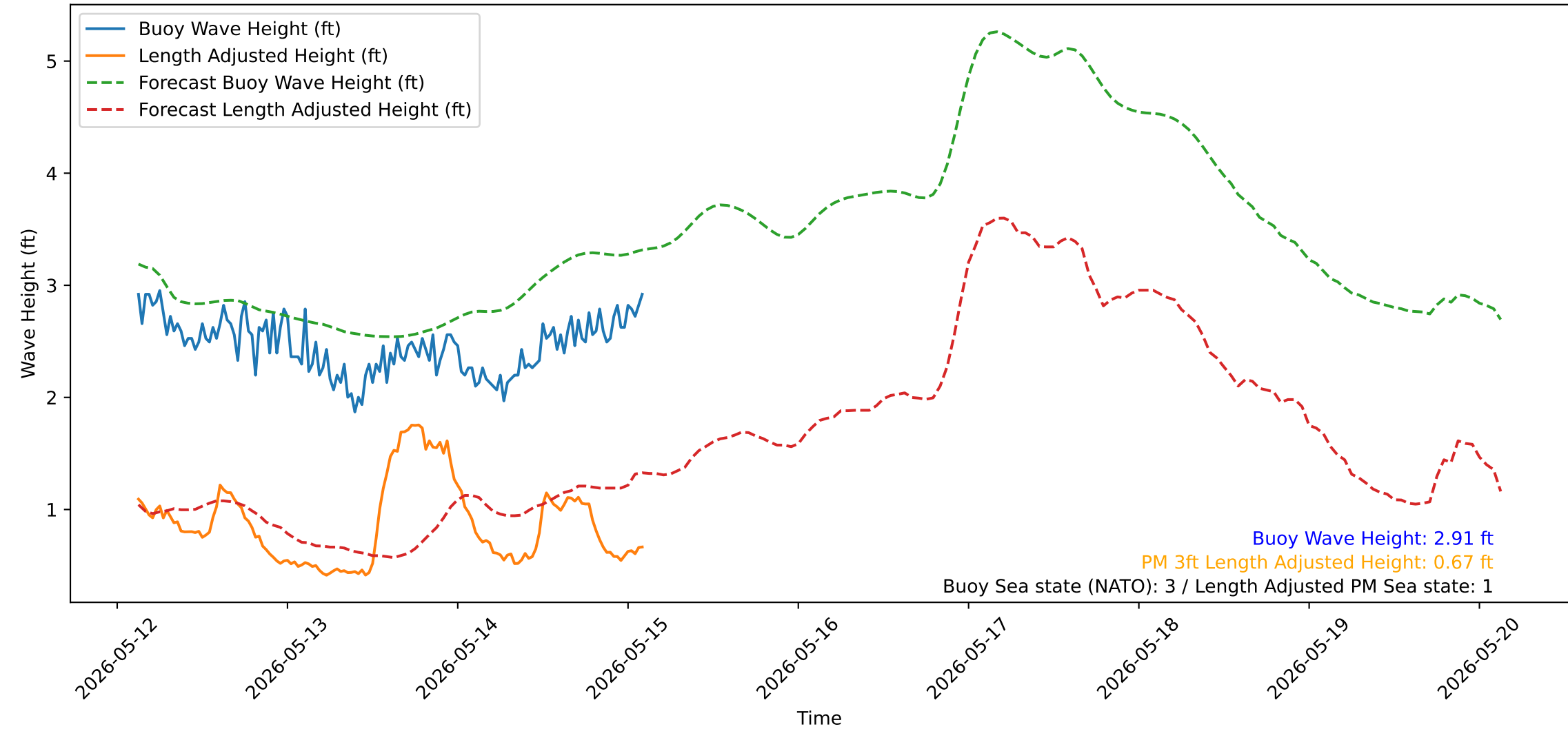
Wave Heights over Time for Red Beach at 2026-05-15 02:40:51
