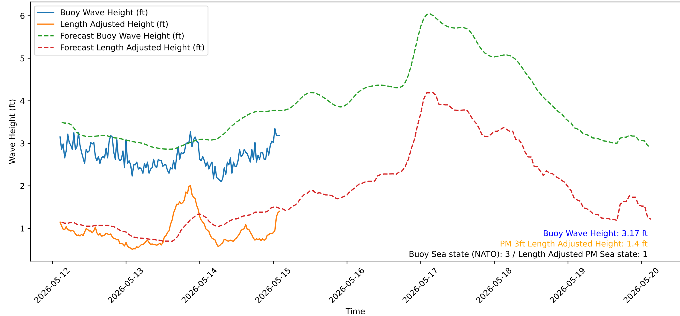
Wave Heights over Time for Green Beach at 2026-05-15 02:41:13
