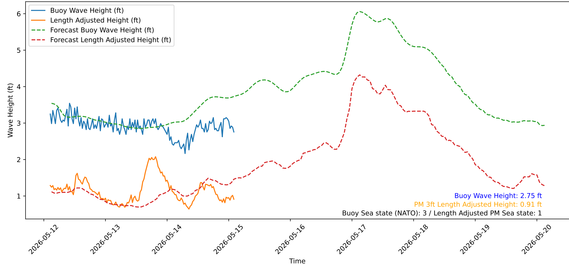
Wave Heights over Time for Oceanside Harbor at 2026-05-15 02:40:31
