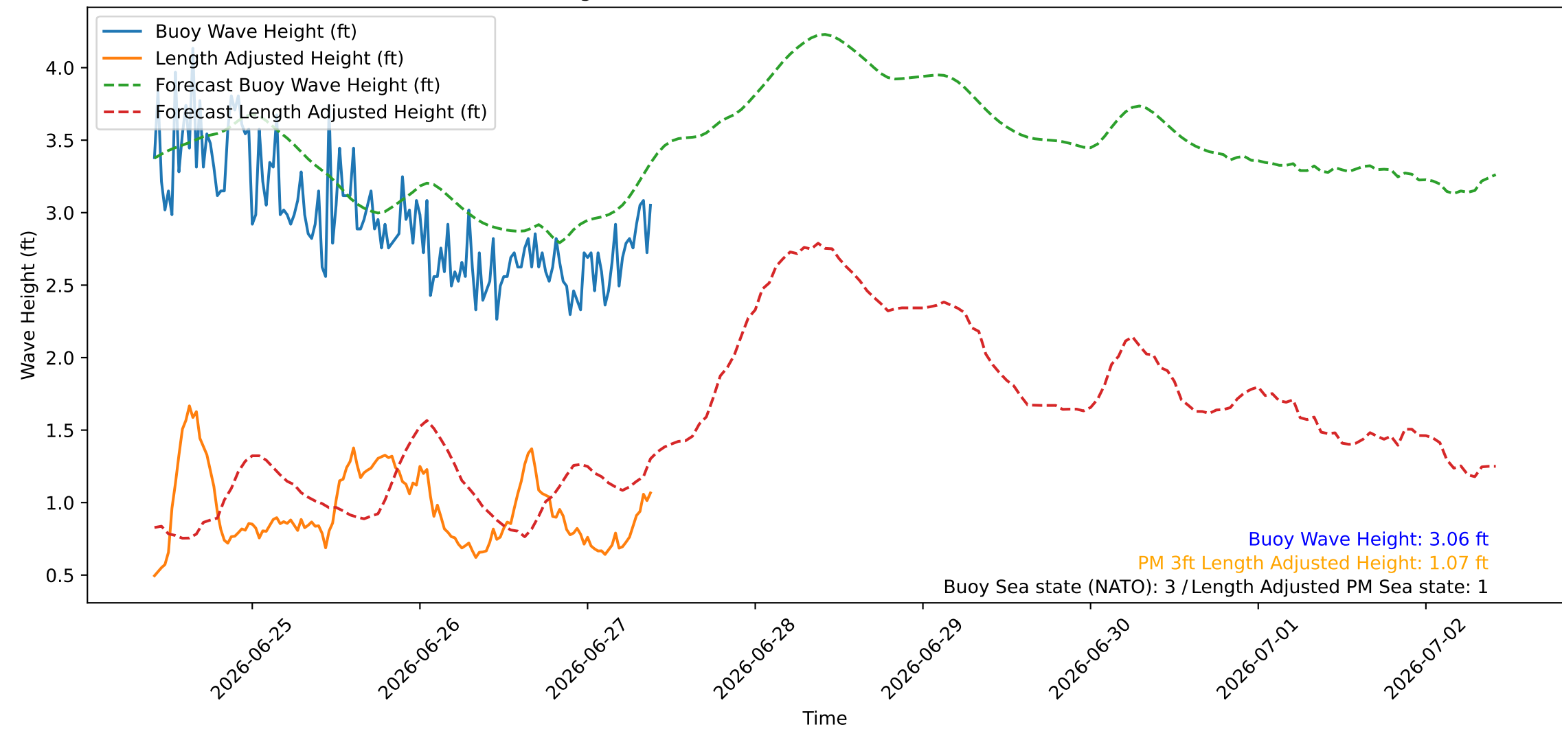
Wave Heights over Time for Red Beach at 2026-06-27 09:40:46
