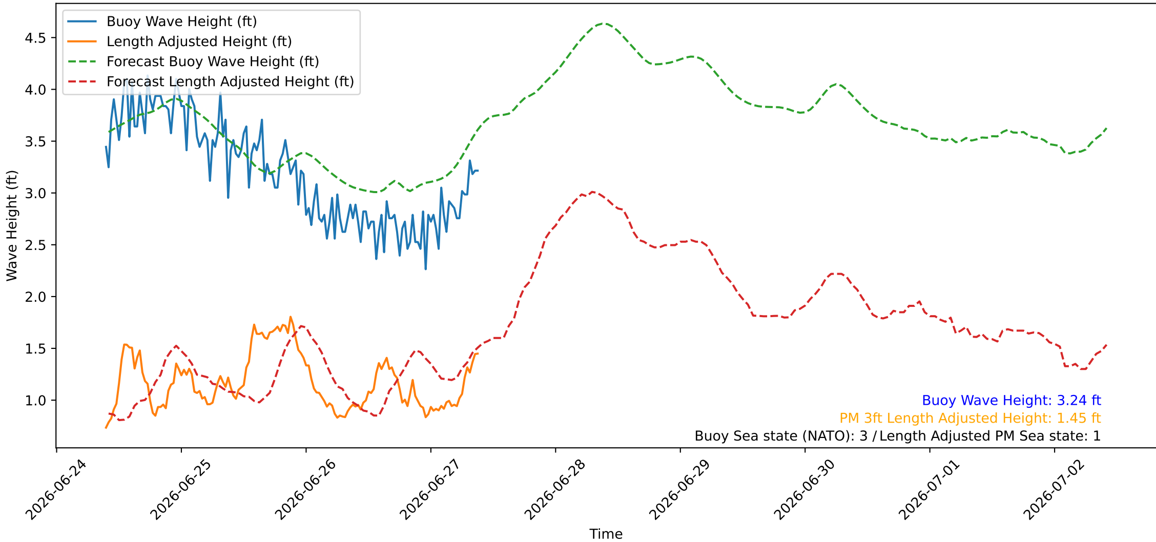
Wave Heights over Time for Green Beach at 2026-06-27 09:41:08
