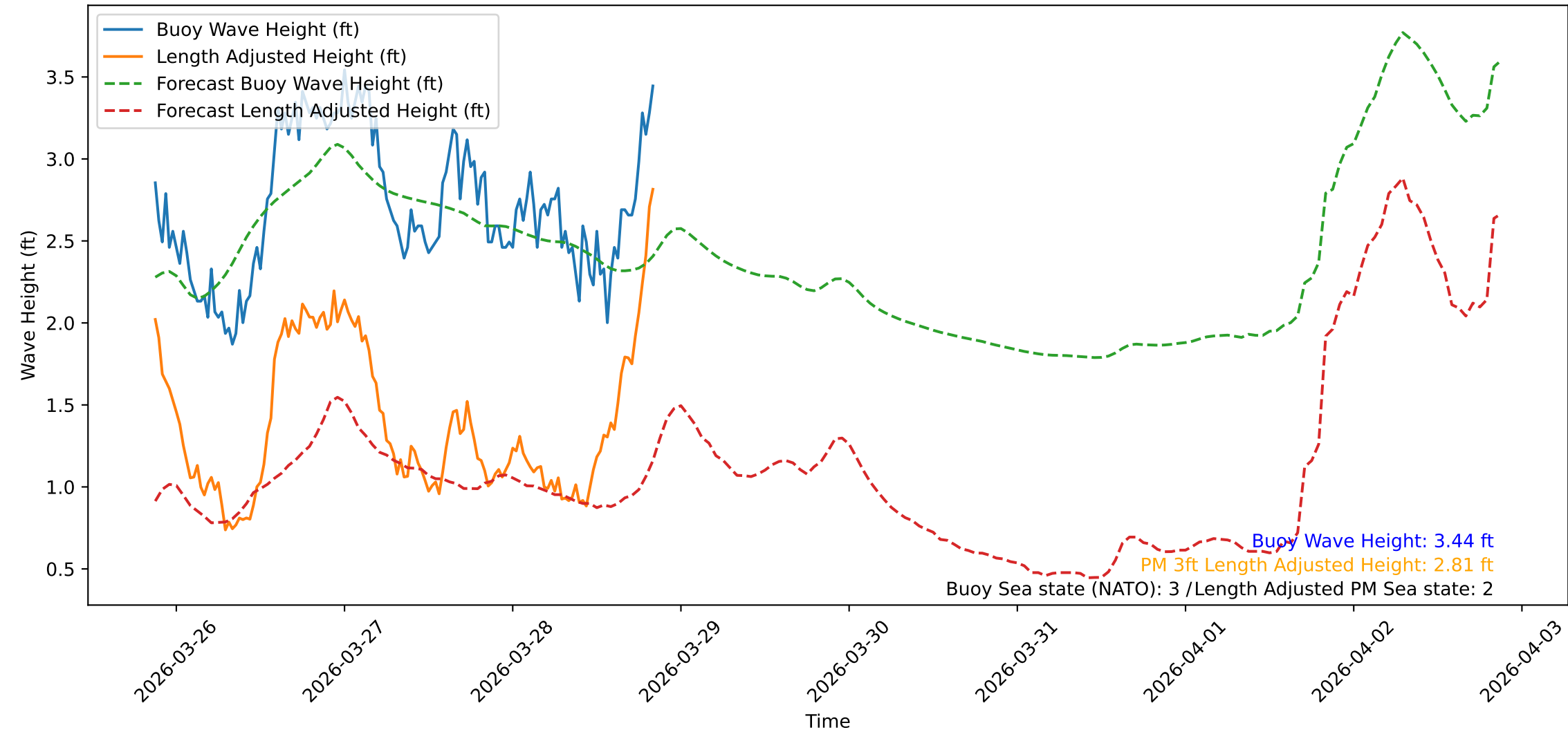
Wave Heights over Time for Green Beach at 2026-03-28 21:01:09
