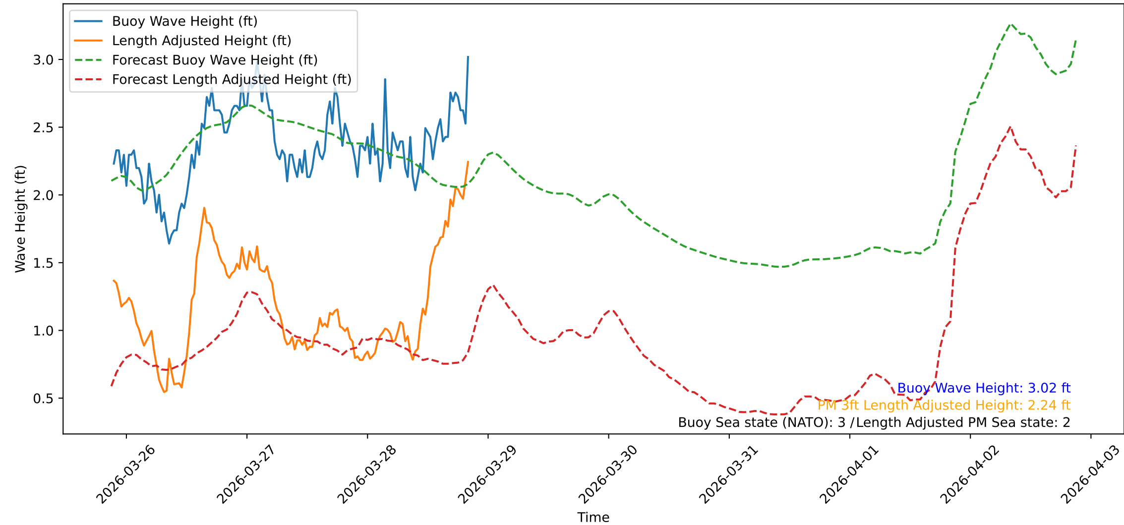
Wave Heights over Time for Red Beach at 2026-03-28 21:00:47
