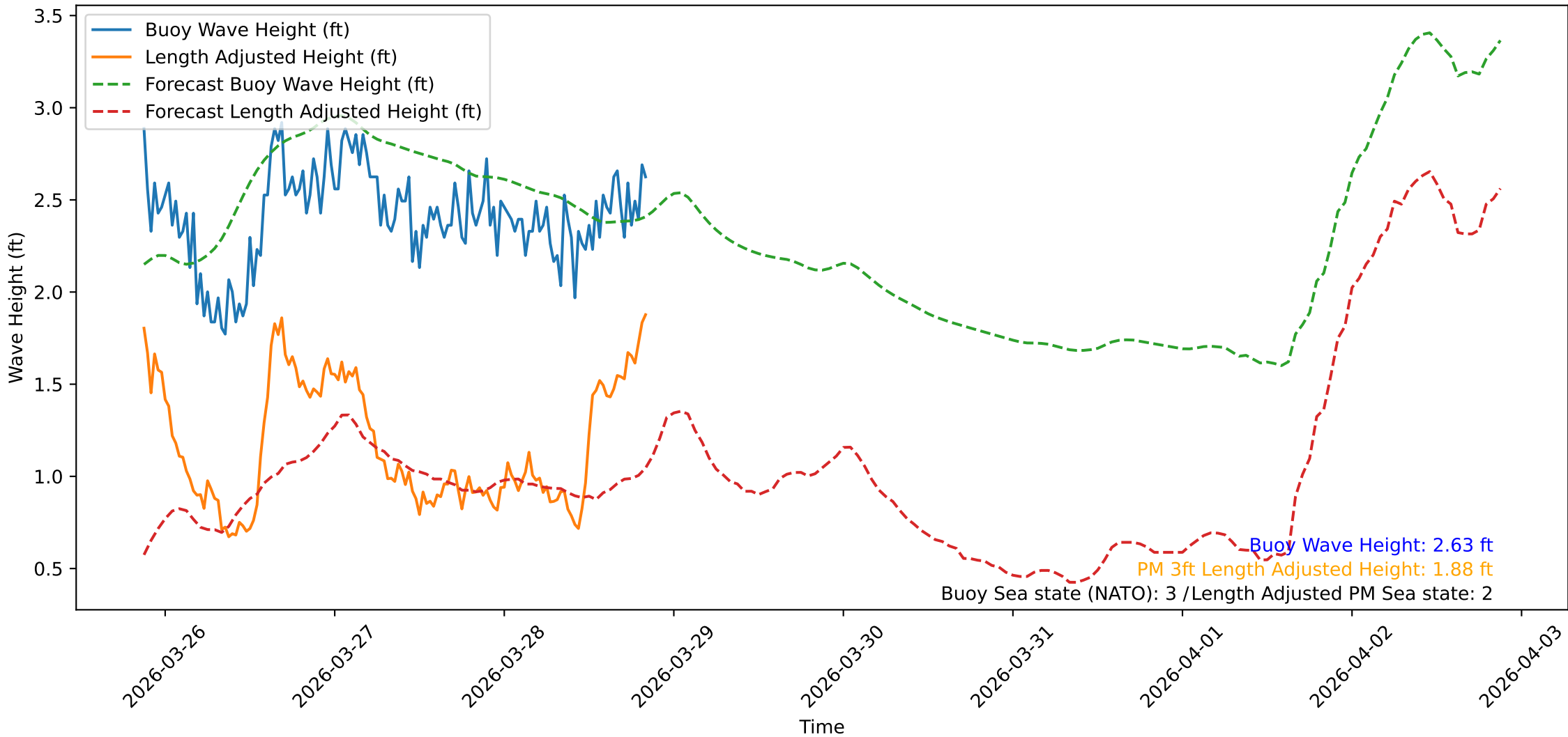
Wave Heights over Time for Oceanside Harbor at 2026-03-28 21:00:31
