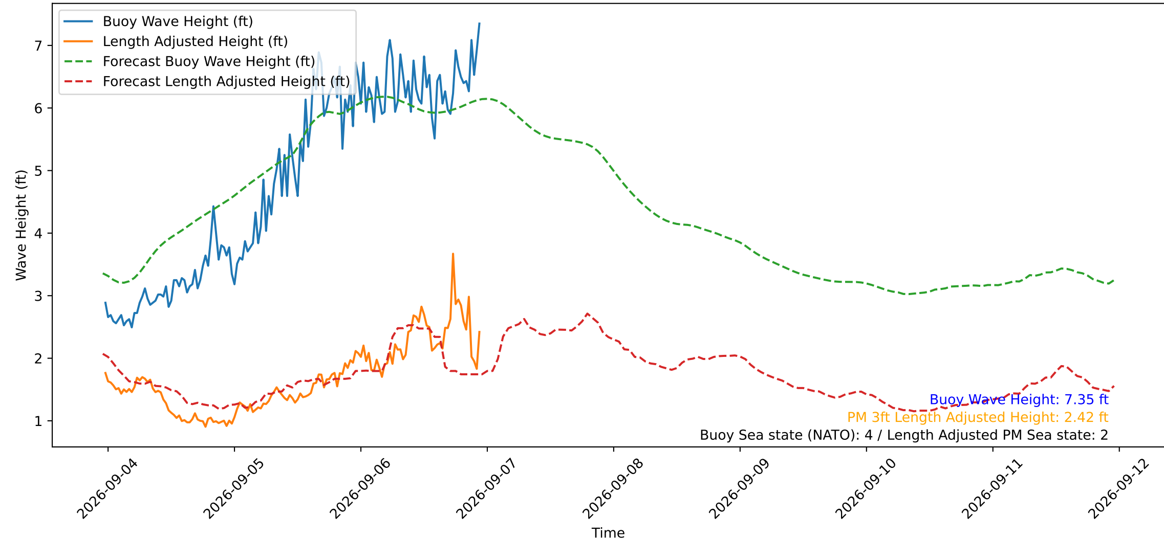
Wave Heights over Time for Green Beach at 2026-09-06 23:21:15
